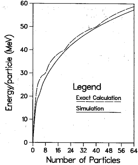
FIG. 3. Ground-state energy per particle calculated for a system of noninteracting neutrons in a harmonic potential with k=4.038 MeV/fm 2 . The dashed curve refers to the exact quantum mechanical calculation, while the solid curve is the result from the simulation.
