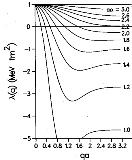
FIG. 1. Eigenvalues of the curvature matrix along q_x = q_y = q_z axis for various values of a\alpha .
