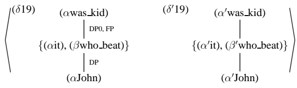
Figure 20: Syntactic and semantic derivation trees for 'It was a kid who beat John'
