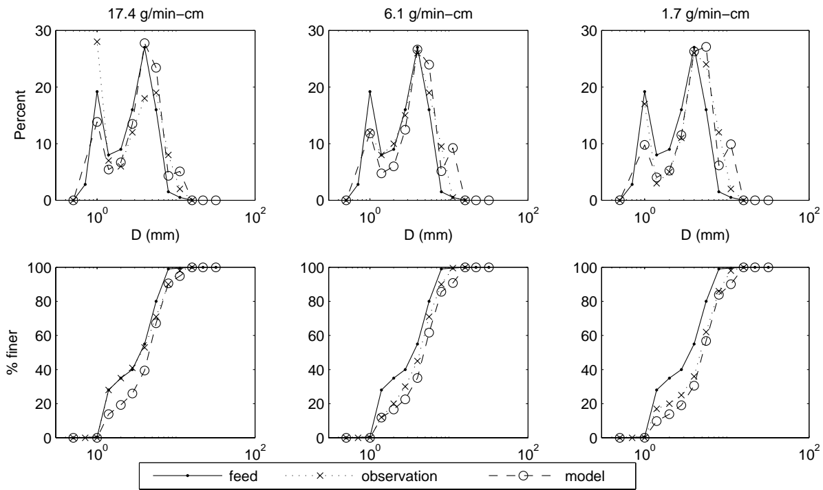
Figure 4. Probability (top) and cumulative (bottom) grain size distributions of the feed, the observed bed surface, and the bed surface predicted by the 1-D model, for the Dietrich et al. (1989) experiments.
