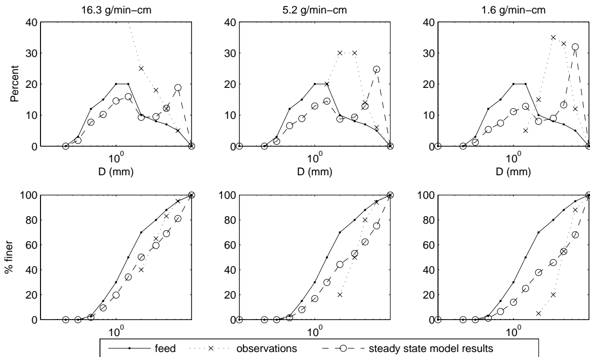
Figure 5. Probability (top) and cumulative (bottom) grain size distributions of the feed, the observed bed surface, and the steady state bed surface predicted by the 1-D model, for the Lisle et al. (1993) experiments.
