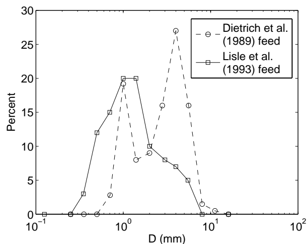
Figure 3. Grain size distributions of the Dietrich et al. (1989) and Lisle et al. (1993) experiments.
