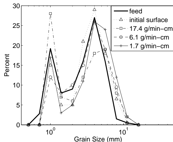
Figure 2. Grain size distributions of the feed and bed surface in the Dietrich et al. (1989) experiments.
