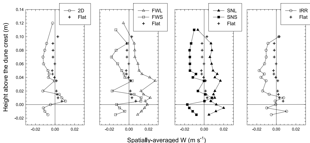
Figure 10. Along-stream spatial averages of centerline mean vertical velocity W . Spatial averages are along lines of constant elevation above the bed form crest.
