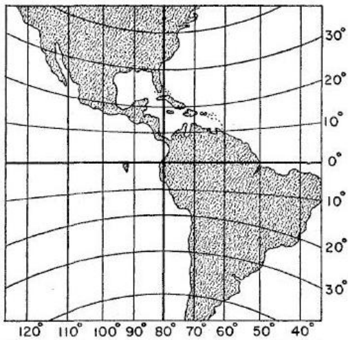
Figure 30. Gnomonic map of the Western Hemisphere
