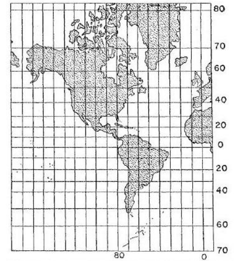
Figure 34. Mercator projection of the Western Hemisphere
