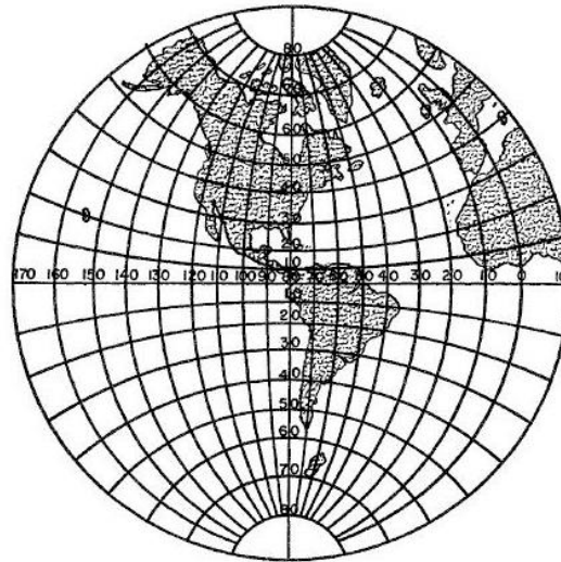
Figure 32. Stereographic map of the Western Hemisphere
