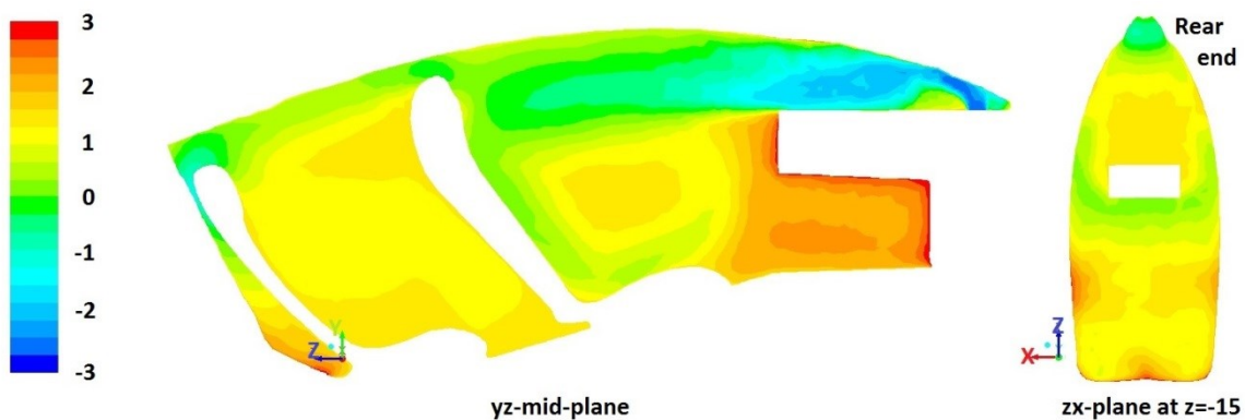
Figure 4.9. PMV contour: Test 1
