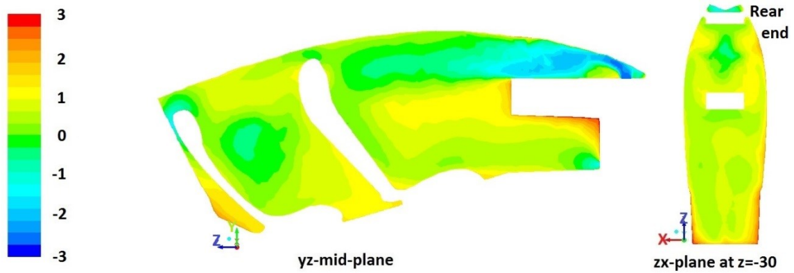
Figure 4.28. PMV contour: Test 20
