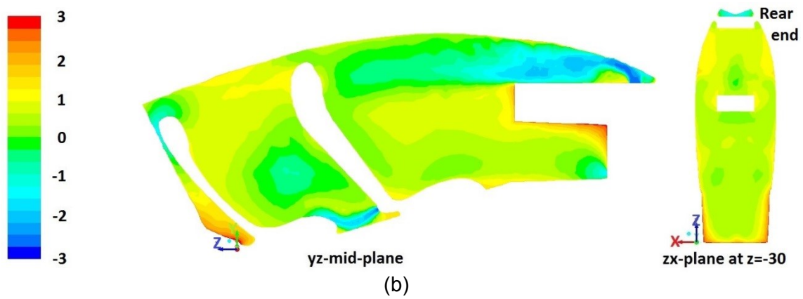
Figure 4.19. PMV contour: (a) Test 11; (b) Test 18
