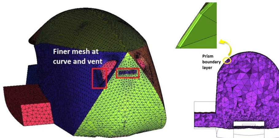
Figure 4.5. Mesh treatment: Finer mesh at curves and vents, and prism layer at boundary
