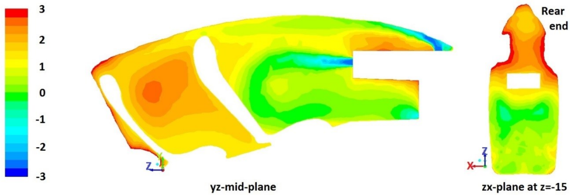
Figure 4.14. PMV contour: Test 6
