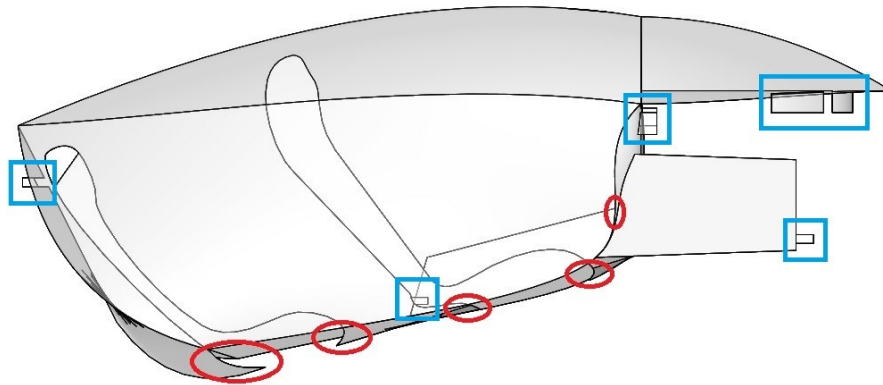
Figure 4.2. The eVaro geometry: The indication of modification-required parts
