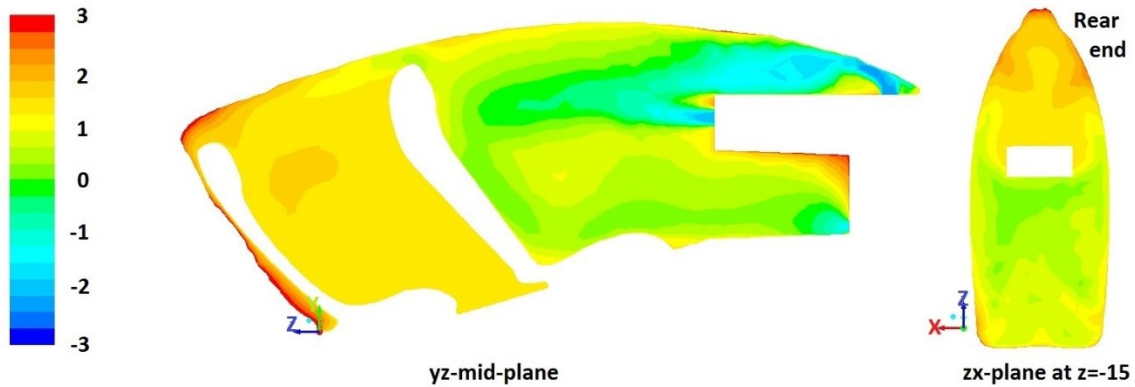
Figure 4.15. PMV contour: Test 7
