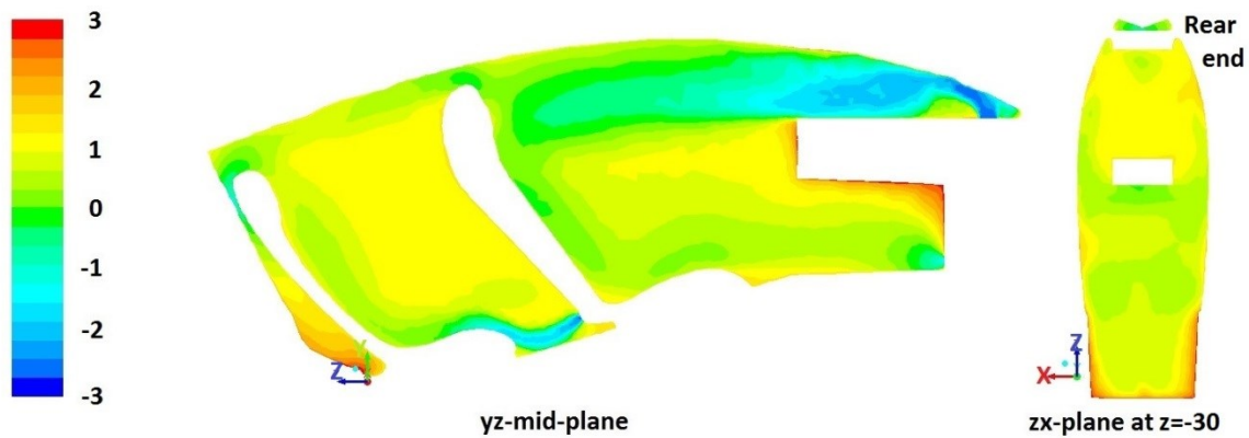
Figure 4.17. PMV contour: Test 9
