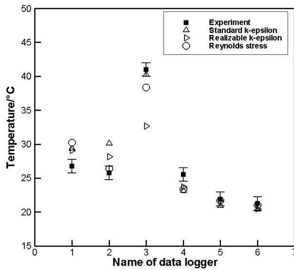
Figure 3.10. Comparison of experiment and numerical simulations for temperature: different turbulence model; Test 4
