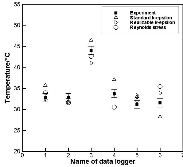
Figure 3.9. Comparison of experiment and numerical simulations for temperature: different turbulence model; Test 3
