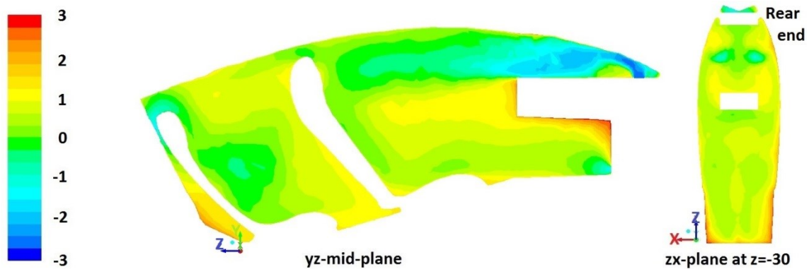
Figure 4.25. PMV contour: Test 17
