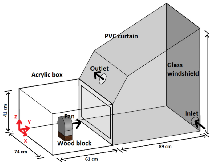
Figure 2.1. The SolidWorks schematic of the experimental testbed
