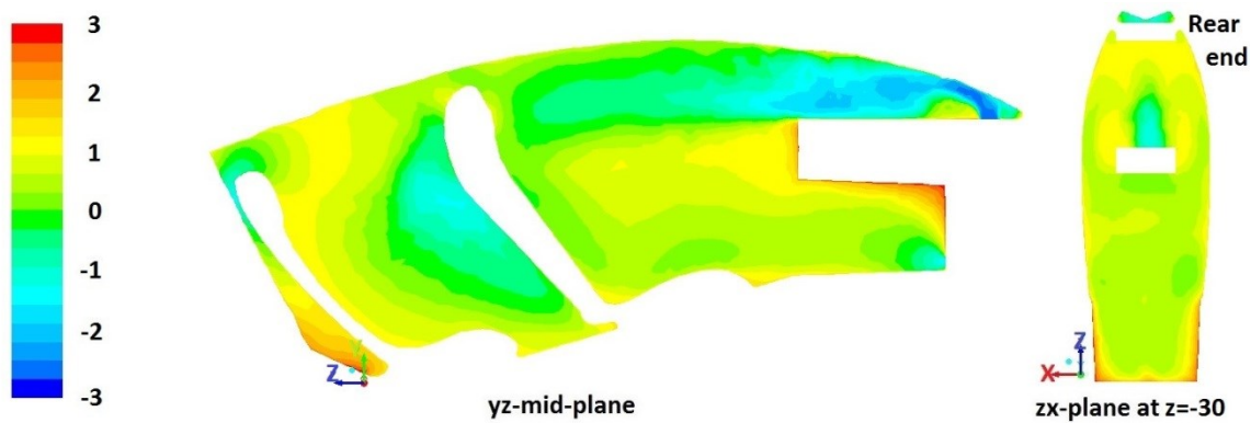
Figure 4.24. PMV contour: Test 16
