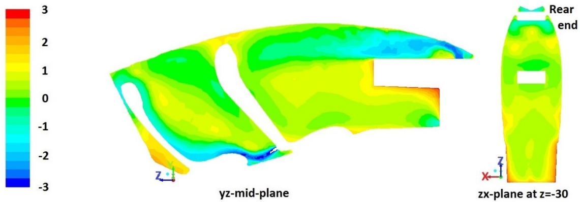
Figure 4.22. PMV contour: Test 14
