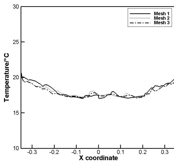
Figure 4.6. Grid dependency check: a line along x-coordinate, from (-0.35, 0, 0.4) to (0.35, 0, 0.4)
