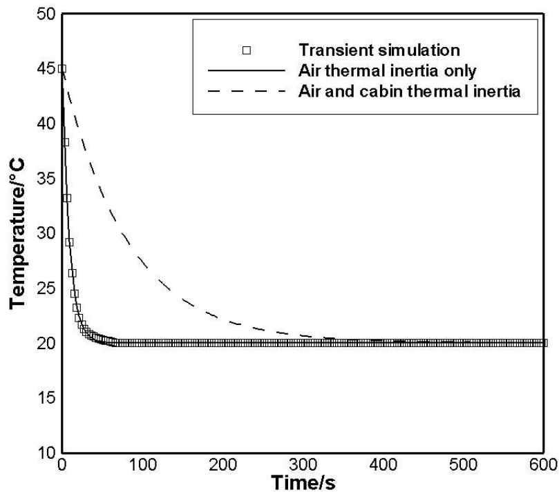
Figure 4.32. Transient simulation results for calculating pull-down time
