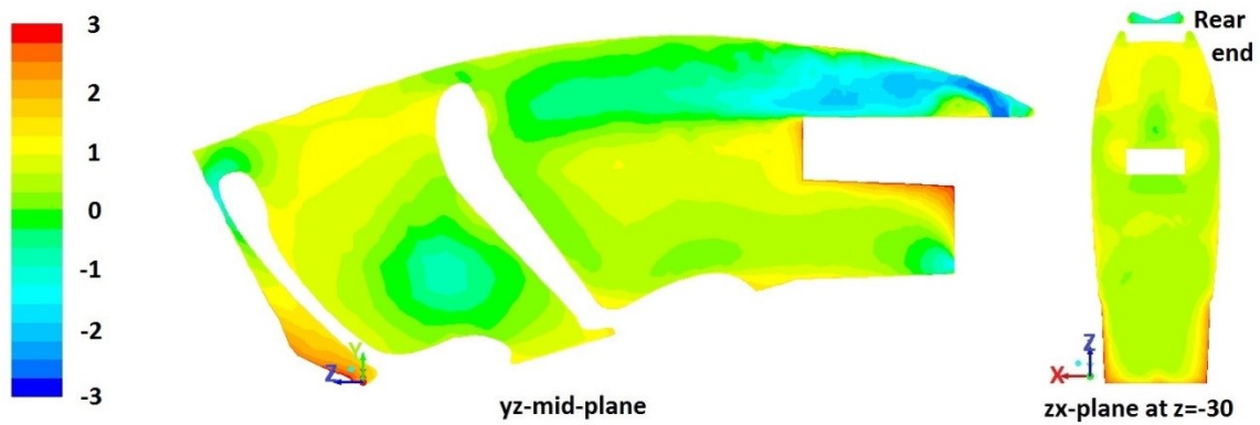
Figure 4.23. PMV contour: Test 15
