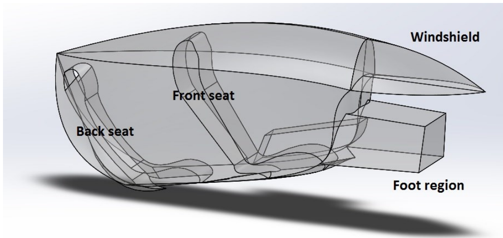
Figure 4.1. The SolidWorks model of the eVaro inner geometry
