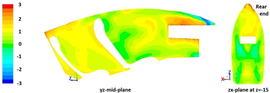
Figure 4.13. PMV contour: Test 5
