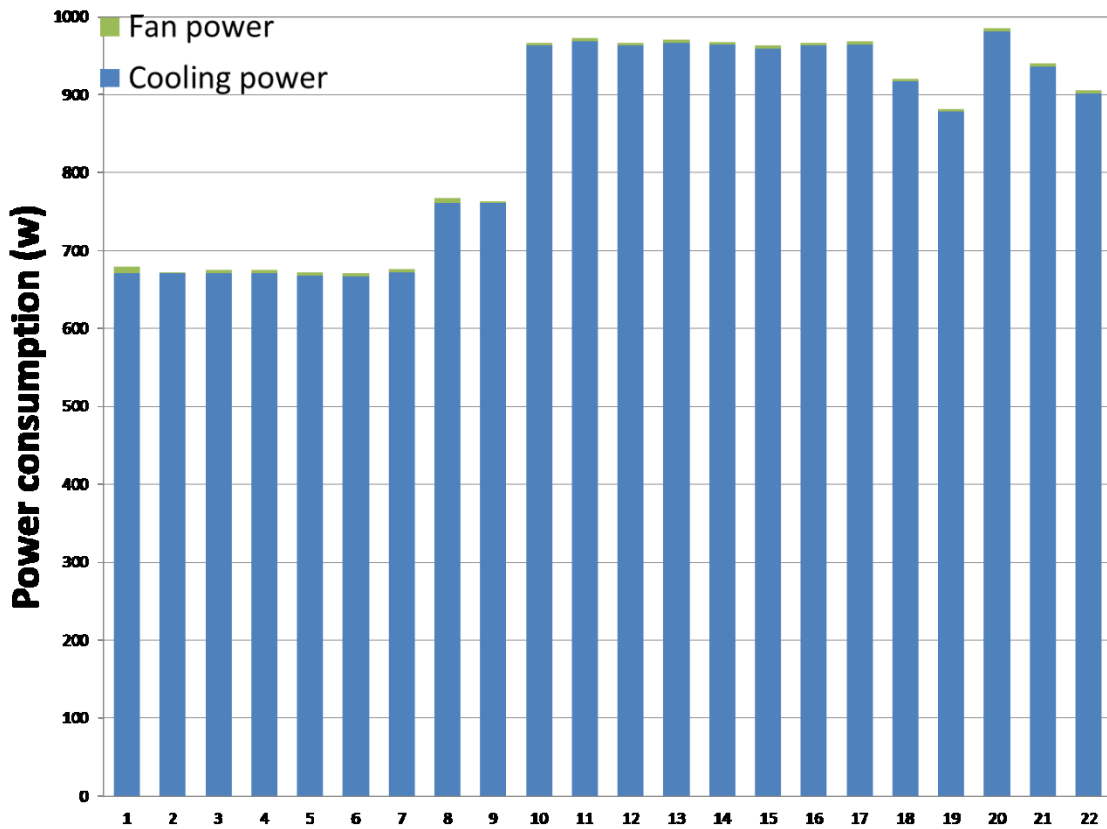
Figure 4.31. Power consumption
