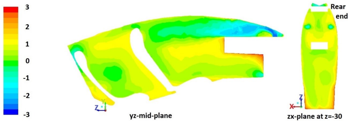
Figure 4.29. PMV contour: Test 21
