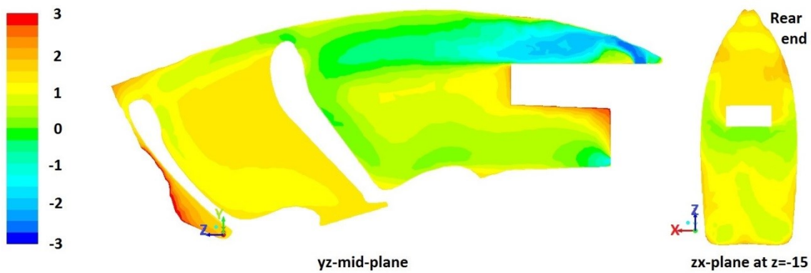
Figure 4.11. PMV contour: Test 3
