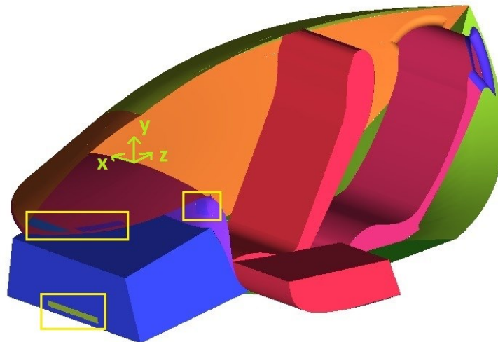
Figure 4.4. The eVaro geometry in ICEM: The vent-extrusions are cleaned up
