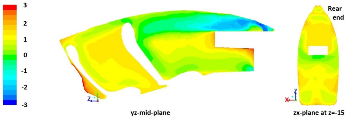
Figure 4.12. PMV contour: Test 4
