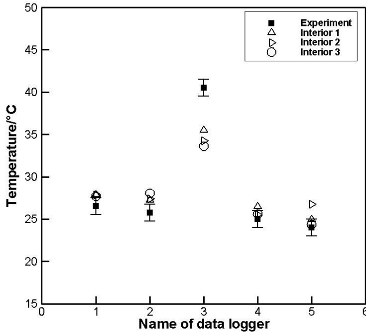
Figure 3.5. Comparison of experiment and numerical simulations for temperature: different interior element size
