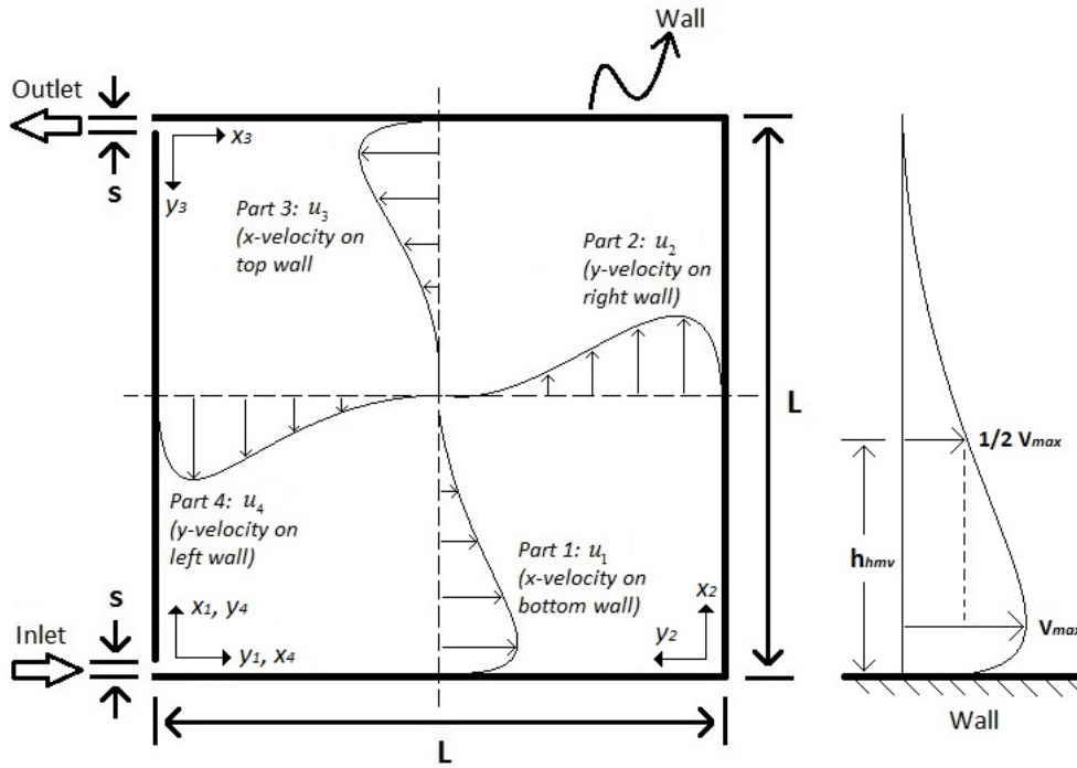
Figure B.5.1. Problem schematic: 2D cavity
