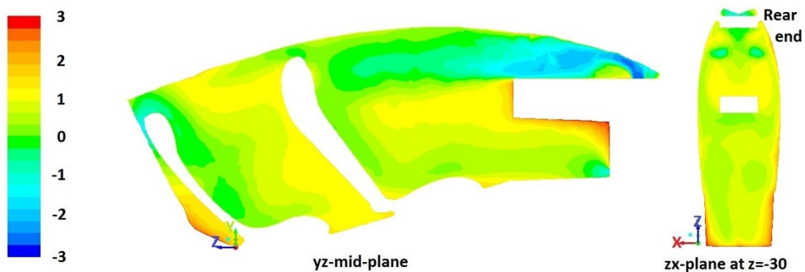
Figure 4.26. PMV contour: Test 18
