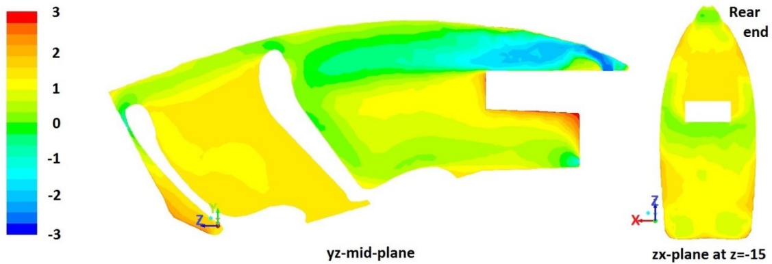
Figure 4.10. PMV contour: Test 2
