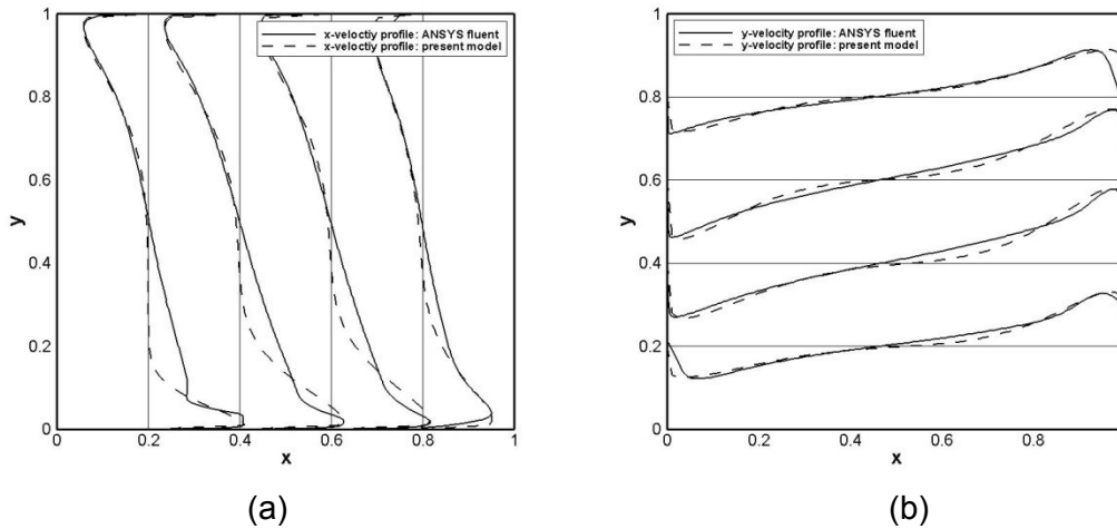
Figure B.5.3. Comparison between the present model and numerical simulations with 0.05 m slit width: (a) x –velocity at vertical cross-sections; (b) y –velocity at horizontal cross-sections
