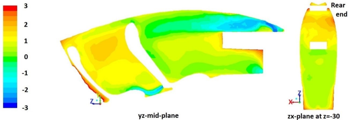
Figure 4.16. PMV contour: Test 8
