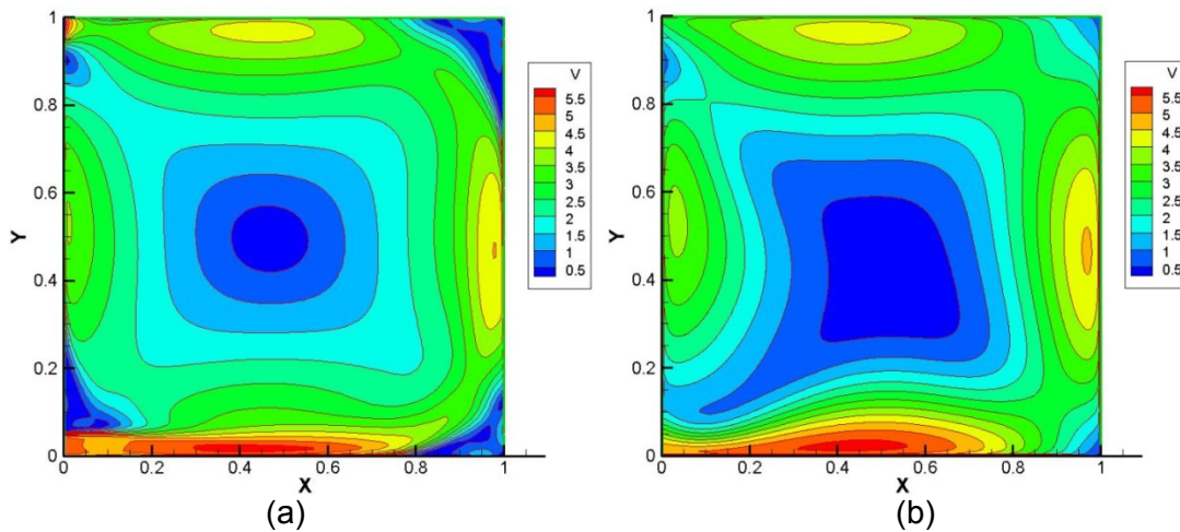
Figure B.5.4. Velocity magnitude contour of the cavity problem: (a) numerical simulation; (b) the present model
