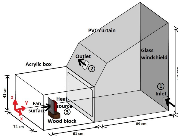
Figure 3.3. The testbed model after modification: 1) Inlet; 2) Outlet; 3) Fan model
