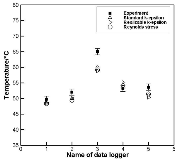
Figure 3.8. Comparison of experiment and numerical simulations for temperature: different turbulence model; Test 2
