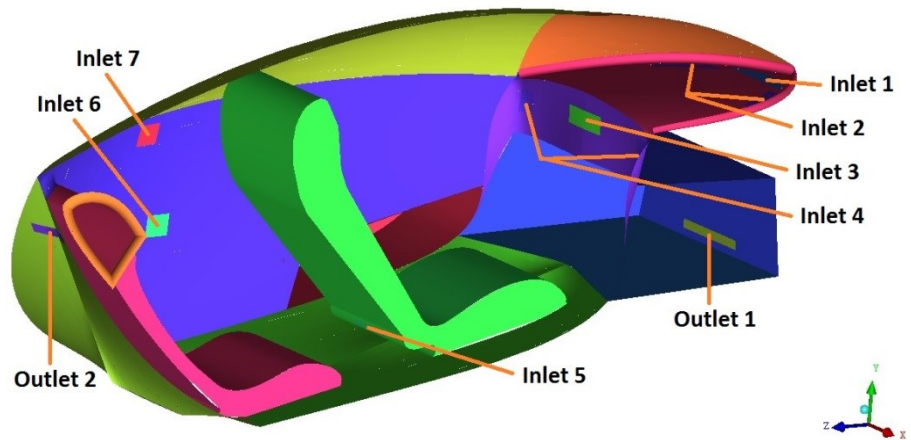
Figure 4.8. The locations of inlets and outlets
