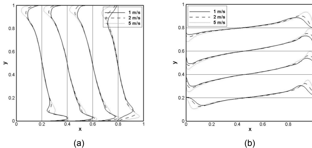
Figure B.5.2. Comparison of velocity at cross-sections: (a) x velocity; (b) y velocity
