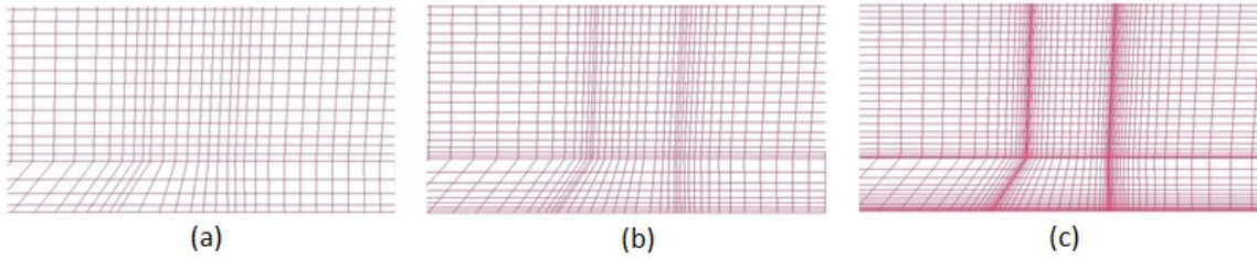
Figure 3.4. Demonstration of 3-level boundary types at near wall region: a cross-section around heater-fan
