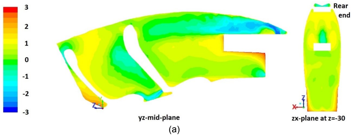
Figure 4.19. PMV contour: (a) Test 11; (b) Test 18
