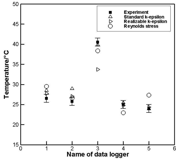
Figure 3.7. Comparison of experiment and numerical simulations for temperature: different turbulence model; Test 1
