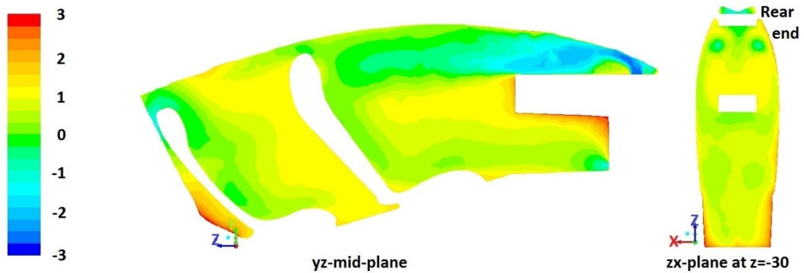
Figure 4.27. PMV contour: Test 19
