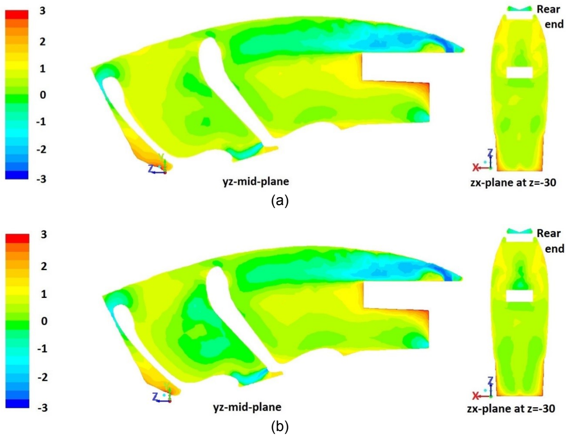
Figure 4.18. PMV contour: (a) Test 10; (b) Test 17
