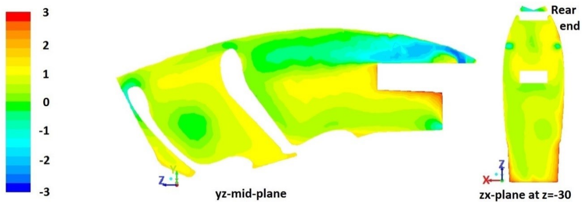
Figure 4.30. PMV contour: Test 22
