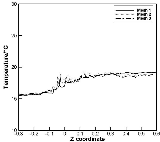
Figure 4.7. Grid dependency check: a line along z-coordinate, from (0, 0.1, -0.3) to (0, 0.1, 0.6)
