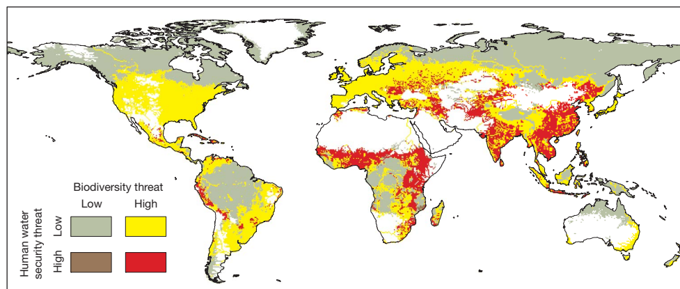
Figure 6 | Prevailing patterns of threat to human water security and biodiversity. Adjusted human water security threat is contrasted against incident biodiversity threat. Much of the developed world faces the challenge of reducing biodiversity threat and protecting biodiversity, while maintaining established water services. The developing world shows tandem threats to human water security and biodiversity, posing an arguably more significant
