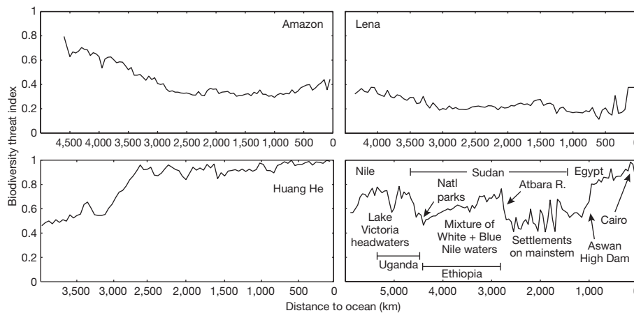
Figure 2 | Incident biodiversity threat transects from headwaters to ocean. Distinctive patterns characterize each river system resulting from complex spatial patterns of stressor loadings across the catchment plus mixing of higher and lower concentration tributary waters through river networks. Transects represent the collective impact of stressors operating within particular
