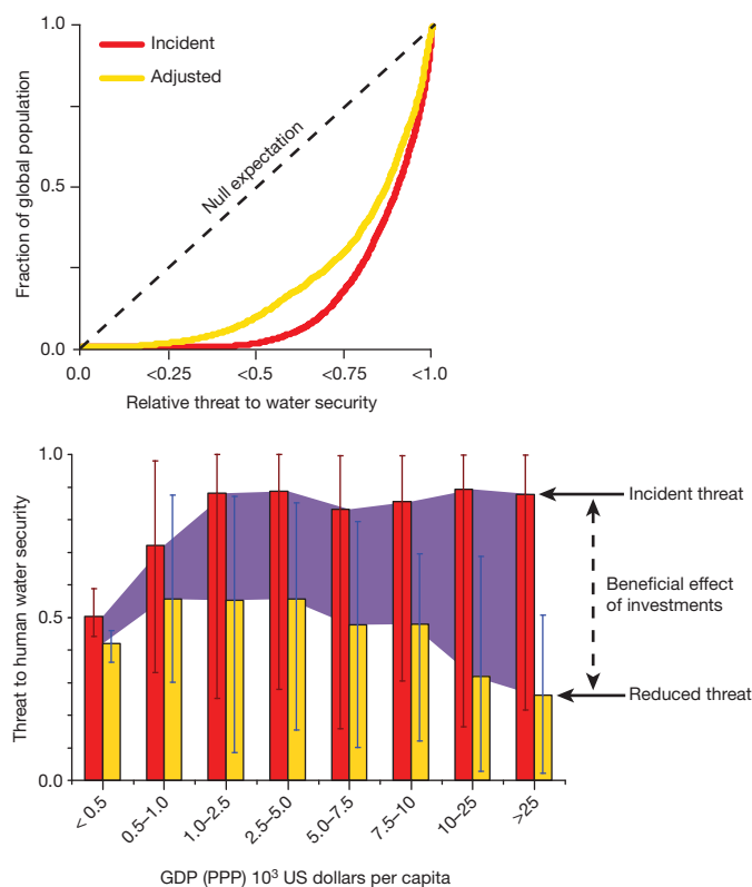
Figure 5 | Globally aggregated human water security threat indices linked to population and level of economic development. Investments in engineering infrastructure and services improve water security, with their value expressed here in reduced threat units. Net benefits accrue to only a fraction of global population (top). Technology investments greatly benefit wealthy nations, shifting them from most to least threatened (bottom). The fraction of global population is over the discharging landmass. GDP (PPP) refers to annual gross domestic product in 2008 at purchasing power parity exchange 50 , with associated grid-cell means of incident human water security threat (red bars) and reduced threat (yellow; see Fig. 4). Vertical lines represent ranges.
