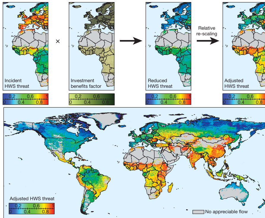
Figure 4 | Shifts in spatial patterns of relative human water security threat after accounting for water technology benefits. Inset maps illustrate the analytical approach and net impact of investment over a north–south transect (top). Incident human water security (HWS) threat is converted to reduced threat (inset maps), which is then globally re-scaled into adjusted human water
