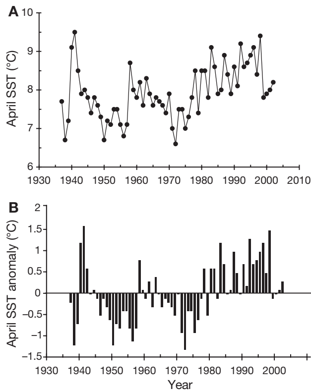
Fig. 2. (A) Mean spring (April) SST at Pine Island, British Columbia, 1937–2002 and (B) SST anomalies over same period
