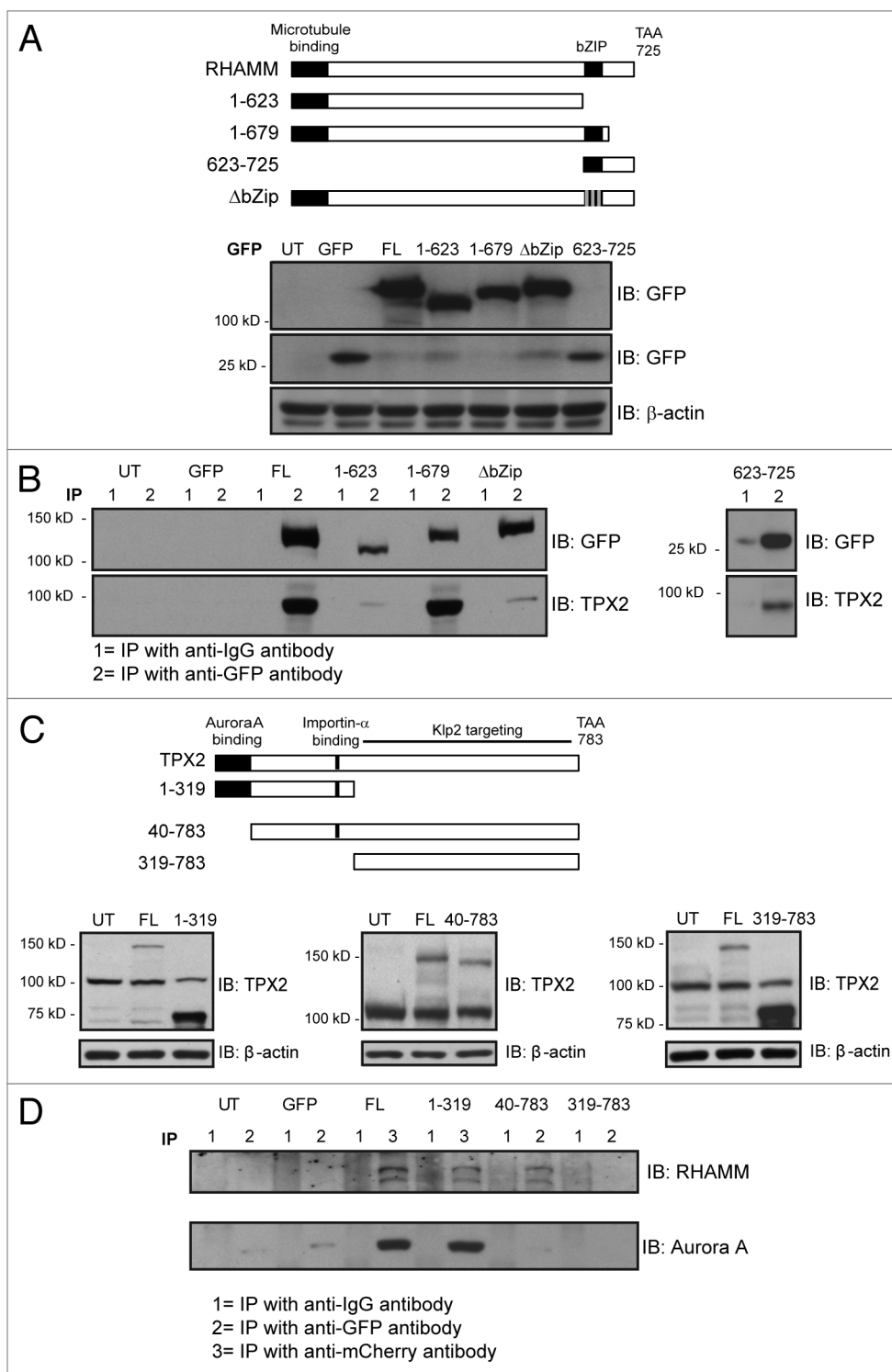
Figure 4. Characterization of the functional domains involved in RHAMM-TPX2 interaction during early mitosis. (A) Schematic diagram of defined domains in RHAMM. The 3 gray lines in the ΔbZIP construct represent leucines mutated to arginines. Western blot analysis confirmed the expression of GFP-RHAMM constructs. β-actin levels confirmed equal loading. (B) Immunoprecipitation of GFP-RHAMM constructs identified the bZIP motif as a necessary domain in RHAMM for the co-precipitation of TPX2. Cell lysates were immunoprecipitated with either an IgG control antibody (lanes marked 1) or antibodies against eGFP (lanes marked 2). (C) Schematic diagram of defined domains in TPX2. Western blot analysis confirmed the expression of mCherry-TPX2 and TPX2-GFP truncation variants. β-actin levels confirmed equal loading. (D) Immunoprecipitation of mCherry-TPX2 or TPX2-GFP truncation variants identified amino acids 40–319 as necessary for the co-precipitation of RHAMM. Cell lysates were immunoprecipitated with either an IgG control antibody (lane marked 1) or antibodies against eGFP (lane marked 2) or mCherry (lane marked 3).
