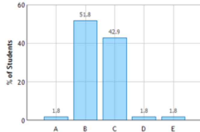
Rolling down a ramp: Question 1 (N = 56)
