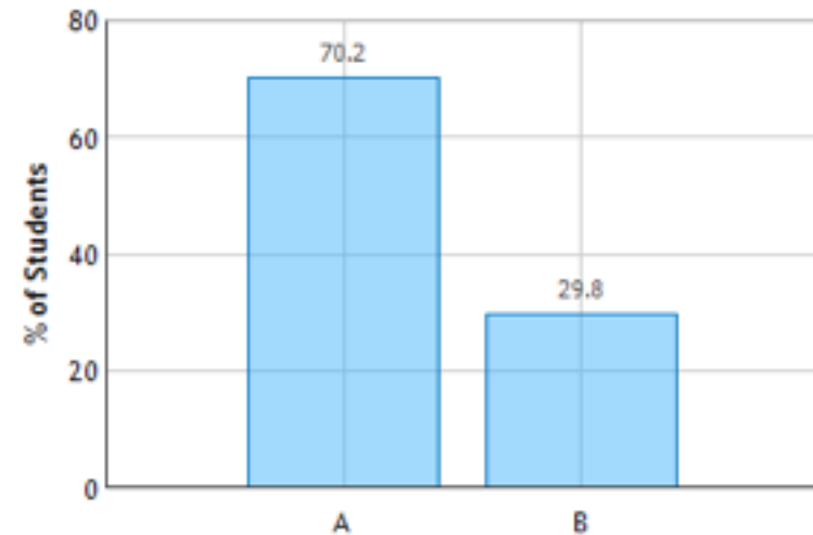
x(t) , v(t) , a(t) plots: Question 1 (N = 57)
