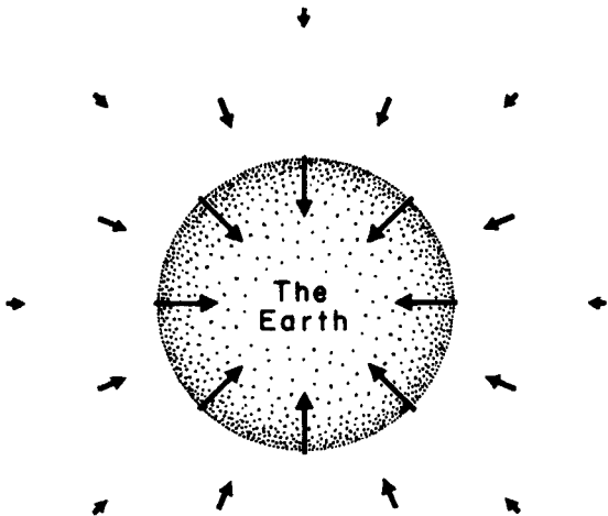
Figure 1.1 The gravitational field of the Earth. The arrows represent the direction and strength of the gravitational field.
