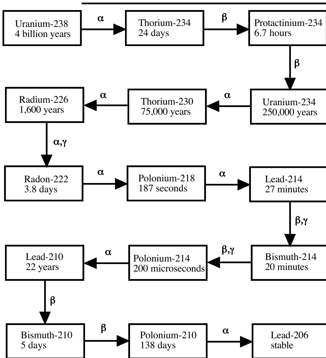
Figure 28-9: The Uranium-238 decay series shown above is one of several natural decay series which start with heavy isotopes of thorium or uranium.
