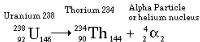
Figure 28-7: Symbols to display the neutrons and protons when the uranium 238 nucleus gives off an alpha particle.
