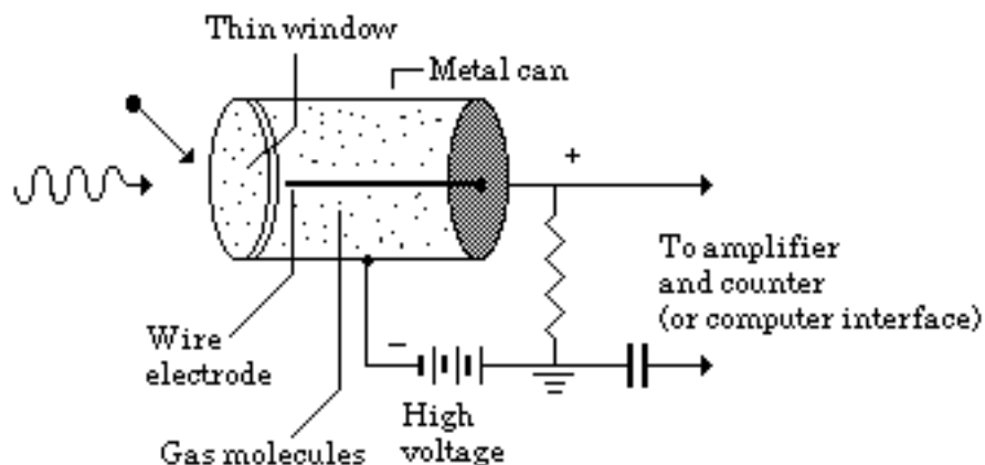
Figure 28-6: A schematic for the Geiger tube, which detects beta particles and gamma rays. The RM-4 Monitor has a Geiger tube and amplifier circuit in it.
