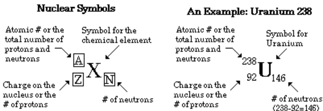
Figure 28-6: Symbols to display the neutrons and protons in nuclear isotopes in general and for the uranium 238 in particular.
