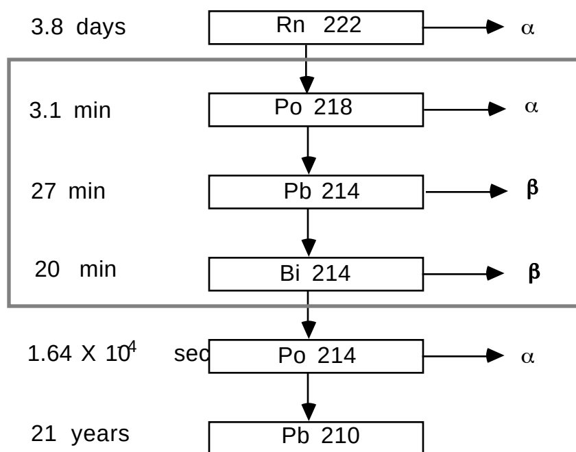
Figure 28-10: The portion of the uranium 238 decay series of interest in radon monitoring
