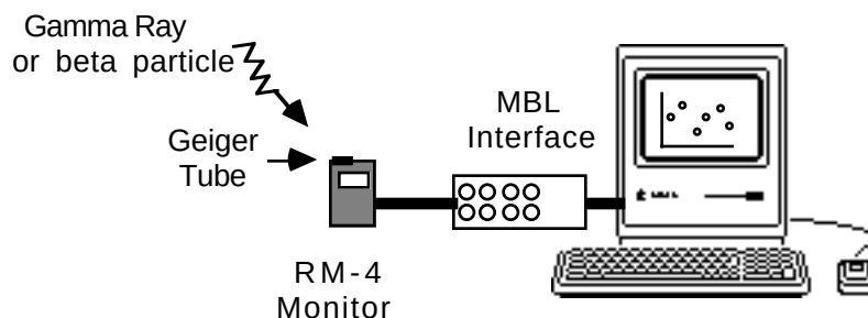
Figure 28-2: An MBL Radiation Counting System
