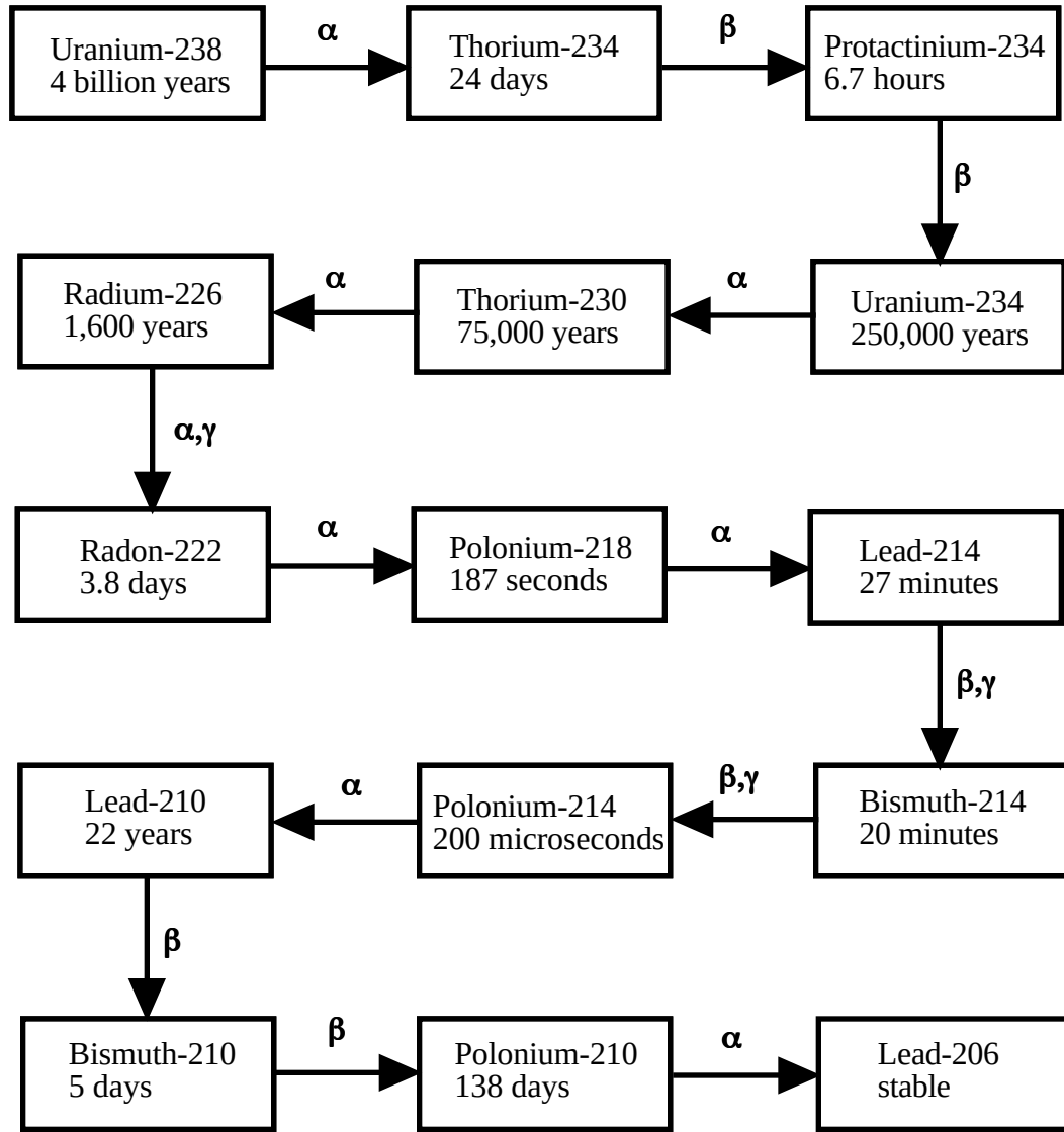
Figure 28-9: The Uranium-238 decay series shown above is one of several natural decay series which start with heavy isotopes of thorium or uranium.
