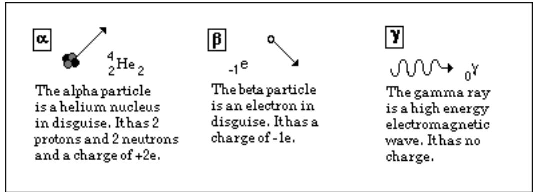
Figure 28-5: The most common types of radiation emitted by radioactive nuclei.
