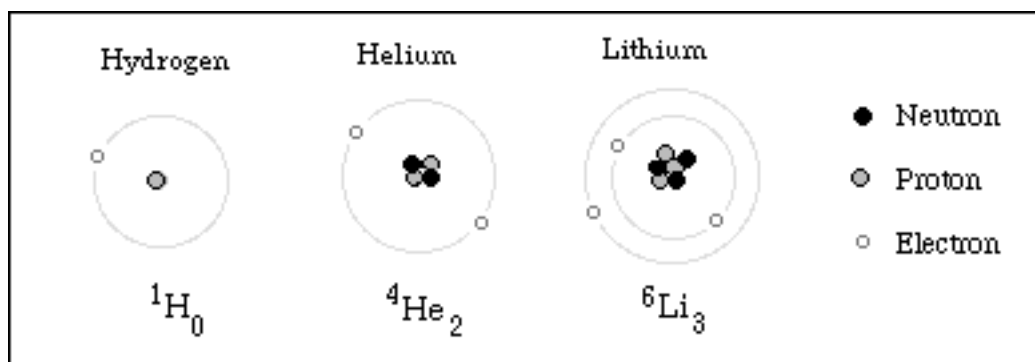
Figure 28-3: The three lightest chemical elements showing the number of protons that define the element along with the most common number of neutrons in the nucleus. The gray circle represents a proton, the black circle a neutron, and the white circle an electron. The diagram is simplified as electrons are not pictured by physicists as orbiting the nucleus of an atom in nice, neat circles.
