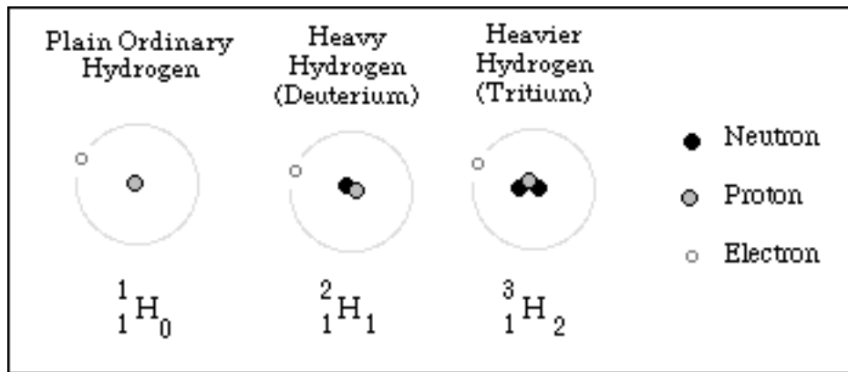
Figure 28-4: Three isotopes of hydrogen. Deuterium is of great interest as a fuel for the nuclear fusion process, which may allow mankind to have an abundant source of low-cost energy.
