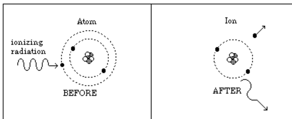
Figure 28-1: Schematic of ionizing radiation in the form of a gamma ray which knocks an electron out of an atom, leaving the atom ionized.
