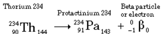
Figure 28-8: Symbols to display the neutrons and protons when the thorium 234 nucleus gives off an beta particle.
