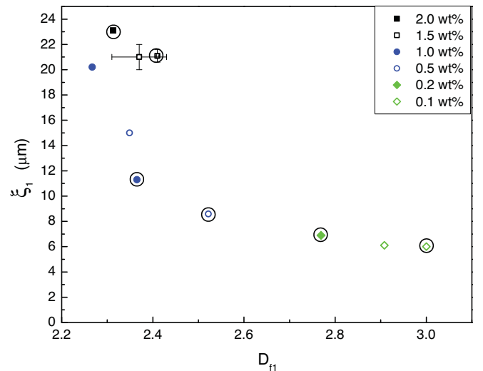
FIG. 9. (Color online) Correlation between the longer length scale \xi_1 and the corresponding fractal dimension D_{f1} . As the particles swell, the fractal dimension decreases from 3 to 2.3. The encircled markers represent data from pH -unmodified Carbopol samples.
