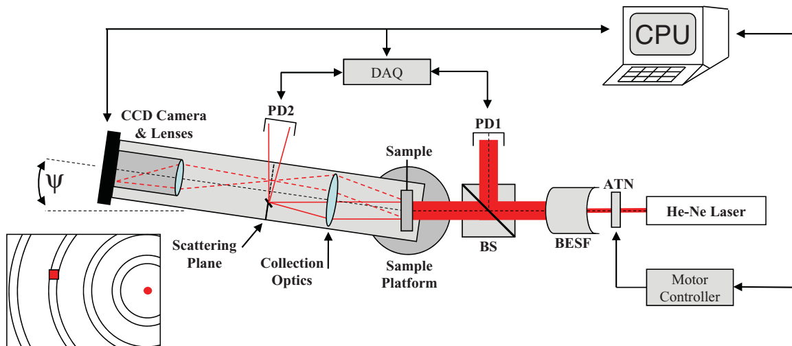
FIG. 1. (Color online) Schematic of the small-angle light scattering instrument setup used in these experiments. Components are described in the text. The lower left shows the field of view seen by the camera. The solid circle represents the optical center and the solid square represents the size of a CCD pixel relative to one of the concentric rings of constant scattering angle \theta . ATN: Attenuator, PD: Photodiode, BS: Beam splitter, BESF: Beam expander and spatial filter.
