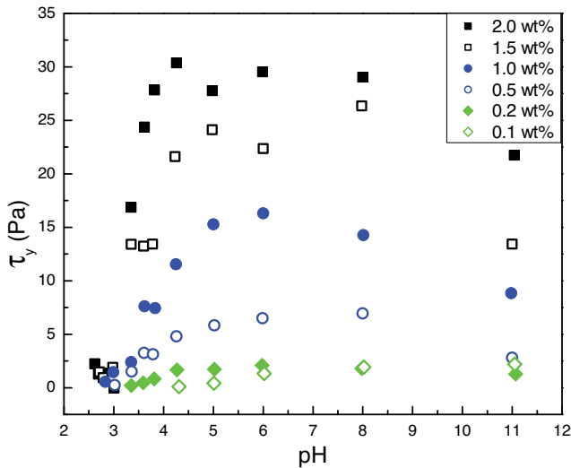
FIG. 3. (Color online) Yield stress as a function of pH for Carbopol concentrations ranging from c = 0.1 wt% to c = 2.0 wt%. The different symbols indicate different concentrations.
