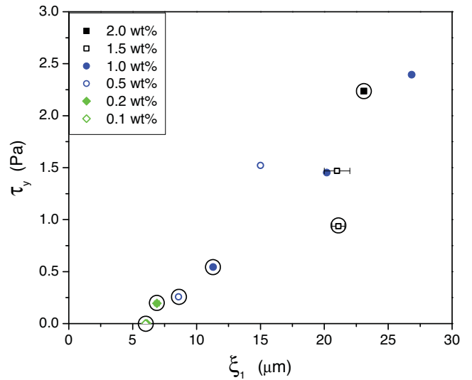
FIG. 10. (Color online) \tau_y plotted as a function of \xi_1 for samples with low yield stress. The yield stress \tau_y increases dramatically as the particles swell. Encircled data points identify pH -unmodified samples.
