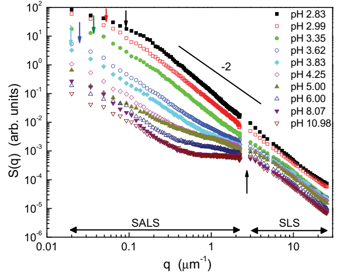
FIG. 4. (Color online) Relative intensity of the scattered light S(q) as a function of scattering wave vector q for 1 wt% Carbopol ETD 2050 and a range of pH values. The arrows identify the locations of the two main scattering features as discussed in the text.
