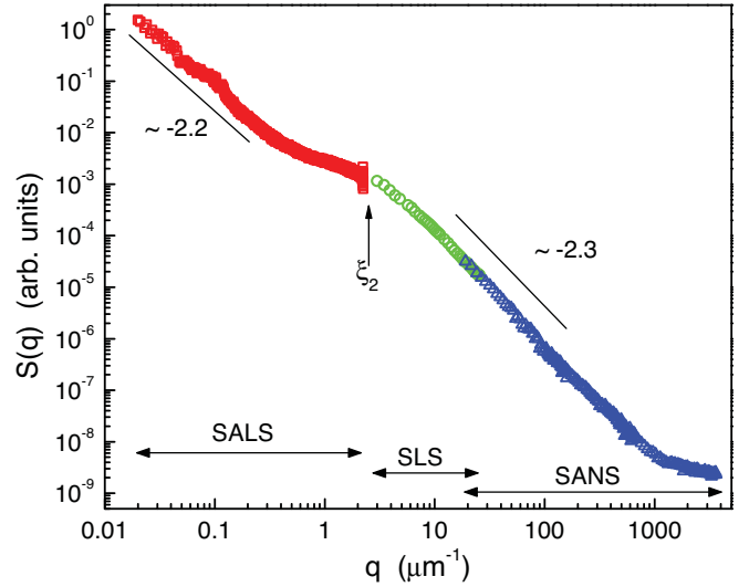
FIG. 8. (Color online) Small-angle neutron scattering and light scattering data for Carbopol with c = 1.5 \text{ wt\%} Carbopol sample adjusted to pH = 6.0 .
