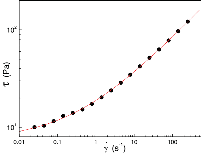
FIG. 2. (Color online) Shear stress as a function of shear rate measured for c = 1.0 wt% Carbopol sample at pH 3.83. The curve is a fit to the Herschel-Bulkley model, Eq. (3), with \tau_y = 7.4 \pm 0.2 Pa, K = 11.4 \pm 0.2 Pa s^n , and n = 0.416 \pm 0.003 .
