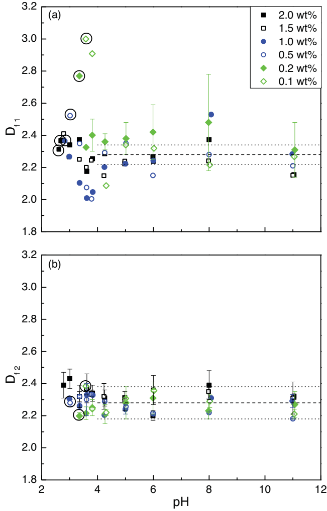
FIG. 7. (Color online) The pH dependence of the fractal dimensions (a) D_{f1} and (b) D_{f2} for samples of different Carbopol concentration. The encircled markers represent data from pH -unmodified Carbopol samples. The dashed and dotted horizontal lines represents the weighted mean and standard deviation of the data for samples with pH \geq 4 .
