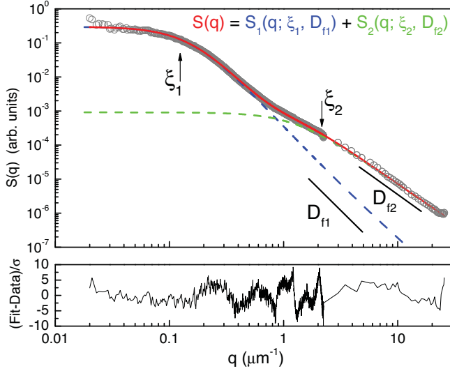
FIG. 5. (Color online) Fit of Eq. (4) to the light scattering data for 0.1 wt% Carbopol at pH = 3.81 . The data are shown as open circles, and the three curves show S_1(q) , S_2(q) , and their sum S(q) . The residuals, in units of the data uncertainty, are shown in the lower portion of the figure.
