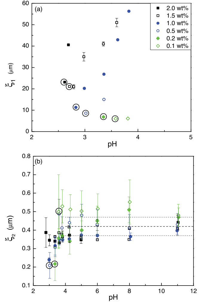
FIG. 6. (Color online) The characteristic length scales (a) \xi_1 and (b) \xi_2 plotted as a function of pH for a range of Carbopol concentrations. The encircled markers represent data from pH -unmodified Carbopol samples. The horizontal lines in (b) represents the weighted mean and standard deviation of the data for pH \geq 4 . Error bars smaller than the data markers are not shown.
