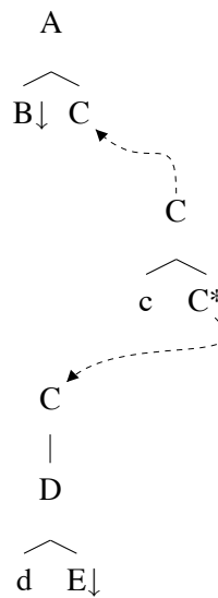
Figure 3.3: Adjoining
