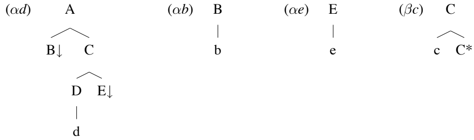
Figure 3.1: Elementary Trees
