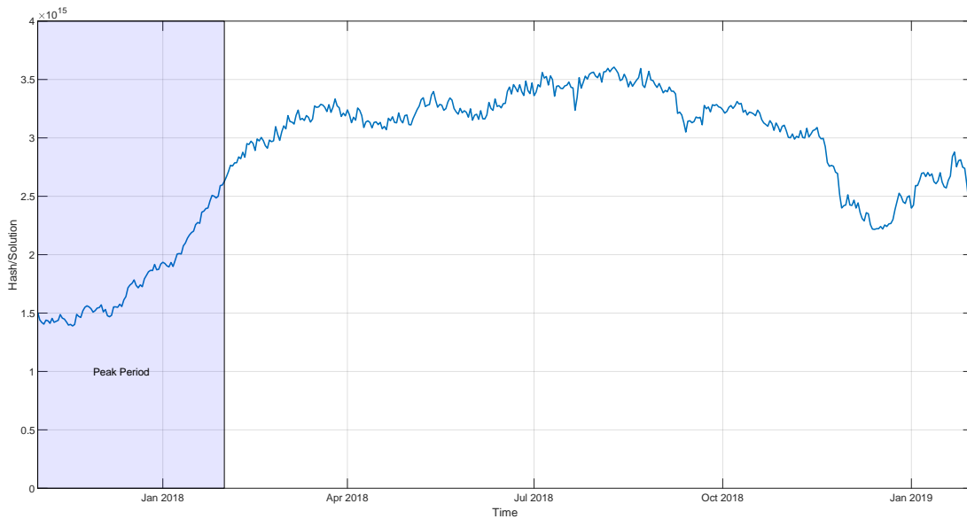
Figure 7: Cryptographic difficulty
