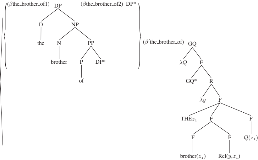
Fig. 28 Multi-component set of elementary trees for the brother of
