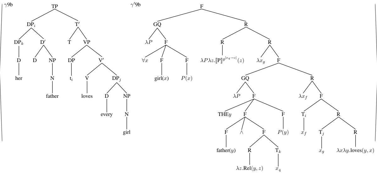
Figure 14: Derived trees for *Her i father loves every girl i .
