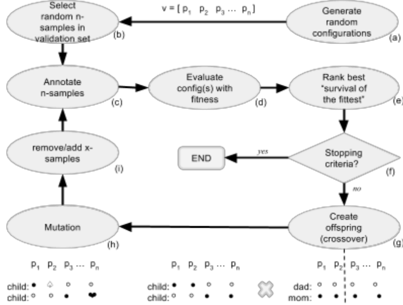
Figure 1. The Genetic Algorithm applied in the Parameter Tuning Architecture (PTA)
