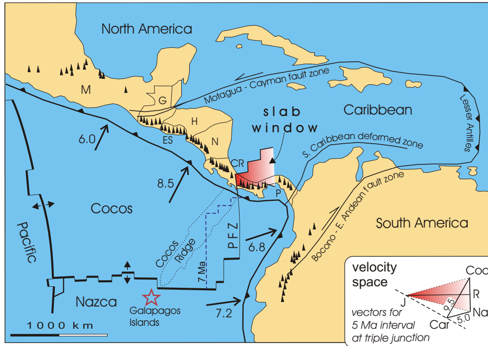
Figures 1-3 from S.T. Johnston and D.J. Thorkelson, 1997, Cocos-Nazca slab window beneath Central America. EPSL 146: 465-474.
