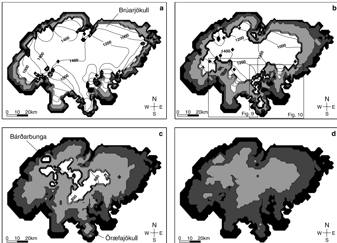
Figure 8. Simulated areal extent of Vatnajökull for the reference model (black) and after 100 (shaded), 150 (lightly shaded), and 200 (white) years of warming with no change in precipitation. Labeled surface contours in Figures 8a–8c indicate the simulated ice surface elevation after 200 years. Per century warming rates are as follows: (a) 1°C; (b) 2°C; (c) 3°C; and (d) 4°C.
