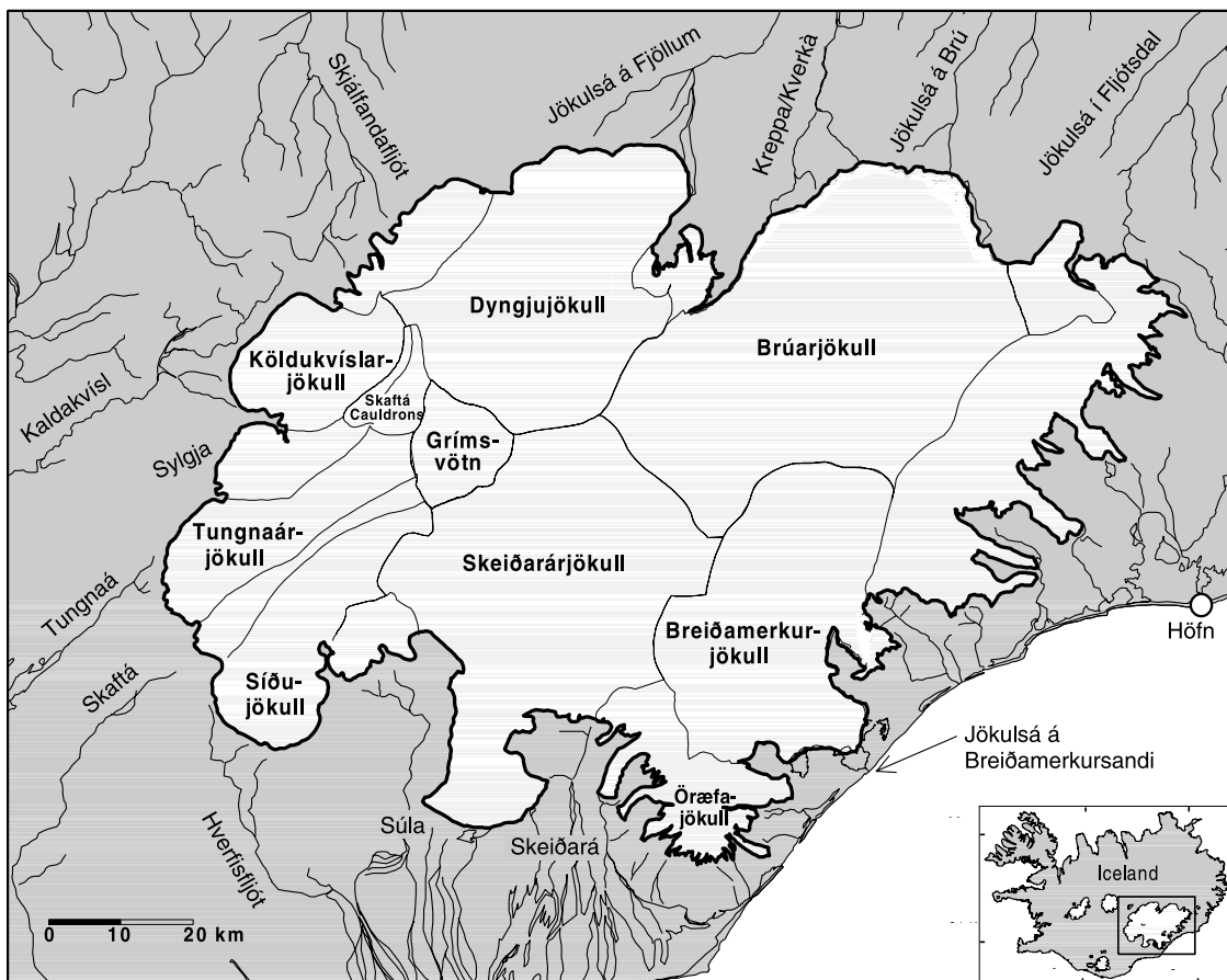
Figure 1. Location map of Vatnajökull and its major outlet rivers. Individual outlet glaciers are delineated by their ice divides.
