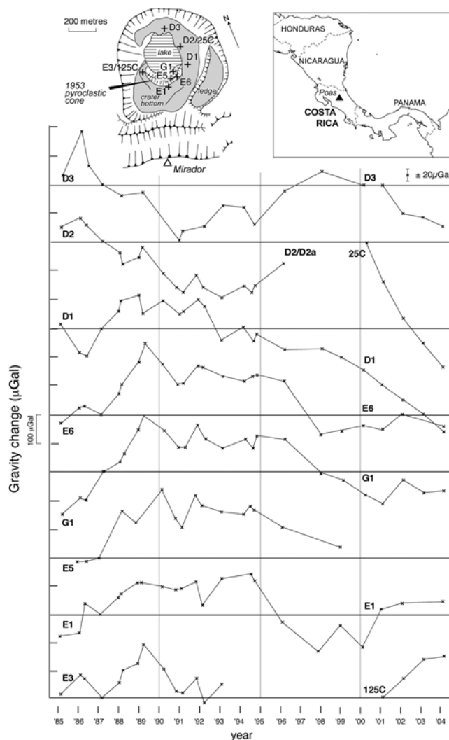
Figure 1. Gravity changes relative to a base station 7 km from the crater are normalised to the difference observed in 1987. Stations in very close proximity (E3 & 125C and D2, D2A & 25C) are not distinguished in the figure. First inset: Station location map within the active crater area of Poás volcano. Second inset: Map showing location of Poás Volcano.
