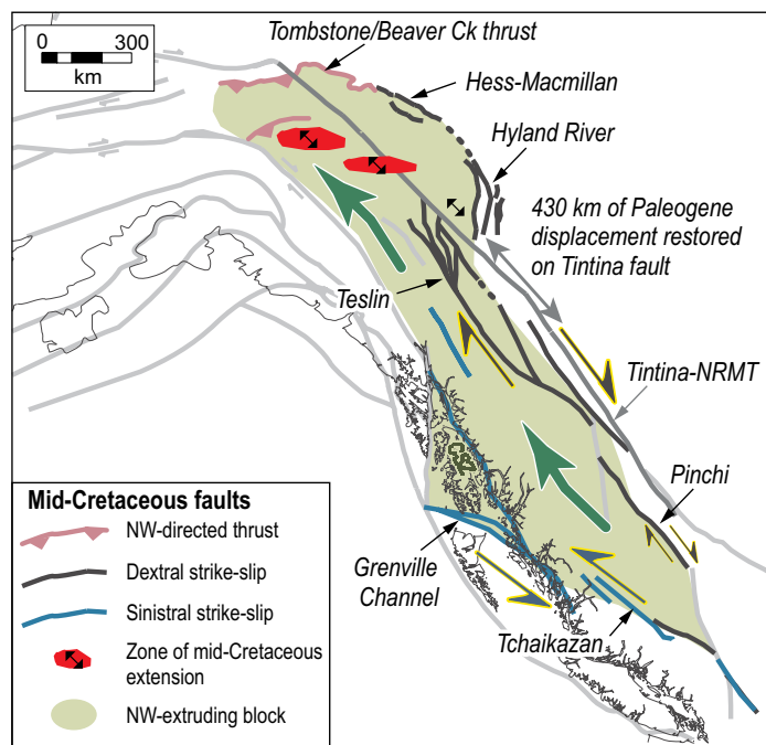
Figure 9. Mid-Cretaceous extensional zones (in red) in east-central Alaska and Yukon (Finlayson and Australia Mountain domains) are located near the leading edge of a northwestward-extruding block (in green). The block is bounded to the southwest by series of sinistral strike-slip faults (Grenville Channel and Tchaikazan), whereas roughly coeval dextral strike-slip faults mark the northeastern edge (Hyland River, Hess-Macmillan) and feed into the NW-directed Tombstone and Beaver Creek thrusts, which define the leading edge of this extruding block. Approximately 430 km of displacement, and offset of Yukon-Tanana terrane, has been restored along the Paleogene Tintina fault (in grey) (modified from Nelson et al., 2013). NMRT—Northern Rocky Mountain Trench.
