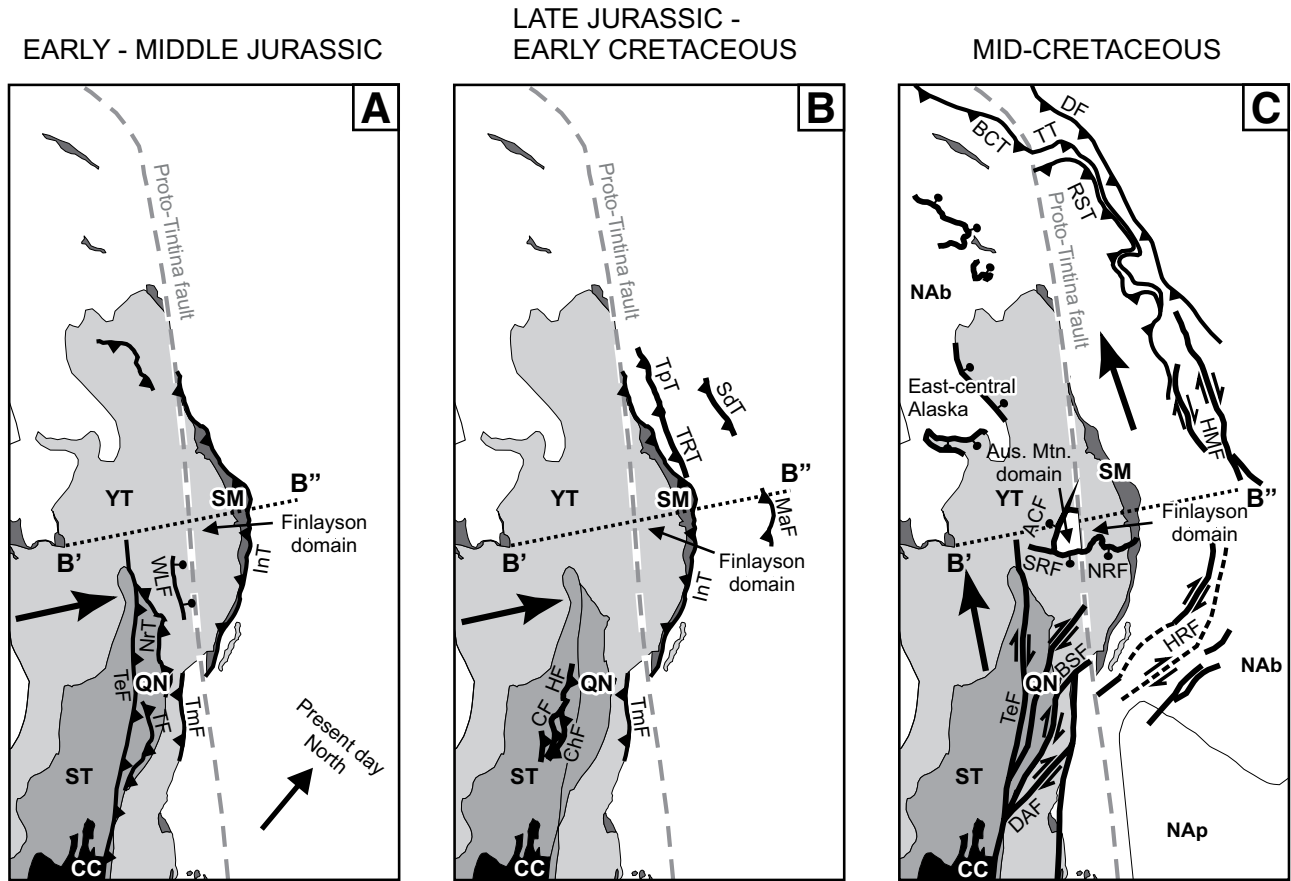
Figure 8. Generalized geological maps illustrating the orientation and kinematics of active structures at the time of each corresponding wedge section in Figure 7. Note, the geological maps are essentially static, in that they do not account for the amount of shortening during each time frame, and they are thus not a true plan view of what is shown in cross sections in Figure 7. Large black arrows illustrate the direction of crustal transport. The southwest-northeast-trending dotted line from B' to B'' is the approximate location of the schematic wedges in Figure 7. (A) Early–Middle Jurassic: characterized by northeast- and southwest-vergent thrust faults, reflecting a dynamic of orogen-normal compression and vertical extension (crustal thickening). (B) Late Jurassic–Early Cretaceous: Northeast- and southwest-vergent thrusts related to continued orogen-normal compression and vertical extension. (C) Mid-Cretaceous: This time was characterized by a change in the orogen's dynamics from orogen-normal shortening and thickening to lateral (orogen-parallel) extension as interpreted for the Stewart River and North River faults and comparable faults in east-central Alaska (Hansen and Dusel-Bacon, 1998; Dusel-Bacon et al., 2002). Fault abbreviations: ACF—Australia Creek fault; BCT—Beaver Creek thrust; BSF—Big Salmon fault; CF—Coghlan fault; ChF—Chain fault; DAF—D'Abbadie fault; DF—Dawson fault; HF—Hoochekoo fault; HMF—Hess-Macmillan fault system; HRF—Hyland River fault system; InT—Inconnu thrust; MaF—March fault; NRF—North River fault; NrT—Needlerock thrust; RST—Robert Service thrust; SdT—Sheldon thrust; SRF—Stewart River fault; TaF—Tadru fault; TeF—Teslin fault; TF—Towhata fault; TmF—Tummel fault; TT—Tombstone thrust; TpT—Twopete thrust; TRT—Tay River thrust; WLF—Willow Lake fault. City abbreviations: D—Dawson; Fb—Fairbanks; RR—Ross River; Wh—Whitehorse; WL—Watson Lake. Terrane abbreviations: CC—Cache Creek; QN—Quesnellia; ST—Stikine; YT—Yukon-Tanana; Nab—North America basinal strata; Nap—North America platform strata.
