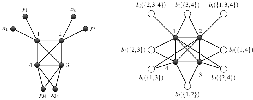
Fig. 4 The graph G for d = 1 and \mathcal{S} = \{\{1, 2, 3\}, \{1, 2, 4\}\} , as constructed in the proof of Theorem 1.5 (left) and in the proof of [15, Theorem 2] (right, where each white vertex represents a set of four vertices).
