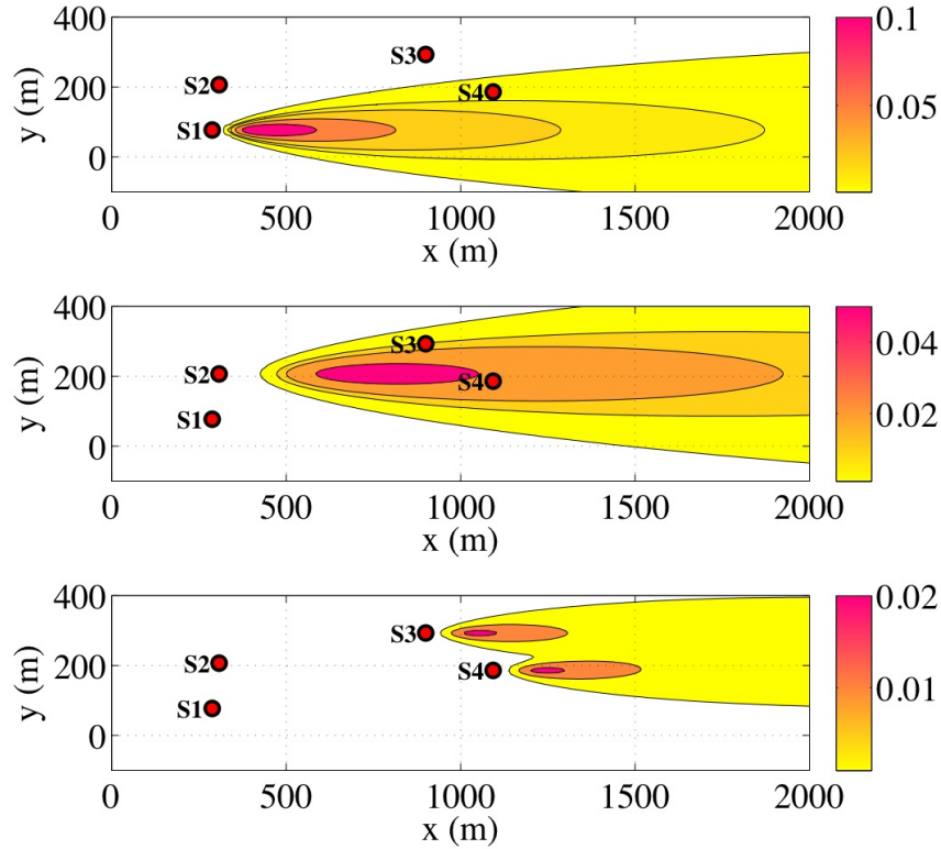
FIG. 3.3. Ground-level concentration (in \text{mg/m}^3 ) for the individual sources: S1 (top), S2 (middle), S3/S4 (bottom).
