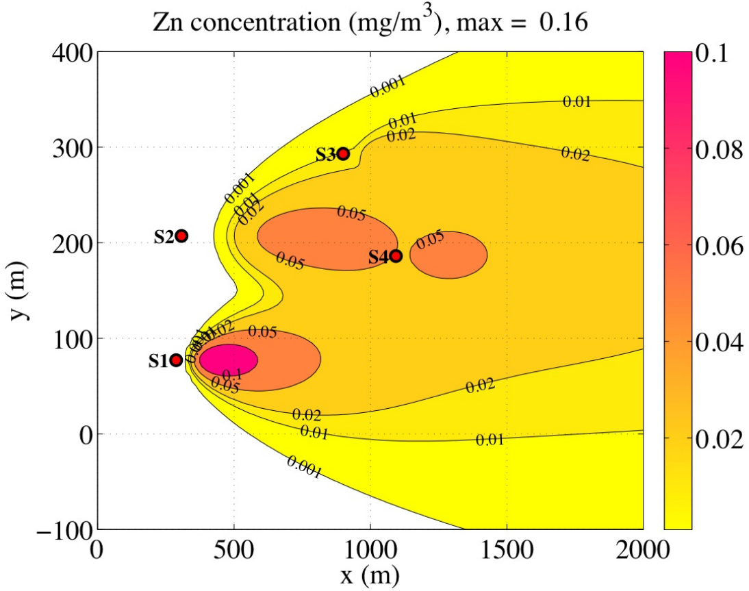
FIG. 3.4. Total ground-level concentration (in mg/m 3 ) for all four sources combined.
