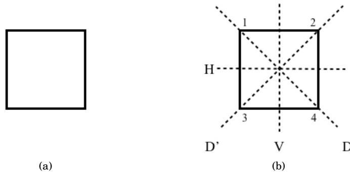
Figure 10.1: A square and its lines of symmetry.
