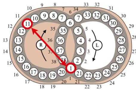
Figure 16.9: Fundamental 2-cycle: \sigma_2 = (1, 11) .
