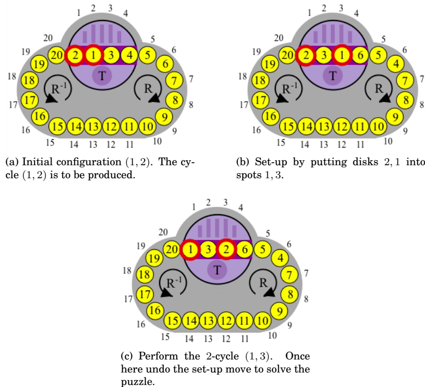
Figure 15.5: The steps for performing the 2-cycle (1, 2) as a conjugate of the 2-cycle (1, 3).
