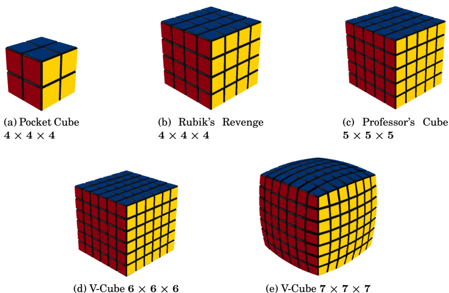
Figure 1.17: n \times n \times n Cubes
