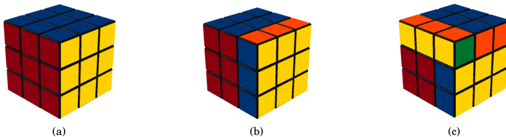
Figure 17.1: Three different configurations of Rubik’s cube.
