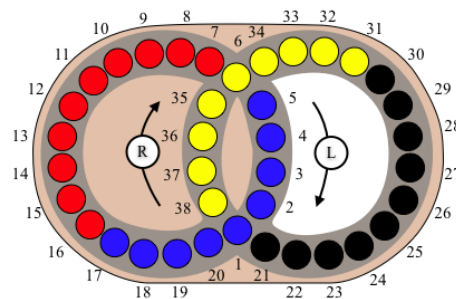
Figure 16.10: Hungarian Rings puzzle - coloured version.
