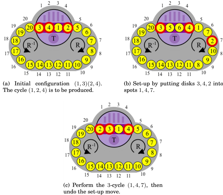
Figure 15.3: The steps for performing the 3-cycle (1, 2, 4) as a conjugate of the 3-cycle (1, 4, 7) .
