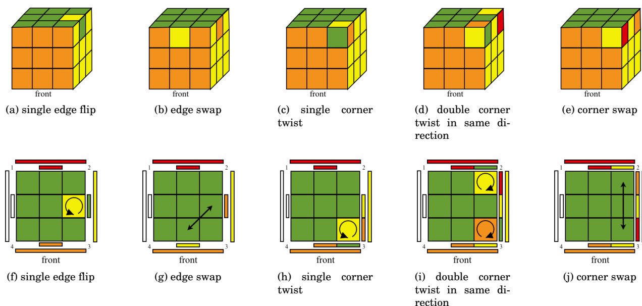
Figure 19.6: Five different moves that are impossible to perform. The image in the bottom row is a face-on perspective of the top face of the corresponding cube in the top row. The thin rectangular boxes on the sides indicate the colour of the side facets, and the long rectangular box indicates the side face colour.
