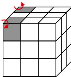
Figure 13.3: cubies moved by [L^{-1}D^2LBD^2B^{-1}, U] .
