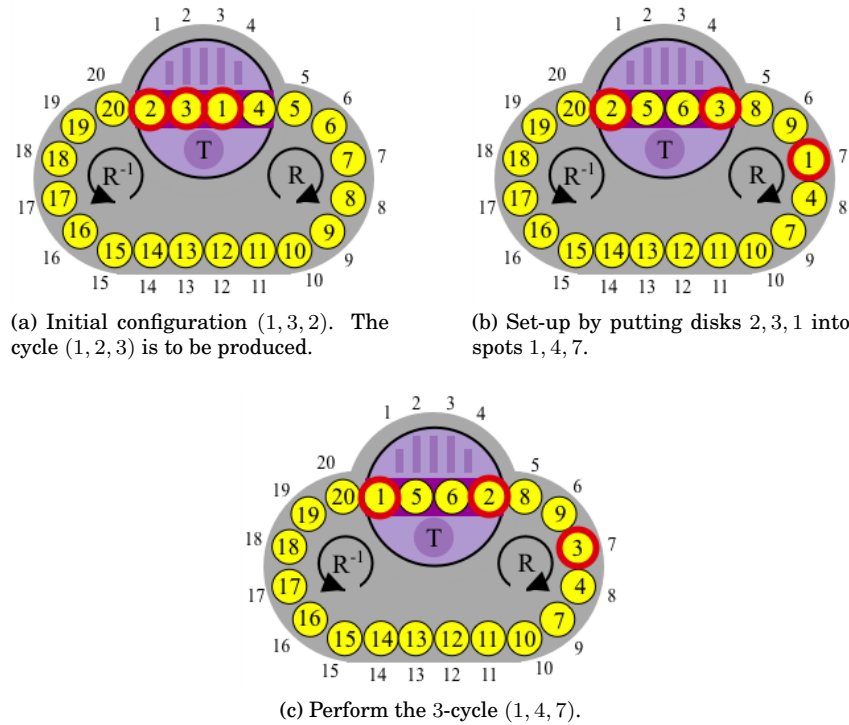
Figure 15.4: The steps for performing the 3-cycle (1, 2, 3) as a conjugate of the 3-cycle (1, 4, 7).
