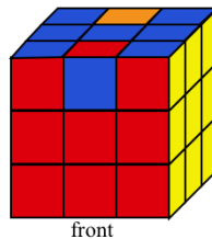
Figure 19.3: Cubie UF is in its home location, but not in its home orientation since it is flipped. Similarly for cubie UB .
