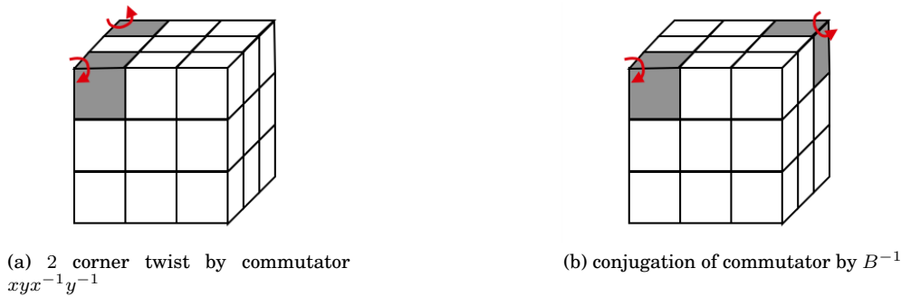
Figure 14.2: twisting 2 corner cubies
