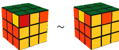
Figure 17.3: A corner swap is equivalent to an edge swap, but not equivalent to the solved state.
