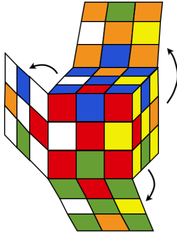
Figure 21.3: The superflip configuration of Rubik's Cube: X_{SF} .
