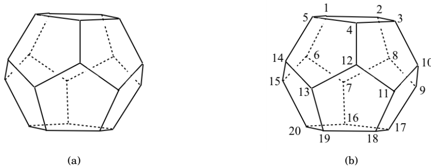
Figure 22.10: regular dodecahedron.
