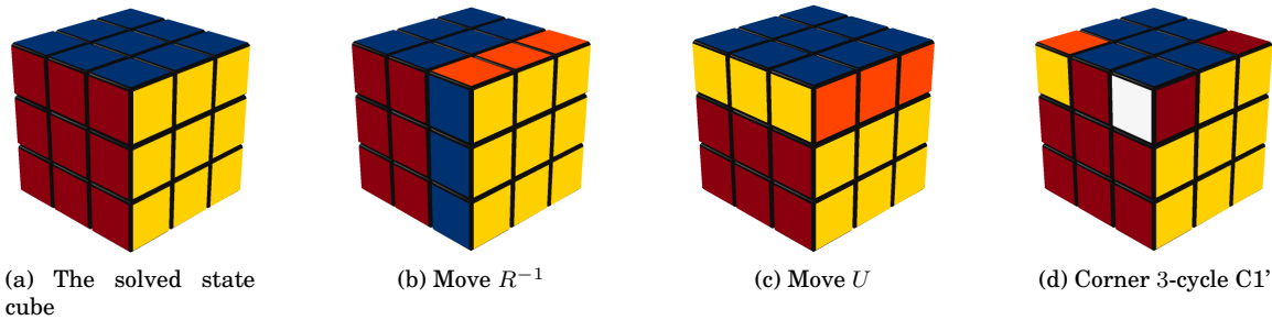
Figure 20.4: Configurations for Example 20.1.
