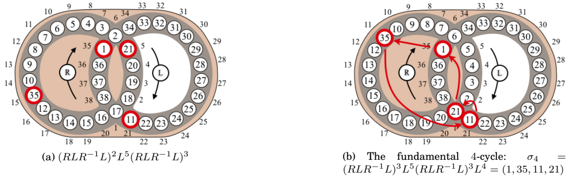
Figure 16.7: The set-up moves for creating the 4-cycle (1, 35, 11, 21) , continued.
