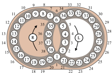
Figure 16.1: Hungarian Rings puzzle - numbered version.
