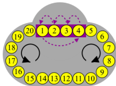
(a) One variation of the turntable move
