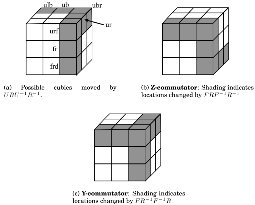
Figure 13.1: Y- and Z- commutators
