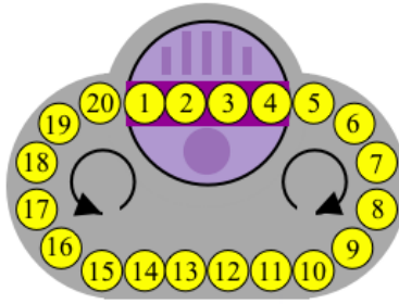
Figure 1.8: The TopSpin Puzzle in its solved state.
