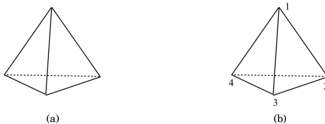
Figure 22.4: regular tetrahedron.
