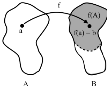
Figure 3.3: The way to visualize a function f , domain A , codomain B and range (shaded region).
