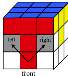
Figure 19.8: Moving an edge piece into the middle layer. To move right apply [D^{-1}, R^{-1}][D, F] , to move left apply [D, L][D^{-1}, F^{-1}] .
