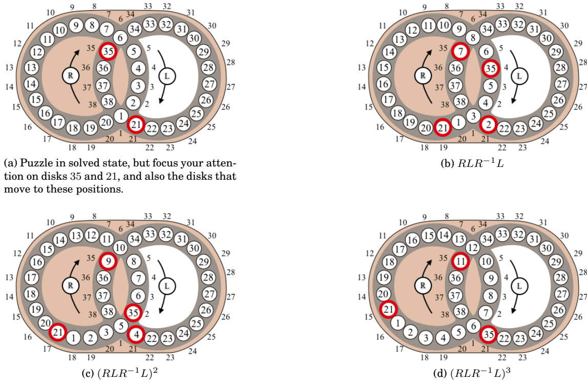
Figure 16.6: The set-up moves for creating the 4-cycle (1, 35, 11, 21).
