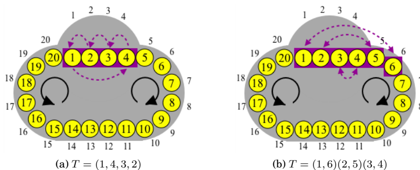
Figure 15.7: Some variation of the turntable move T for the Oval Track puzzle.
