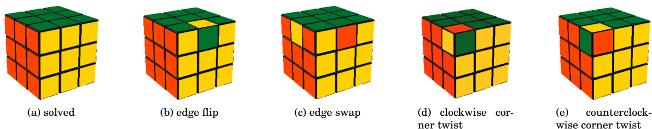
Figure 17.2: Five different equivalence class representatives of \mathcal{A} . How many more are there?
