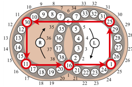
Figure 16.4: Fundamental 5-cycle: \sigma_5 = (L^5 R^5)^4 = (1, 25, 30, 11, 16) .
