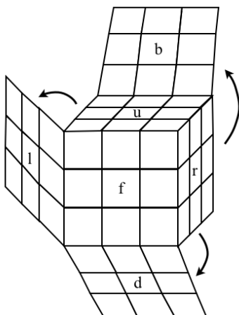
Figure 1.14: Labeling sides of Rubik's Cube by f , b , r , l , u , d .
