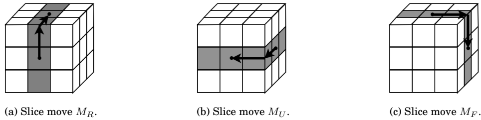
Figure 19.1: Three basic slice moves of Rubik's Cube.
