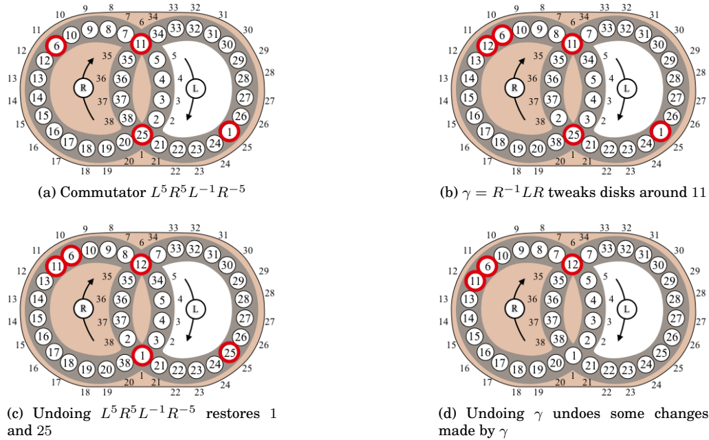
Figure 14.4: A compound commutator that uses the commutator [L^5, R^5] to construct a 3-cycle (6, 11, 12)
