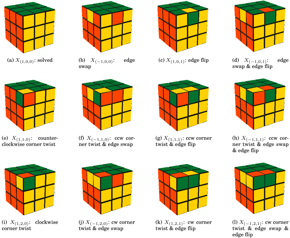
Figure 20.6: Representatives for the 12 different equivalence classes in RC_3^*
