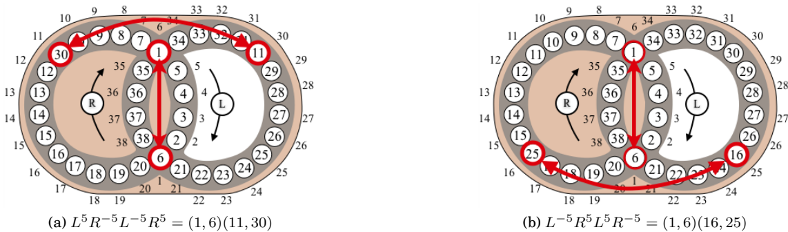
Figure 16.3: Basic commutators on the Hungarian Rings puzzle
