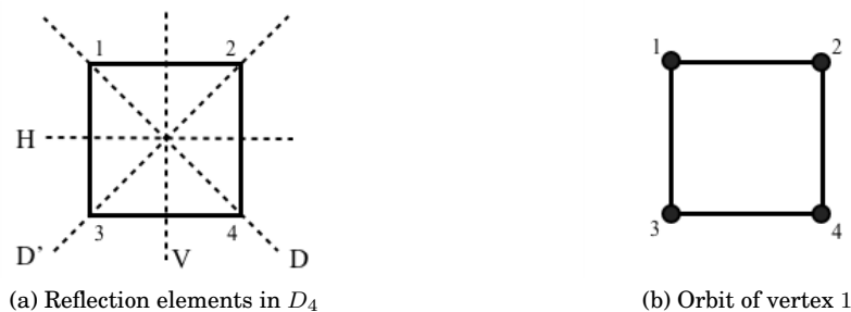
Figure 22.1: The group D_4 acting as a permutation group on the set of vertices.
