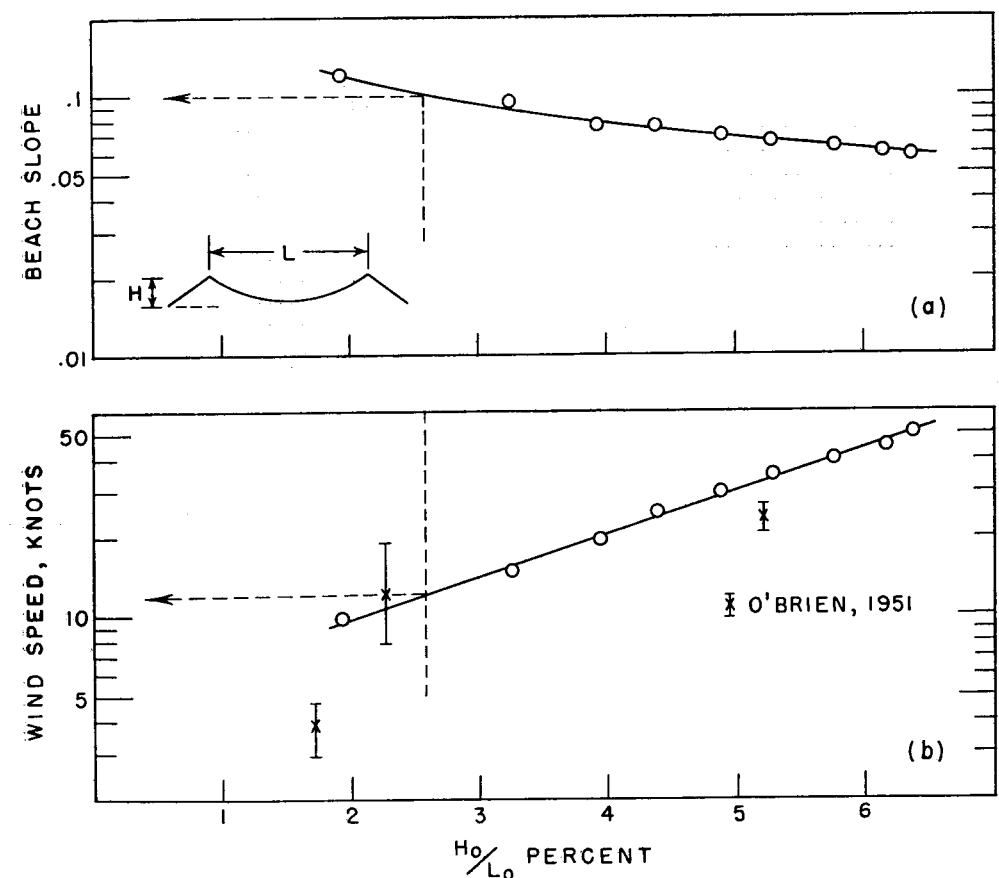
FIG. 4.—Interrelations of wind speed, wave characteristics, and beach slope
