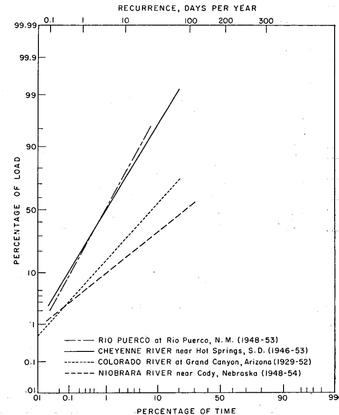
FIG. 2.—Plot of cumulative per cent of time against cumulative percentage of total suspended load
