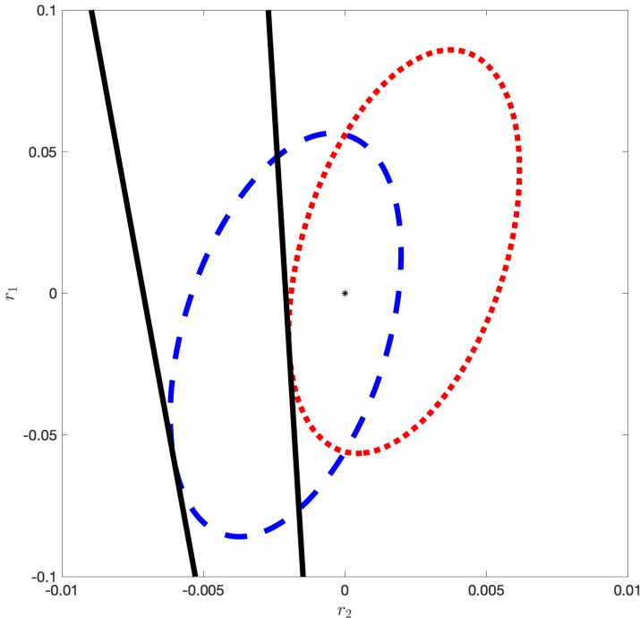
Figure 1: An illustration for section 6, figure 3 configuration for \mathbf{q}_{s,0} = .1 and \mathbf{q}_{u,s} = .2 . The figure displays parameter contours for (r_1, r_2) , holding relative entropies fixed. The upper right contour depicted with a red dots is for z equal to the .1 quantile of its stationary distribution under the baseline model and the lower left contour depicted with blue dashes is for z at the .9 quantile. The dot depicts the (r_1, r_2) = (0, 0) point corresponding to the baseline model. Tangency points denote worst-case structured models.
