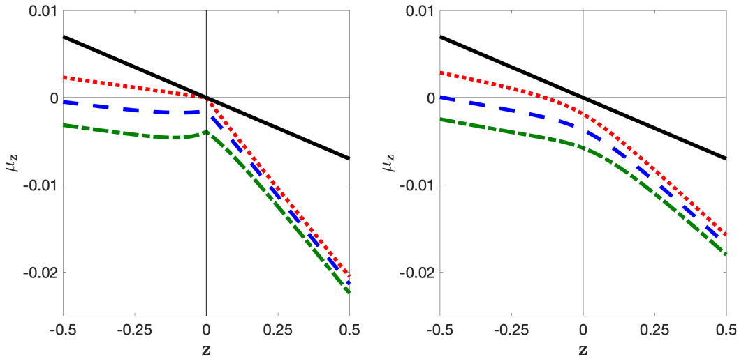
Figure 5: Distorted growth rate drift for Z . Relative entropy \mathbf{q}_{s,0} = .1 . Left panel: \rho_2 = \frac{(.01)}{|\sigma_z|^2} . Right panel: \rho_2 = \frac{(.01)}{2|\sigma_z|^2} . Black solid : baseline model; red dotted : worst-case structured model; blue dashed : \mathbf{q}_{u,s} = .1 ; and green dot-dashed : \mathbf{q}_{u,s} = .2 .
