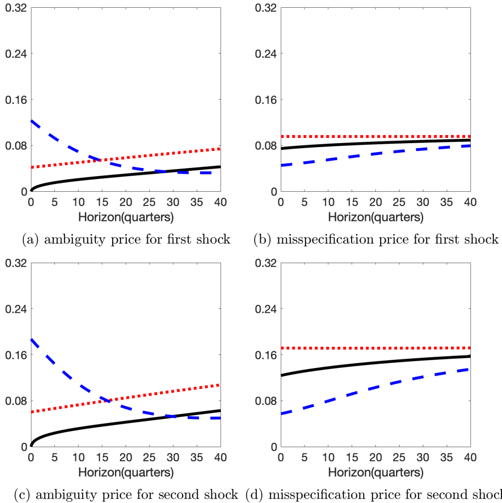
Figure 7: Contributions to shock price elasticities for alternative horizons. The panels in the left-hand side column plot the ambiguity component v^t(x) - \tilde{v}^t(x) . The panels in the right-hand side column plot the misspecification component \tilde{v}^t(x) . The change in exposure occurs at the same future date as the consumption payoff. In both cases \mathbf{q}_{s,0} = .1 . The figure reports the median and deciles for the section 6 specification with (\beta_c, \beta_z) structured uncertainty. Black solid : median of the Z stationary distribution red dotted : .1 decile; and blue dashed : .9 decile.
