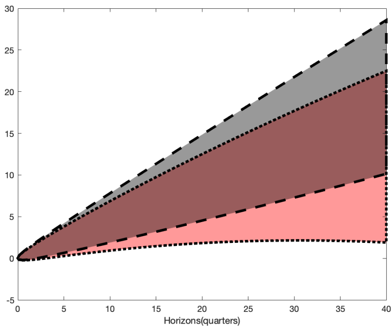
Figure 4: Distribution of Y_t - Y_0 under the baseline model and worst-case model for q_{s,0} = .1 and q_{u,s} = .2 . The gray shaded area between the dashed lines depicts the interval between the .1 and .9 deciles for every choice of the horizon under the baseline model. The red shaded area between the dotted lines gives the region within the .1 and .9 deciles under the worst-case model.
