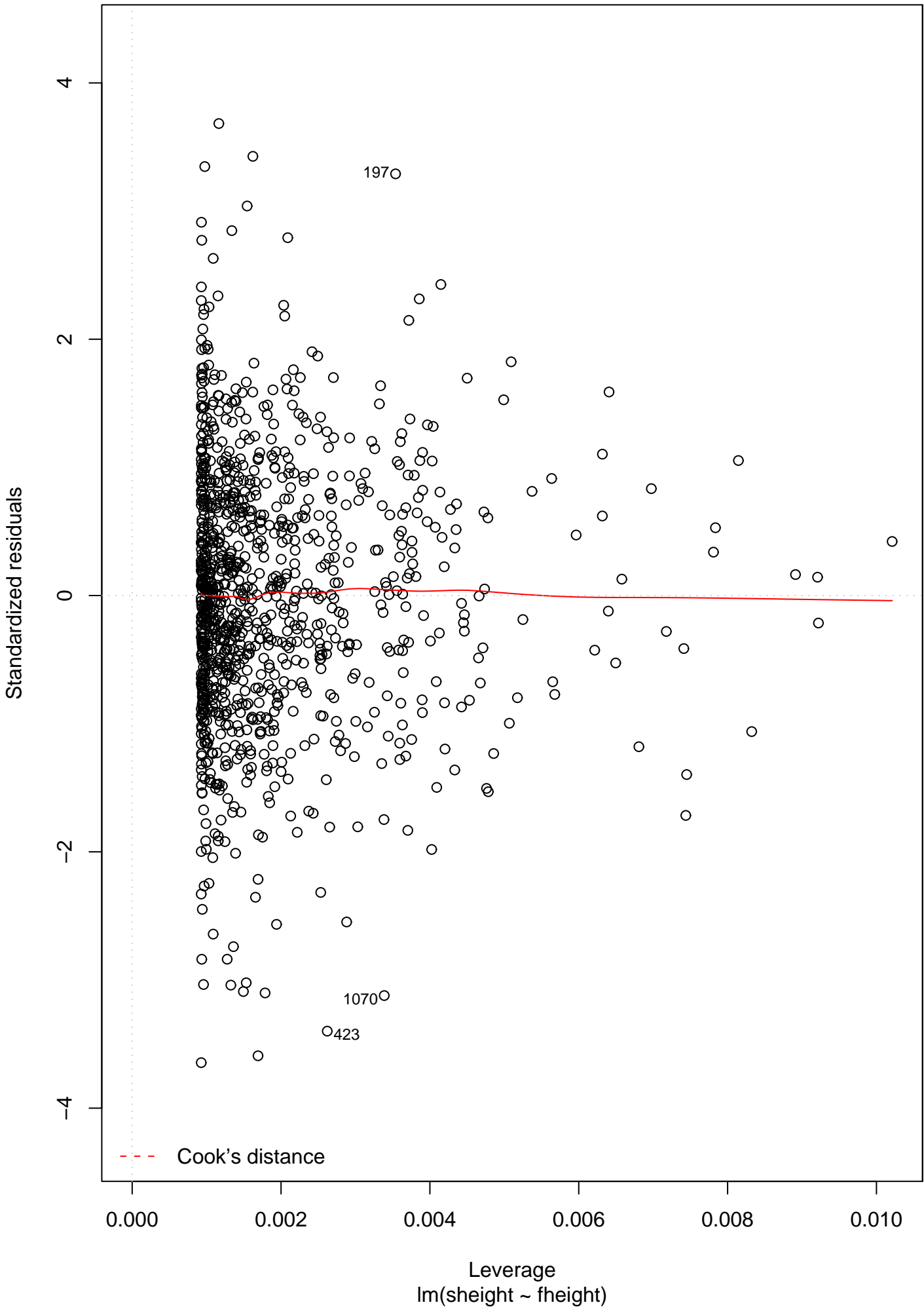
Residuals vs Leverage
