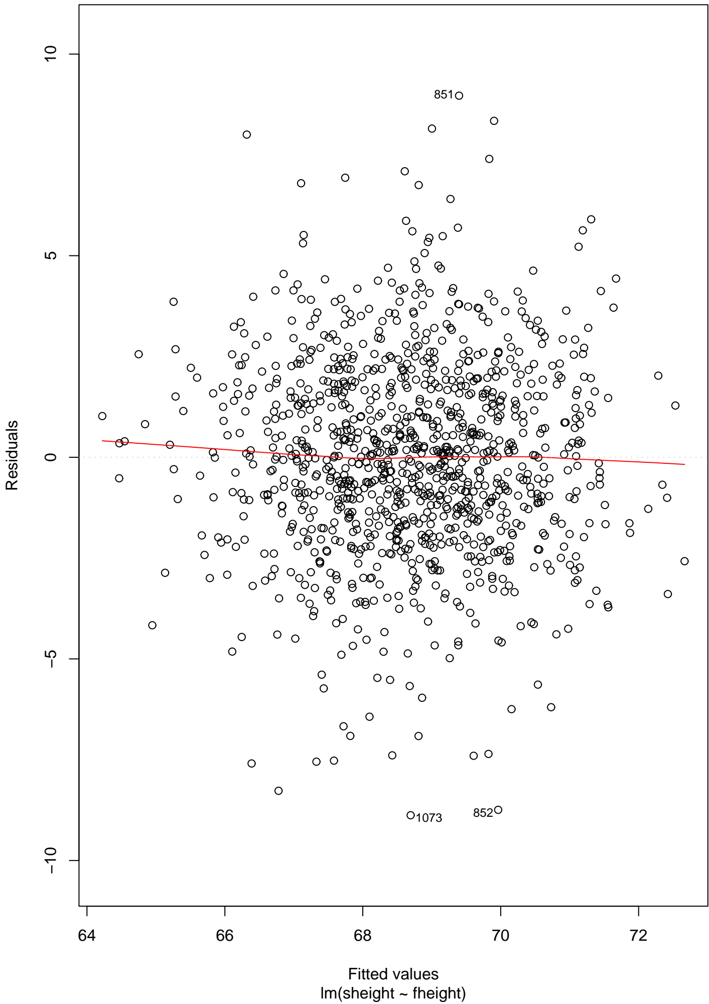
Residuals vs Fitted
