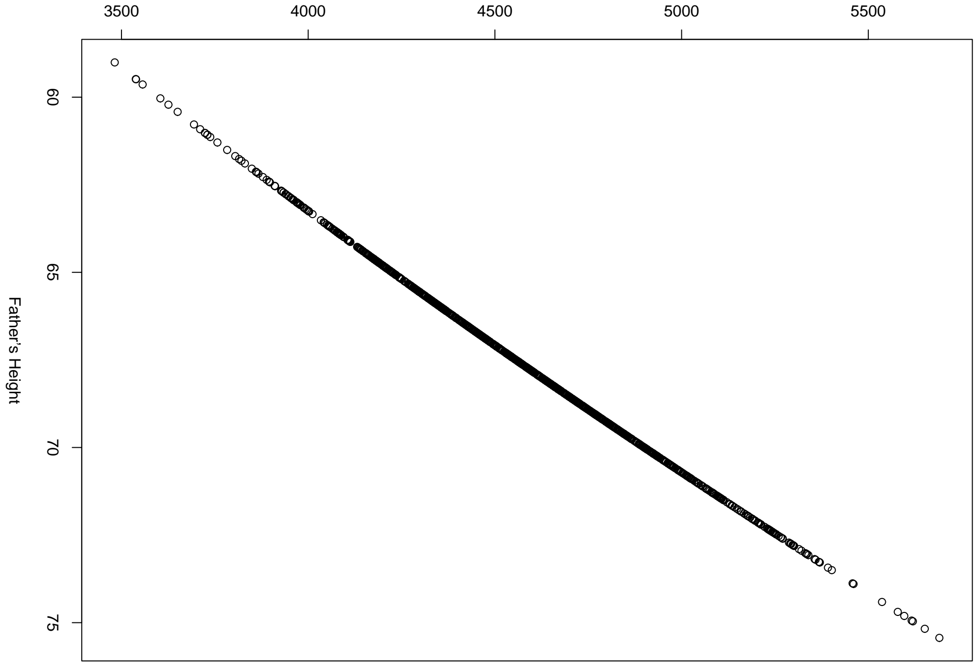
Father's Height Squared
