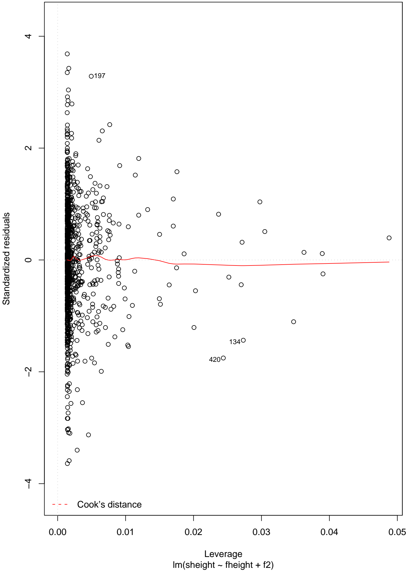
Residuals vs Leverage
