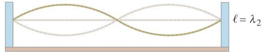
First overtone or second harmonic, f_2 = 2f_1
