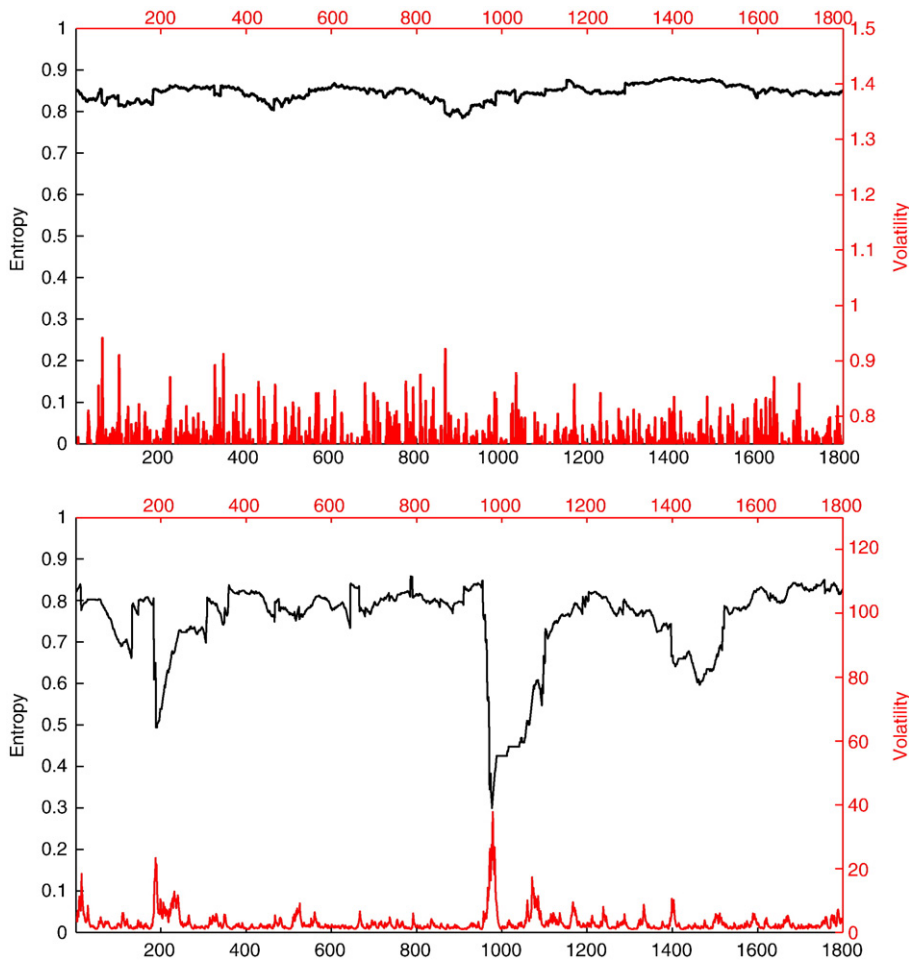
Fig. 2. Tsallis entropy with GARCH (1,1) process. For each panel, entropy values are on the left side of the vertical axis and the corresponding conditional volatility is on the right vertical axis. The GARCH (1,1) process is x_t = z_t \sigma_t , \sigma_t^2 = c + \alpha \varepsilon_{t-1}^2 + \beta \sigma_{t-1}^2 where z_t is an identically and independently distributed normal random variable with zero mean and unit variance. The entropy is calculated with q = 2 , n = 10 , K = 200 days and 2000 observations. The range of entropy is [0, 0.9] for q = 2 . In the top panel, the volatility persistence is set to be minimal with coefficients c = 0.5 , \alpha = 0.05 and \beta = 0.05 which leads to stable entropy across time. The spread of volatility across time does not exhibit large bursts and entropy fluctuates around a tight band of 0.85. The bottom level corresponds to a very persistent volatility with c = 0.5 , \alpha = 0.5 and \beta = 0.4999 . Outbursts of volatility are evident with 40% high peaks and it is clustered. The entropy falls dramatically in such high volatility periods and the dips in the entropy are evident relative to the top panel. In this example, the drop in the entropy in high volatility periods is contemporaneous with almost no lead time for predictability. In subsequent figures, we will demonstrate that it is possible to predict such high volatile periods with plenty of lead time using option based indicators and the entropy principle of belief heterogeneity.
