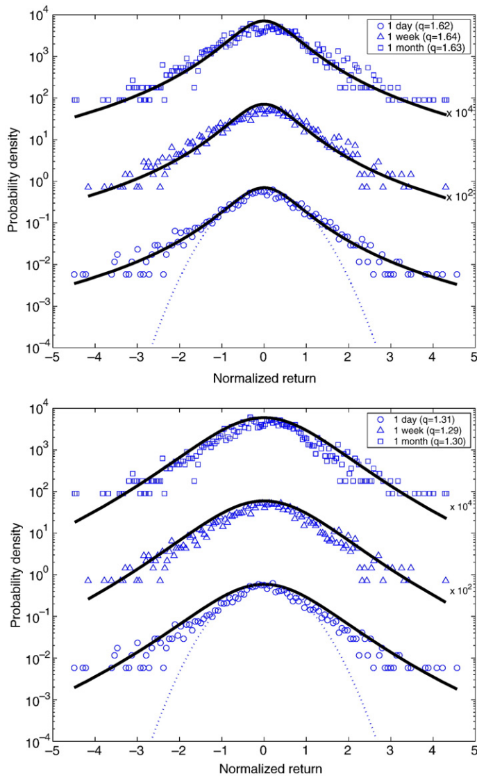
Fig. 1. Empirical histograms for the daily, weekly and monthly S&P-500 Index normalized returns (1990–2000). Normalized returns are plotted on the x-axis and the probability density on the y-axis as a log-linear plot. Top panel: The estimation of the optimal q involves minimizing the sum of the squared errors of the logarithms of the q -Gaussian probability density (solid line) and the data-implied empirical density (circles for the daily, triangles for the weekly, and squares for the monthly data). Bottom panel: The estimation of the optimal q is performed using the maximum likelihood estimator. The curves for the weekly and monthly data have been shifted vertically by 10^2 and 10^4 , respectively. The dotted line is the Gaussian distribution.
