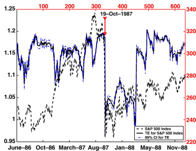
Fig. 4. Daily S&P-500 Index and dynamic entropy. Tsallis entropy (TE) values are on the left side of the vertical axis (solid line) and the daily S&P-500 Index for 1986–1988 is on the right vertical axis (dotted line). The time-dependent, discrete entropy is calculated from the daily S&P-500 Index based on the size of the moving window of K = 120 days. The entropy does not provide any lead time for predicting the October 19th crash. The sudden drop in the entropy is simultaneous with the drop in the index.
