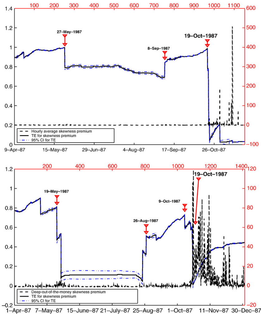
Fig. 3. Hourly skewness premium and dynamic entropy. For each panel, entropy values are on the left side of the vertical axis and the hourly skewness premium is on the right vertical axis. The size of the moving window is K = 500 hours ( \approx 60 days). In the top panel, the hourly average skewness premium ( x ) is plotted with the dotted line and time-dependent discrete Tsallis entropy (TE) for x is the solid line. The entropy dips on May 27, 1987 and recovers on September 8, 1987. In the bottom panel, hourly skewness premium ( x ) for the deepest (available)-out-of-the-money call and put options for 1987 is plotted with the dotted line and time-dependent discrete Tsallis entropy (TE) for x is the solid line. The entropy dips on May 20, 1987 and starts recovering on August 31, 1987. There is another sudden small drop a week before the crash.
