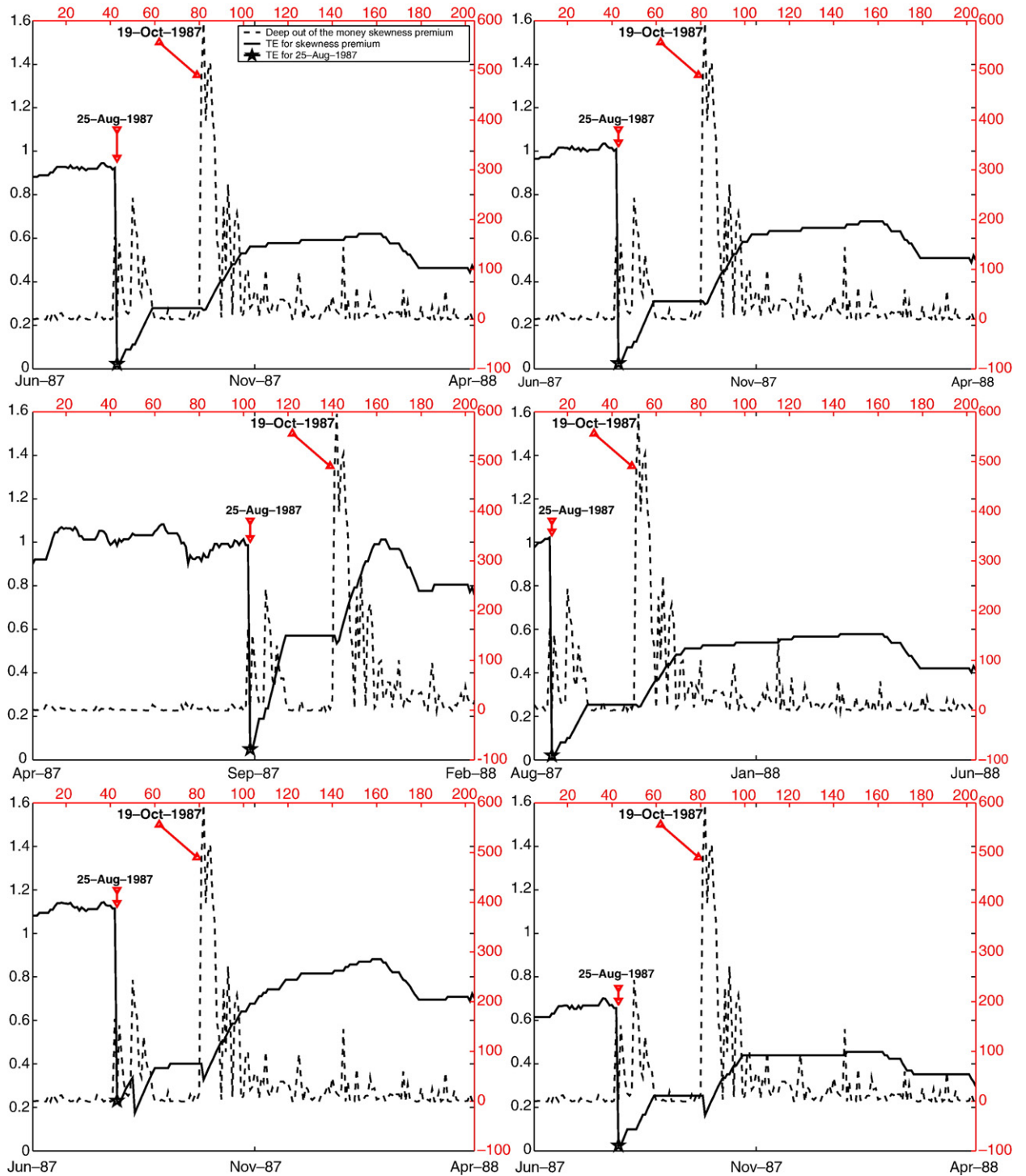
Fig. 6. Robustness testing. For each panel, entropy values are on the left side of the vertical axis (solid line) and the daily skewness premium for the deepest (available)-out-of-the-money call and put options is on the right vertical axis (dotted line). The entropy dips on August 25, 1987 and its level on that day is marked with the star. Robustness testing is performed with respect to the size of the moving window in days ( K ), number of states ( n ) and the optimal entropic index ( q ). Top left: K=120 , n=10 , and q=1.53 ; top right: K=120 , n=10 , and q=1.42 ; middle left: K=60 , n=10 , and q=1.42 ; middle right: K=150 , n=10 , and q=1.42 ; bottom left: K=120 , n=15 , and q=1.42 ; bottom right: K=120 , n=5 , and q=1.42 .
