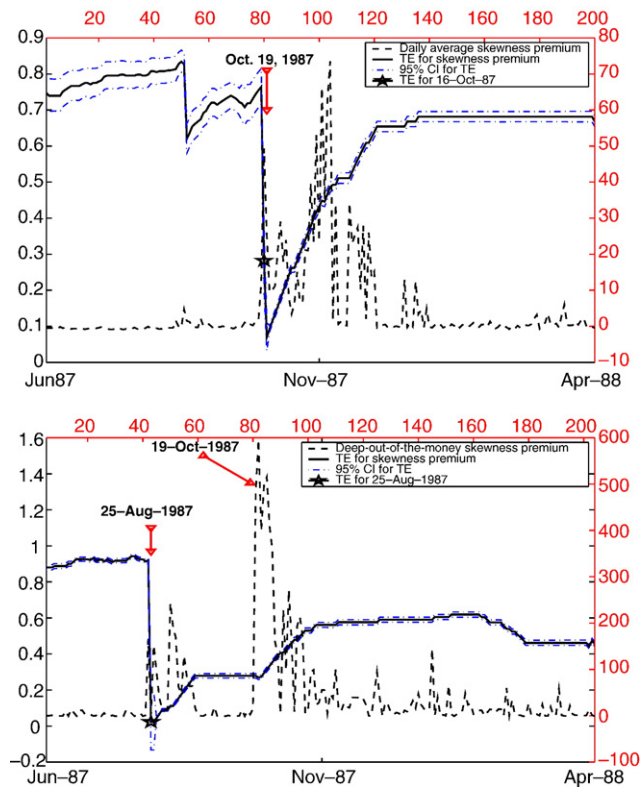
Fig. 5. Daily skewness premium and dynamic entropy. For each panel, entropy values are on the left side of the vertical axis and the daily skewness premium is on the right vertical axis. The size of the moving window is K = 120 days. In the top panel, daily average skewness premium ( x ) is plotted with the dotted line and time-dependent discrete Tsallis entropy (TE) for x is the solid line. The entropy dips on October 16, 1987 and its level on that day is marked with the star. In the bottom panel, daily skewness premium ( x ) for the deepest (available)-out-of-the-money call and put options is plotted with the dotted line and time-dependent discrete Tsallis entropy (TE) for x is the solid line. The entropy dips on August 25, 1987 and its level on that day is marked with the star.
