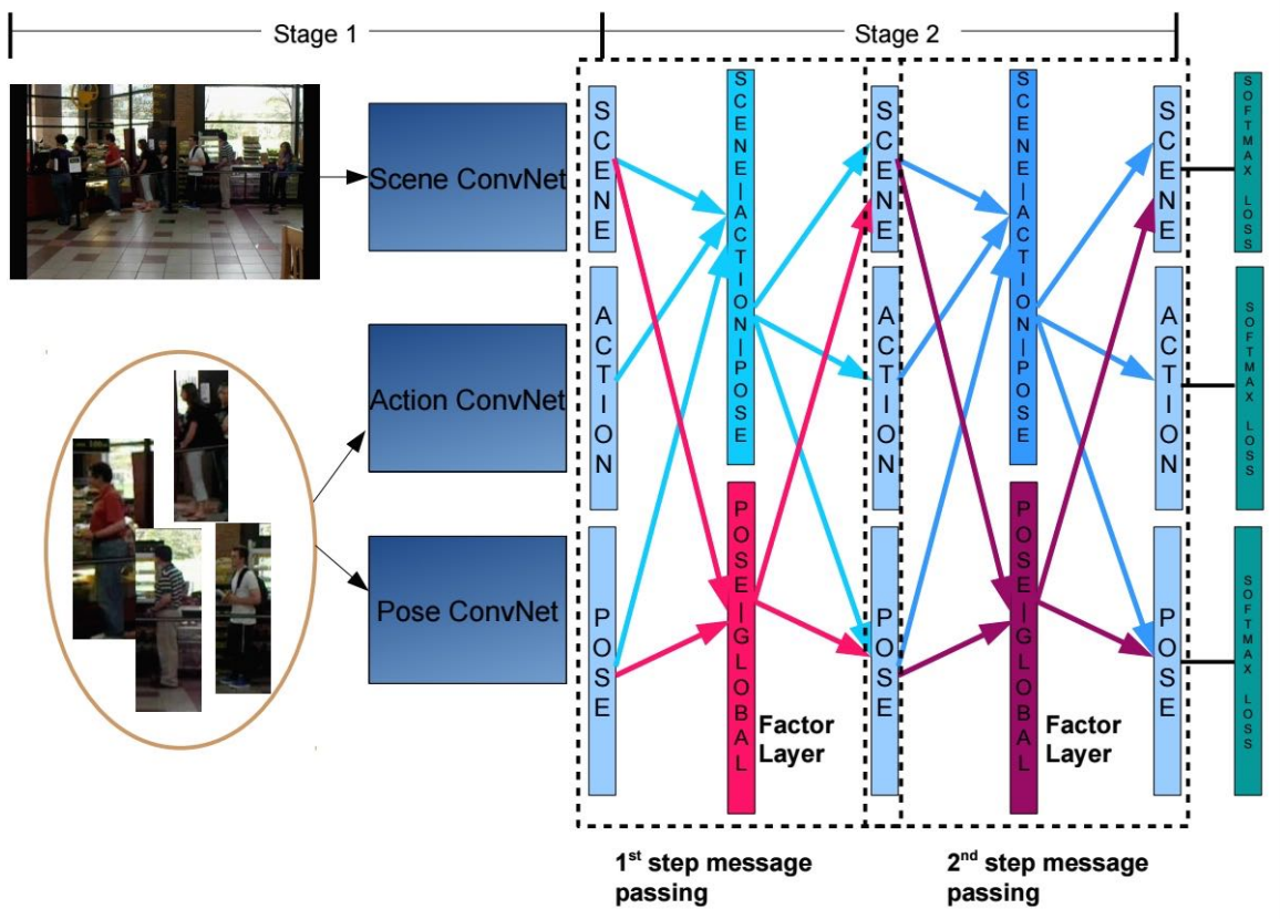
Figure 2.4: Overview of Deng et al. [7] deep structured model
