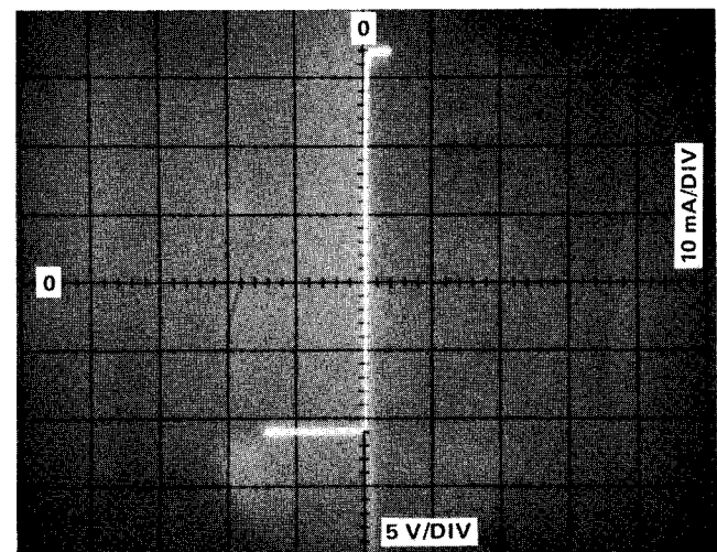
Fig. 58. 741 Linear IC, Supply Current vs. Supply Voltage.
