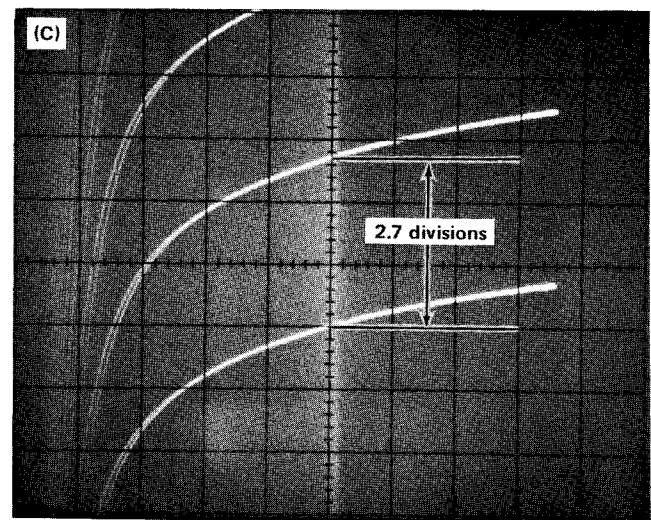
Fig. 14B, C. Illustration of step 19, g_m calculation (cont).
