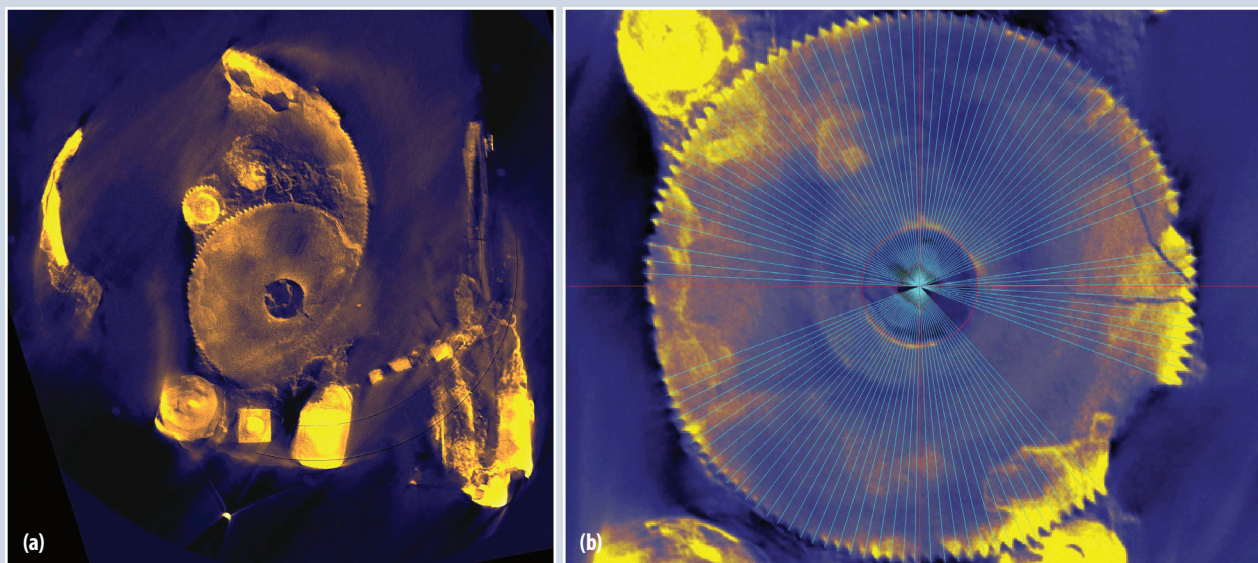
Figure 2. Typical X-ray CT slices, in a false color scale. (a) A gear with 127 teeth in the center that calculates the mean motion of the moon against the stars, according to the Metonic cycle. The large partial gear originally had 223 teeth and drives the Saros dial. (b) The 127-tooth gear, marked in Vectorworks for counting the teeth. Copyright 2006-2008 Antikythera Mechanism Research Project.
