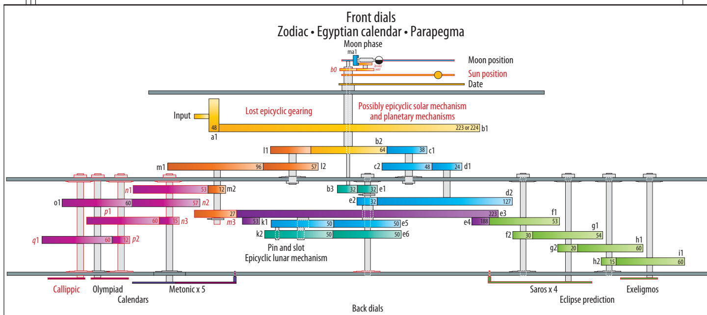
Figure 4. Schematic gear diagram. Elements in black are those for which there is evidence; those in red are conjectural. Note that two gears have 38 teeth ( = 2 \times 19 ); one gear has 127; and one gear (or possibly two) has 223. Three gears have 53 teeth, the first of which contributes to the correct rotation for the lunar anomaly; the other two cancel out the effect of the first, where this prime factor isn't wanted. Copyright 2011 Images First Ltd.
