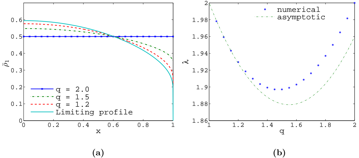
Figure 5: (a) Normalized steady states \bar{\rho}_1^\epsilon for \epsilon = 1, 0.5, 0.2 ( q = 2, 1.5, 1.2 ) computed directly from (53) using the numerical methods from Section 4.1. The plain solid line represents the leading order term \bar{\rho}^{(0)} of the expansion (54b). Equilibria \bar{\rho}_1^\epsilon approach the limiting profile \bar{\rho}^{(0)} as \epsilon \rightarrow 0 . (b) Eigenvalues \lambda_\epsilon for various values of \epsilon \in (0, 1] ( q \in (1, 2] ), computed directly from (53) (dots). The dashed line is the asymptotic approximation of \lambda^\epsilon from (54a) valid at order O(\epsilon^2) . Note the excellent agreement between numerics and asymptotics for small \epsilon ( q close to 1).
