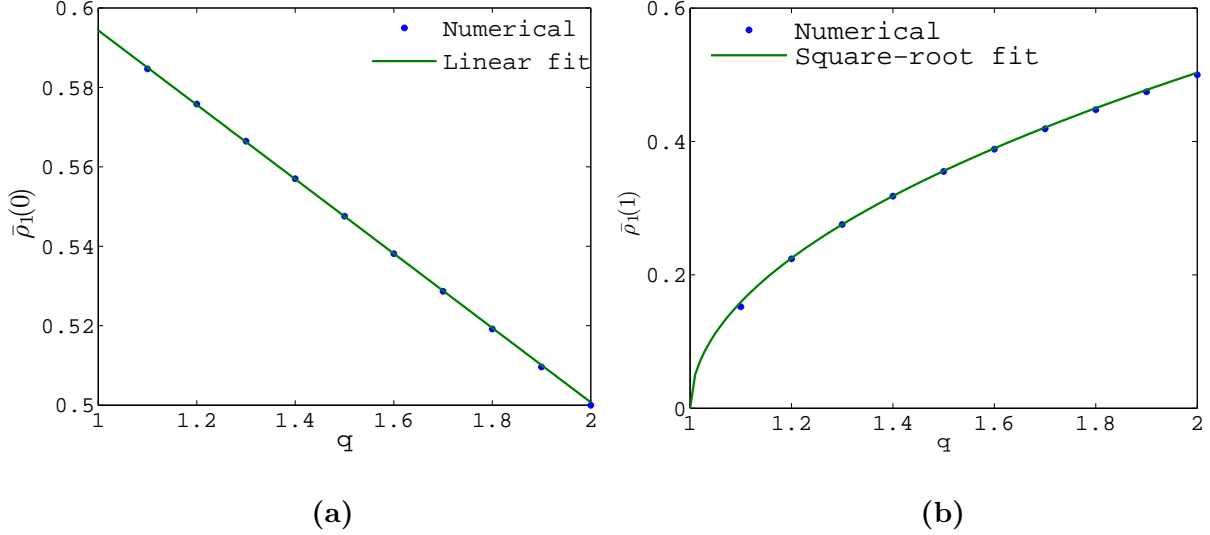
Figure 6: (a) Validation of the asymptotic expansion (54b) away from the boundary. At x = 0 , \bar{\rho}_1^\epsilon(0) has a linear dependence on \epsilon of the form 0.5944 - 0.0936\epsilon , as the expansion (54b) is uniform near the origin. (b) At x = 1 , \bar{\rho}_1^\epsilon(1) has a square-root dependence on \epsilon of the form \sqrt{0.2530\epsilon} . There is a boundary layer near x = 1 where the expansion (54b) is no longer valid.
