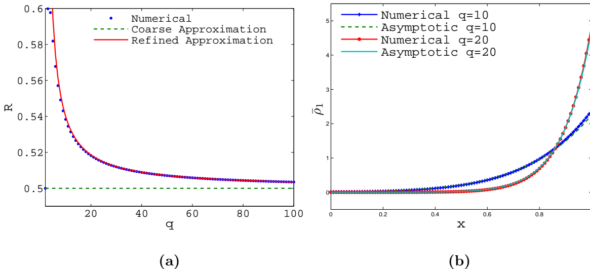
Figure 3: Numerical and asymptotic solutions in dimension one, as q \rightarrow \infty . (a) Radius R of the steady states (24). The refined asymptotic approximation (48) (solid line) agrees extremely well with the numerical solution (dots). The coarse approximation R = 0.5 (dashed line) captures the (slow) asymptotic limit, as q \rightarrow \infty . (b) Eigenfunctions \bar{\rho}_1 of T_1 computed by numerical (Section 4.1) and asymptotic (equation (47)) methods. The agreement between the two sets of results is excellent.
