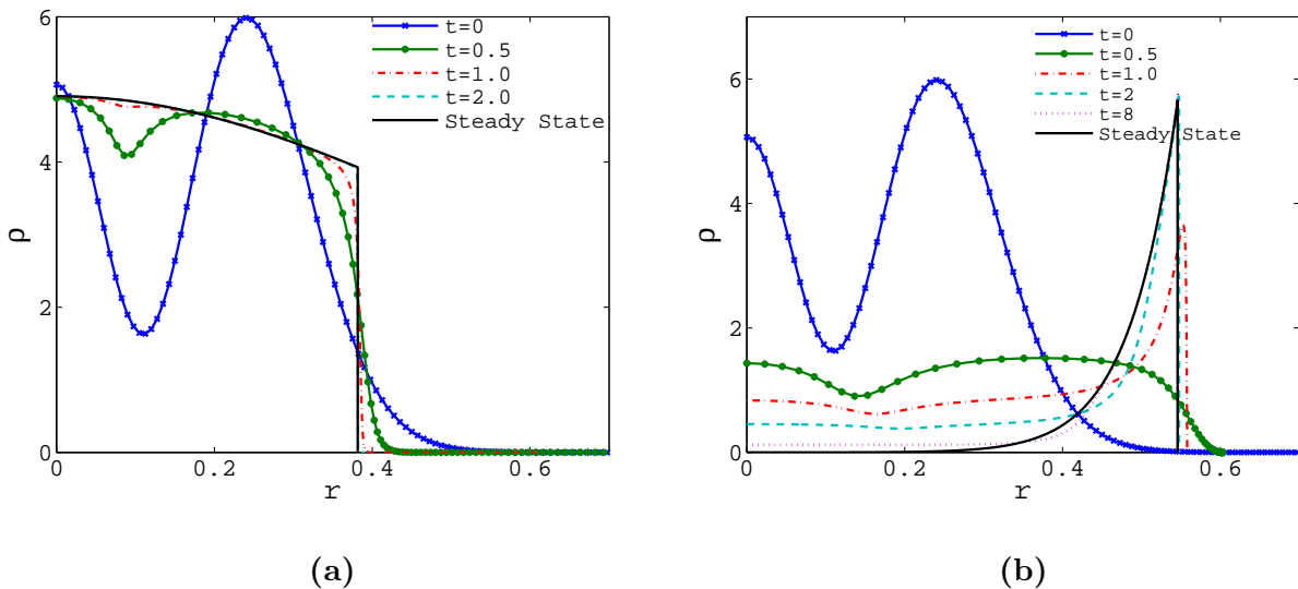
Figure 2: Time evolution of a radially symmetric solution to the aggregation model (1)-(2) with (a) q = 1.5 and (b) q = 20 , in three dimensions, starting from initial data (42). The solutions approach asymptotically the steady states studied in Section 3 (solutions to (24)) and shown in Figure 1. Numerics with a variety of other initial conditions suggests that these equilibria are global attractors for the dynamics of (1)-(2).
