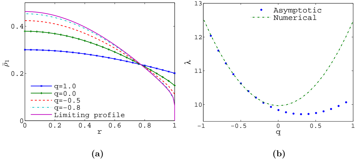
Figure 7: (a) Equilibria \bar{\rho}_1^{\epsilon} in three dimensions for \epsilon = 2, 1, 0.5, 0.2 ( q = 1, 0, -0.5, -0.8 ) computed numerically from (43) (see Section 4.1). The plain solid line is the limiting profile \bar{\rho}^{(0)} found by inverse iteration from (61b). As \epsilon \rightarrow 0 , \bar{\rho}_1^{\epsilon} approaches the limiting profile, confirming the asymptotic expansion. (b) Comparison between numerics and asymptotics in three dimensions: eigenvalues obtained numerically from (43) (dots) and from the asymptotic expansion (54a) valid at order O(\epsilon^2) . The two sets of results agree very well for small \epsilon ( q close to -1 ).
