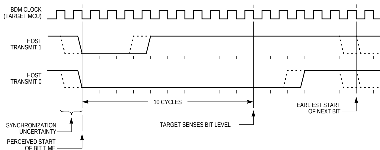
Figure 8-1. BDM Host to Target Serial Bit Timing
