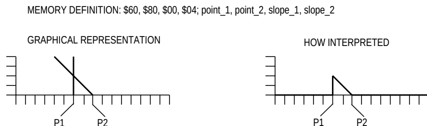
Figure 9-8. Abnormal Membership Function Case 3
