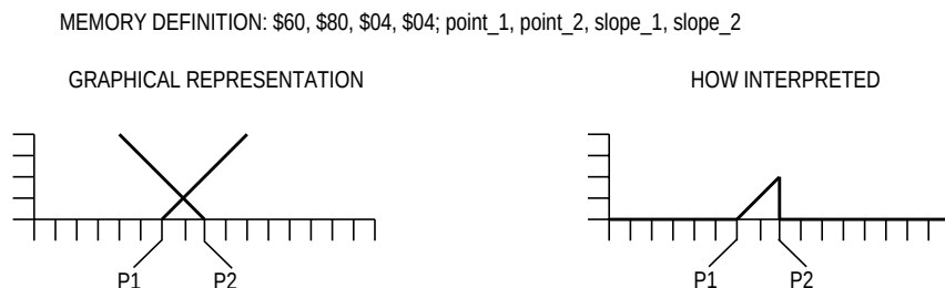
Figure 9-6. Abnormal Membership Function Case 1
