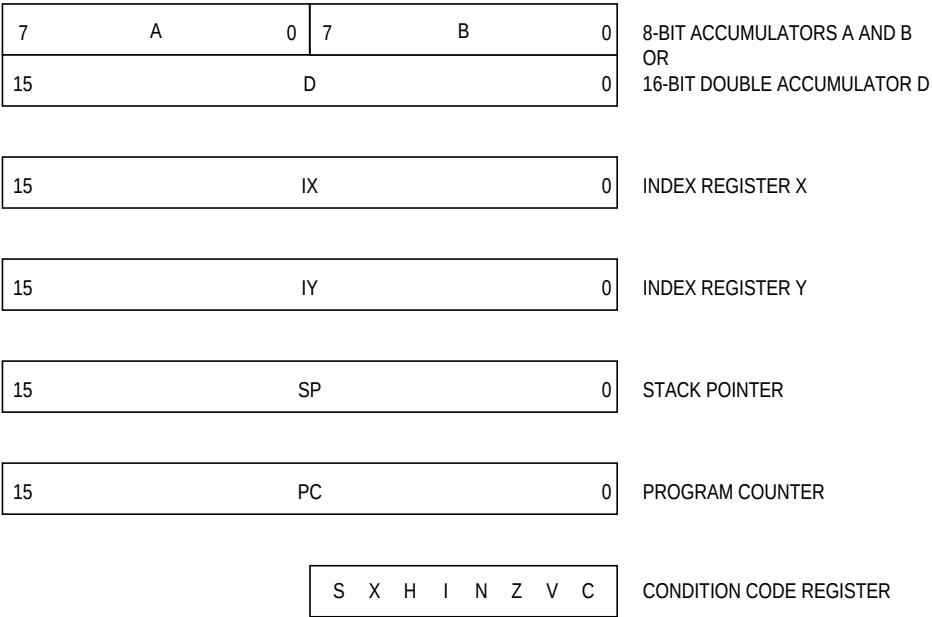
Figure 2-1. Programming Model
