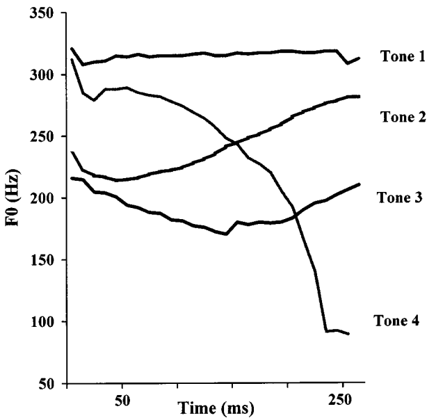
FIG. 1 F0 contours for the four Mandarin tones, each combined with the syllable guo .
