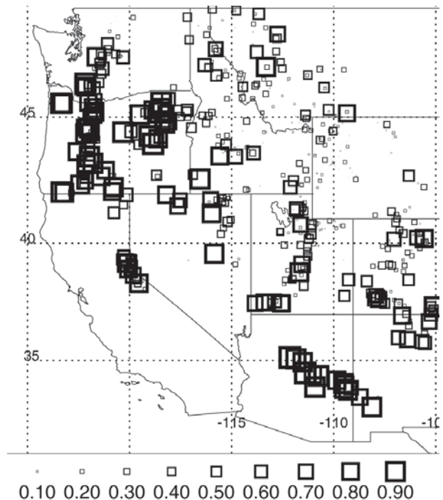
FIG. 5. Correlations from SNOTEL data of total daily melt events (the sum of negative changes in SWE from 1 Oct to 31 Mar) and 1 Apr SWE. The size of the square corresponds to correlation, and all correlations are negative. In the warmer mountains, winter melt events have a strong (negative) influence on 1 Apr SWE.
