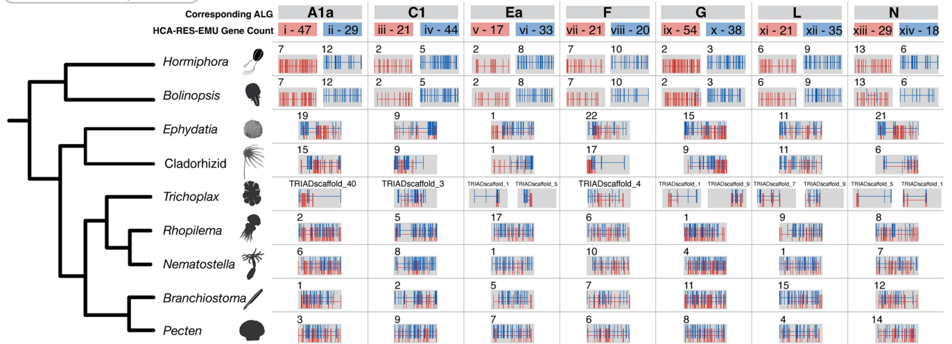
Extended Data Fig. 8 | Mixing plots of HCA-EMU-RES reciprocal best blastp results. This figure parallels Fig. 3 of the main text, but includes more genes by requiring orthology between metazoans without requiring orthologs in corresponding outgroups. Limiting the macrosynteny search to animals shows many genes participating in the extension of metazoan ALGs to the ctenophores.
