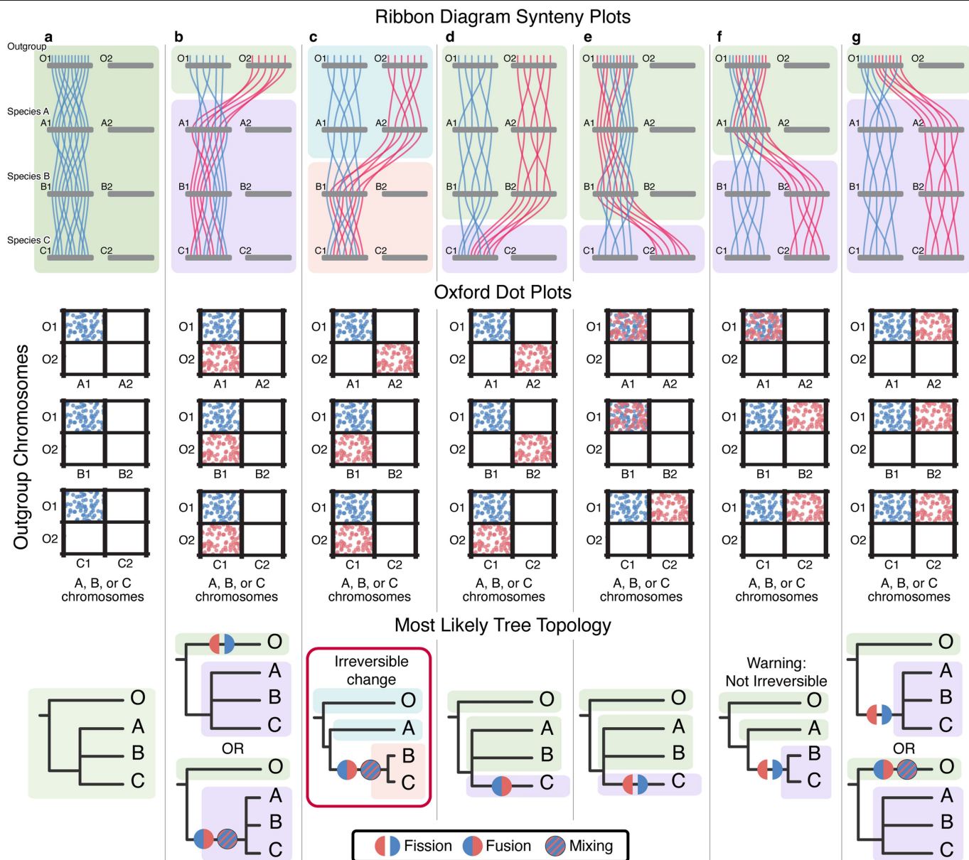
Extended Data Fig. 4 | Seven basic ALG configurations in species quartets. a-g. The seven configurations of ALGs found in four species highlight the evolutionary history of chromosomes. The cartoon ribbon plot in each panel shows chromosomes (horizontal bars) and the positions of genes in two ALGs
