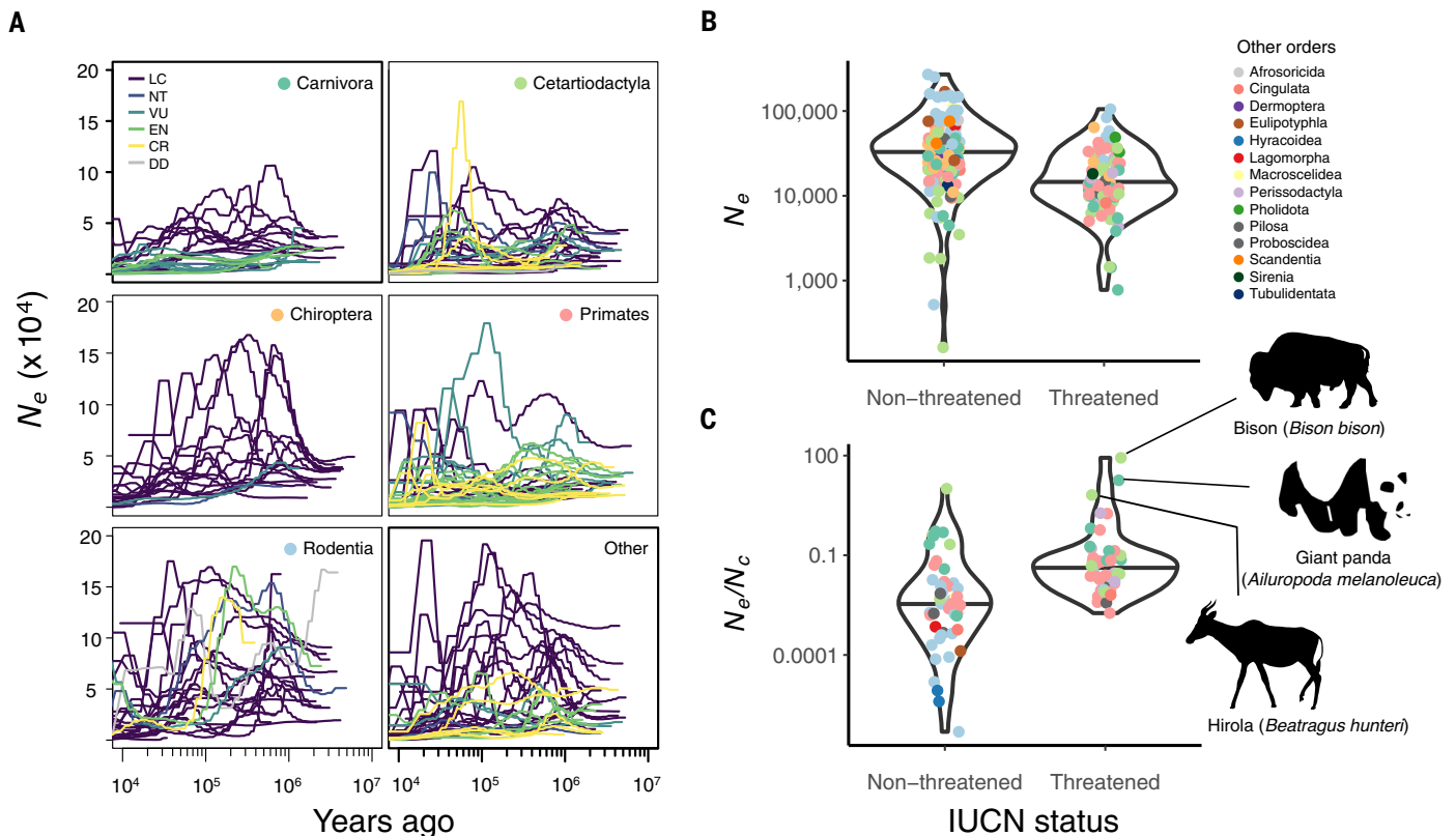
Fig. 1. Demographic history across mammalian orders and IUCN Red List categories. (A) Estimates of effective population sizes ( N_e ) over time, displayed by taxonomic order. Lines represent individual species, colored by IUCN status (LC, Least Concern; NT, Near Threatened; VU, Vulnerable; EN, Endangered; CR, Critically Endangered; DD, Data Deficient). Colored dots correspond to the taxonomic order of species depicted in (B) and (C). For visualization, only species with N_e estimates
