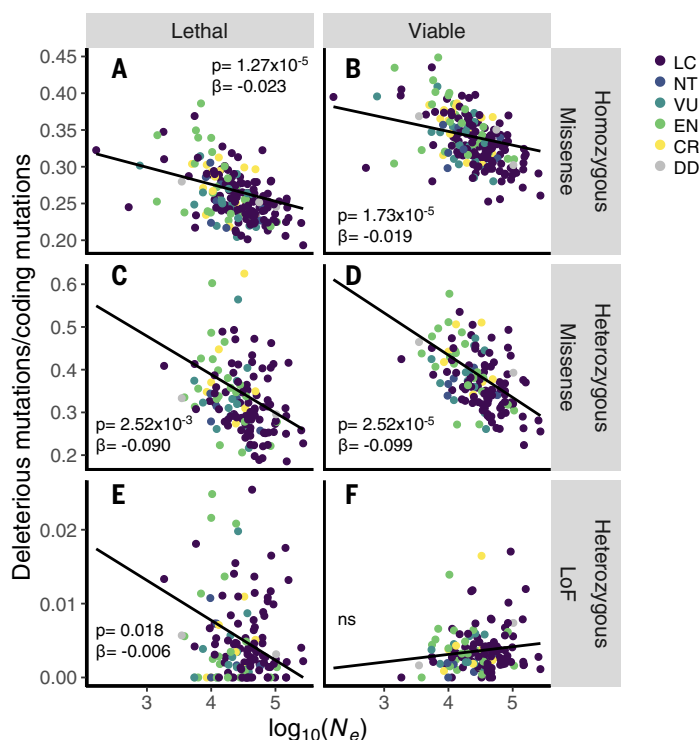
Fig. 2. Historically small populations have higher deleterious genetic load in protein-coding genes.
