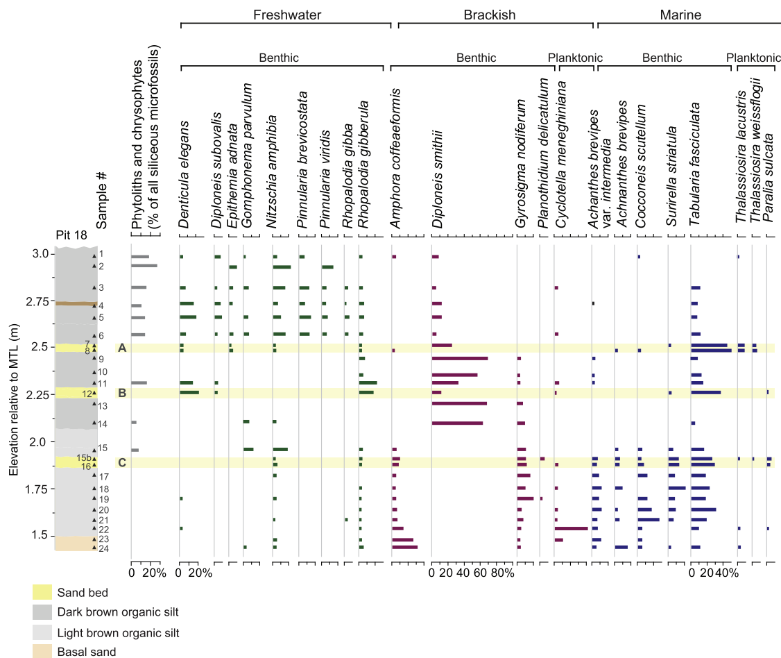
Fig. 9. Summary of microfossil analyses for pit 18. Triangle symbols on stratigraphic column show locations of numbered samples. Relative abundance of diatoms (showing only those species that are ecologically diagnostic) is expressed as a percent of the total count. Abundance of grass phytoliths and chrysophyte cysts expressed as a percent of total siliceous microfossils.
