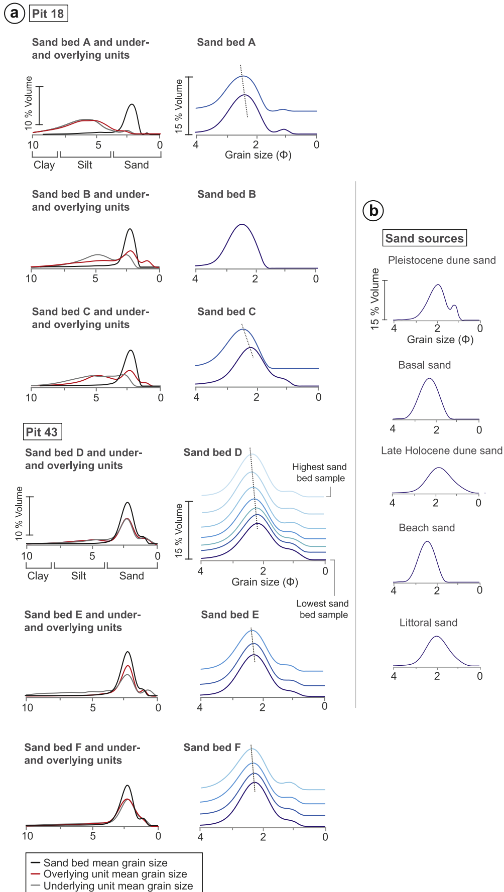
Fig. 7. a) Grain-size differential volume curves for stratigraphic units and sand beds F-A. Lines connecting differential volume curves show normal grading in sand beds. b) Grain size differential volume curves for modern surface sediments of the Quintero lowland.
