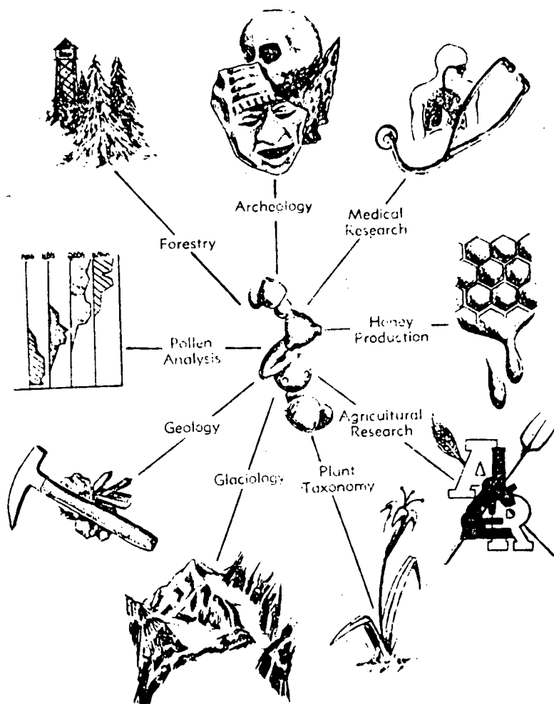
Some important applications of palynology. KAPP (1969)
