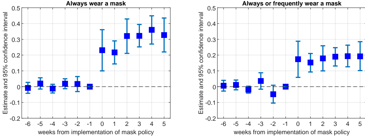
Figure 5: Event Study of Self-reported Mask Usage – Canada
