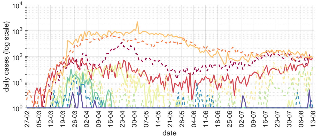
Figure B10: Canada – Daily cases, deaths and tests
