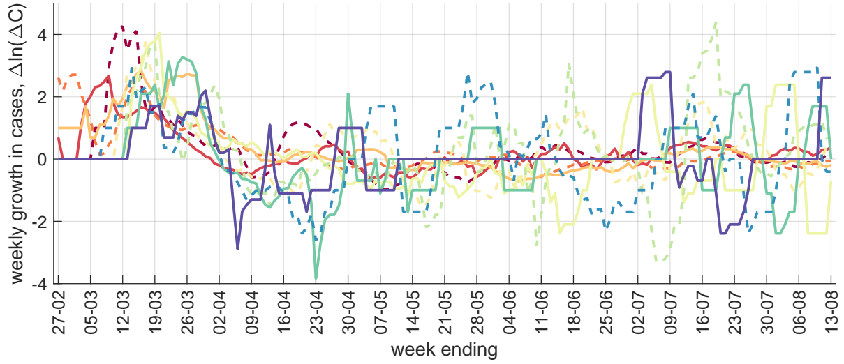
Figure B8: Canada – Weekly cases, deaths and tests (growth rate)
