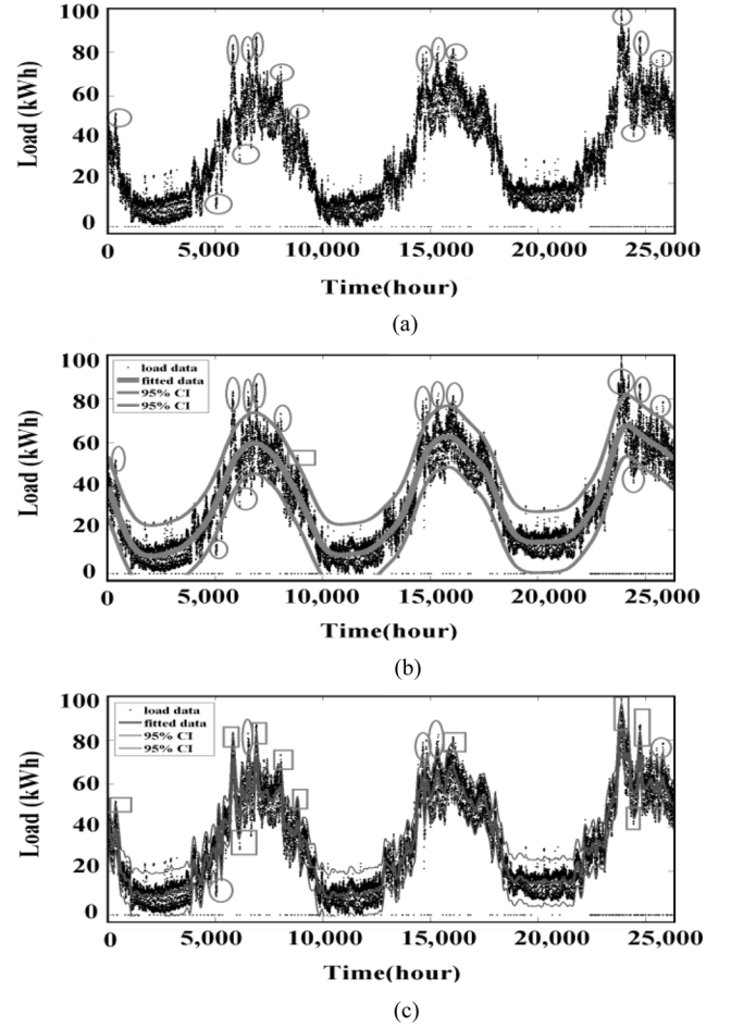
Fig. 5. Globally corrupted data detection for the three-year testing data. The predefined 10 smoothness levels are different in locally and globally corrupted data detection (refer to Section IV-C). (a) Three-year testing data with 15 globally corrupted regions. (b) B-Spline smoothing result with smoothness Level 7. (c) B-Spline smoothing result with smoothness Level 4.
