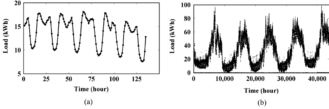
Fig. 3. Local patterns and global patterns in load curve data. (a) Local patterns. (b) Global patterns.
