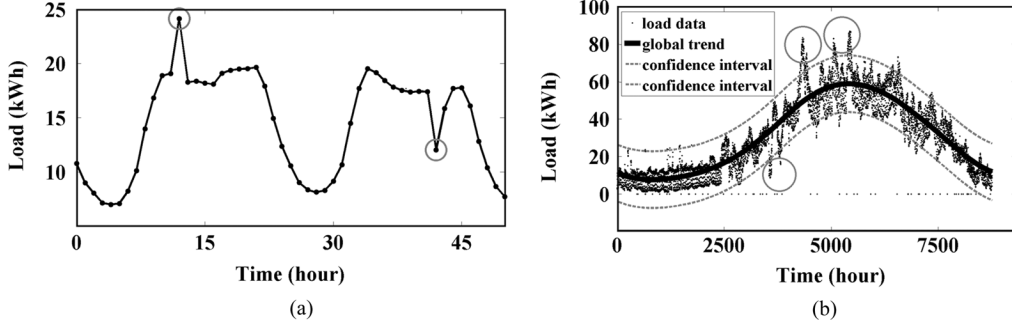
Fig. 1. Examples of locally and globally corrupted data (regions). (a) Locally corrupted data. (b) Globally corrupted data.
