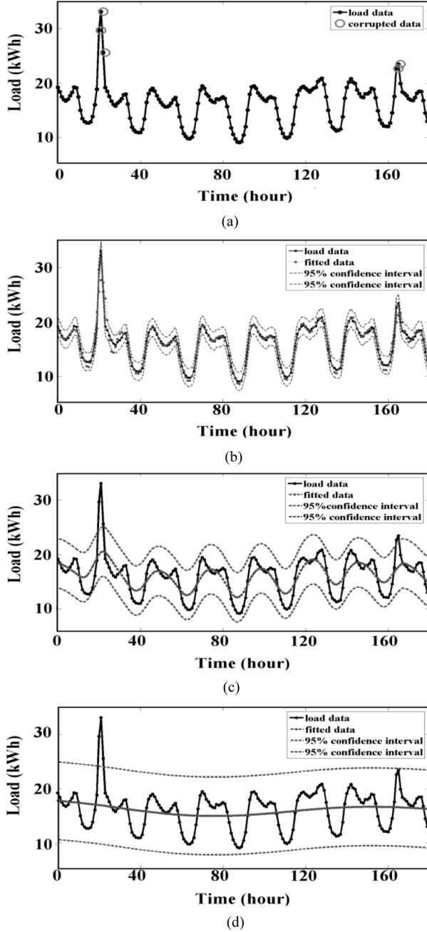
Fig. 4. Locally corrupted data detection—B-Spline smoothing. (a) Real observations with 5 corrupted data points in circles. (b) Result for smoothness Level 1. (c) Result for smoothness Level 6. (d) Result for smoothness Level 10.
