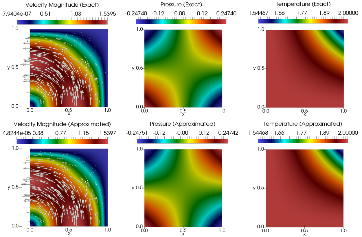
Figure 6.1: Graphical comparison of the exact solution (\mathbf{u}, p, \varphi) (upper row) and its numerical approximation (\mathbf{u}_h, p_h, \varphi_h) (lower row) for the data given in Example 1. Results calculated with 216,315 DOF and a first-order approximation (\mathbb{RT}_0 - \mathbf{P}_1 - P_0 - P_1 - P_0) .
