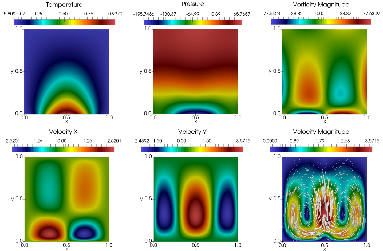
Figure 6.2: Contours of temperature, pressure and vorticity magnitude (taken as 2\gamma_{21} to coincide with the usual definition of vorticity) in the upper row, and velocity in the lower row for the data given in Example 2. Results calculated with 3,493,345 DOF and a first order approximation ( \mathbb{RT}_0 - \mathbf{P}_1 - P_0 - P_1 - P_0 ).
