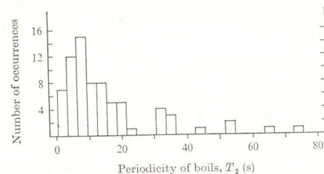
FIGURE 9. Histogram of boil periodicity over flat bed in lower Wabash River. Table 1 summarizes hydraulic data. \bar{T}_2 = 16 s, \sigma = 15 s, N = 74 .
