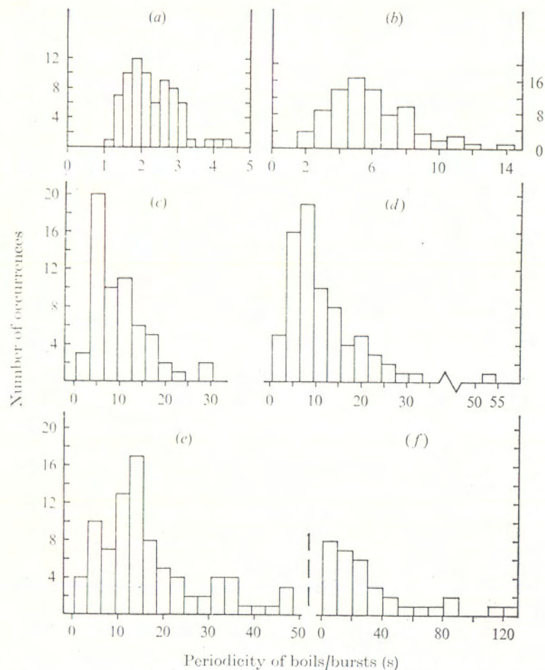
FIGURE 8. Histograms of boil periodicity T_2 in lower Wabash River [(c)–(f)] and of burst periodicity T_1 in laboratory flow of Kim et al. [(a), (b)] (1971, figures 21b and 22b). Table 1 summarizes boil measurements. (a) \bar{T}_1 = 2.3 s, \sigma = 0.71 s, N = 73 . (b) \bar{T}_1 = 6.5 s, \sigma = 3 s, N = 87 . (c) \bar{T}_2 = 9.8 s, \sigma = 6.0 s, N = 60 . (d) \bar{T}_2 = 12 s, \sigma = 8.2 s, N = 75 . (e) \bar{T}_2 = 17 s, \sigma = 11 s, N = 86 . (f) \bar{T}_2 = 35 s, \sigma = 32 s, N = 33 .
