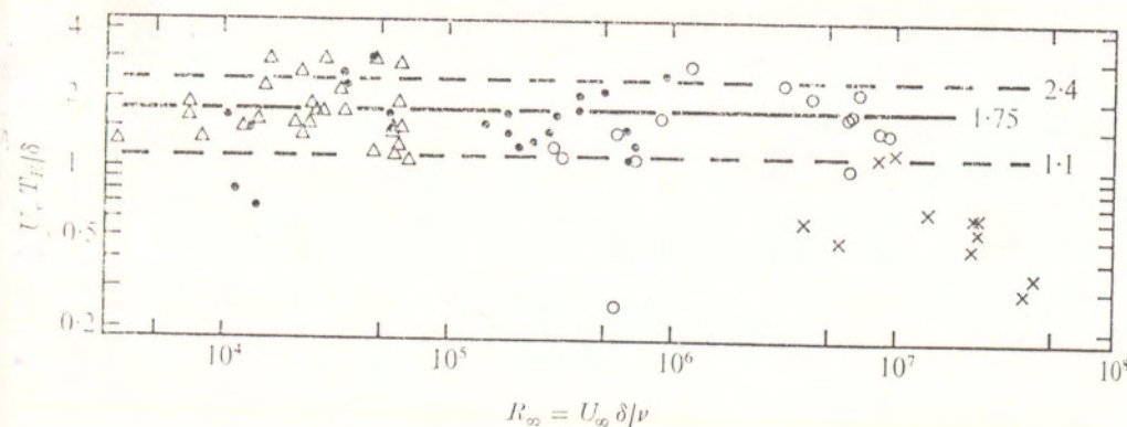
FIGURE 11. Scaling of Eulerian integral time scale with outer variables, emphasizing type of flow. \times , Mississippi River ( \delta > 6 m); \circ , canals and Missouri River ( 0.5 \text{ m} < \delta < 5 m); \bullet , flumes with moving bed material ( 0.04 \text{ m} < \delta < 0.60 m); \triangle , flumes with no movement of bed material ( 0.02 \text{ m} < \delta < 0.29 m). 1.75 is arithmetic mean of T_E^* for all data except Mississippi River values. Dashed lines define bandwidth of 2.1, which includes most of the non-Mississippi data (cf. figures 3, 7, 10). Data from tables 1, 2, 4, 6–8, 10 and 11 of McQuivey (1973).
