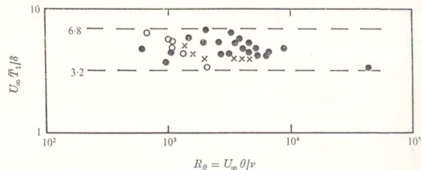
FIGURE 3. Scaling of burst periodicity with outer variables. Dashed lines define bandwidth of 2.1 which includes all data. \bullet , hot-wire air data; \times , hot-film water data; \circ , visual water data. Data sources are Rao et al. (1971, figure 9) and Blinco & Simons (1975, figure 8).
