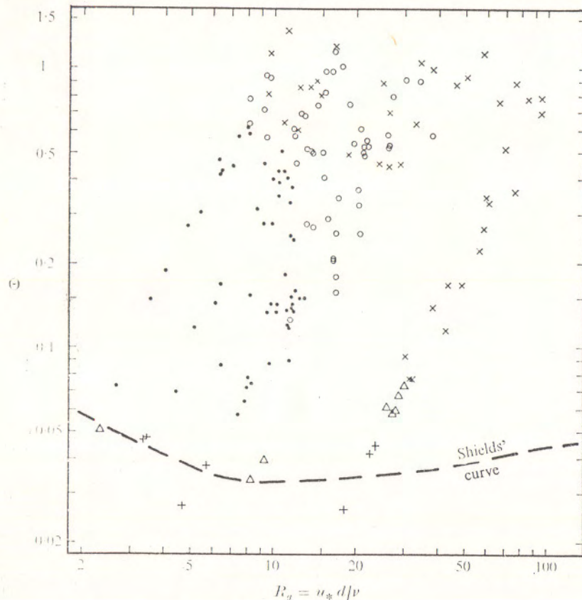
FIGURE 15. Existence fields of lower-regime bed configurations as a function of the dimensionless inner parameters \Theta , the dimensionless shear stress (Bagnold 1966), and R_g (cf. similar plot in Allen 1970, figure 2.5). x, dunes only; o, dunes superimposed by small-scale ripples; •, small-scale ripples only; Δ, lower plane bed with movement of bed material; +, plane bed with no movement of bed material. Data from Guy et al. (1966, tables 2–11). Only a representative sampling of the plane-bed data in Guy et al. is plotted. Shields' curve (heavy dashed line) is taken from Graf (1971, p. 96).
