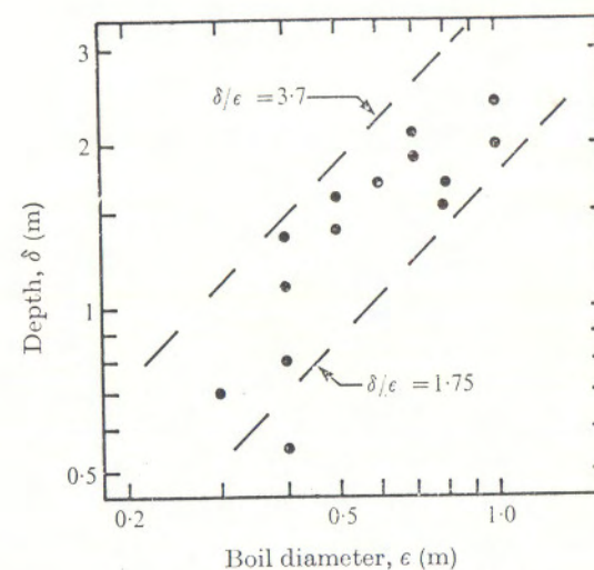
FIGURE 10. Boil diameter versus flow depth in Polomet' River, U.S.S.R. Dashed lines define bandwidth of 2:1. Data from Korchokha (1968, table 3).
