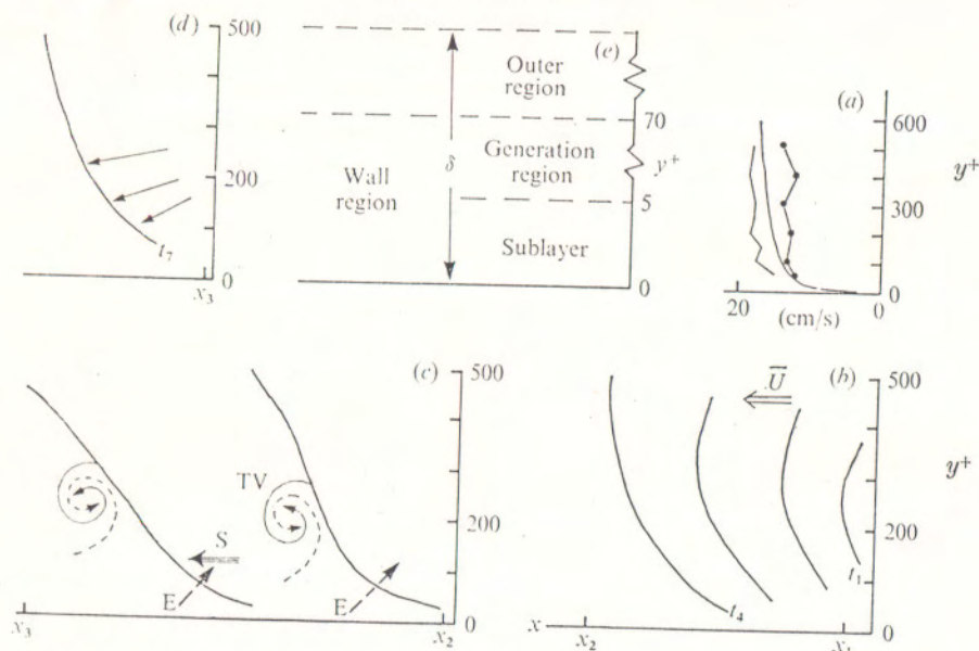
FIGURE 2. Structure of the turbulent boundary layer revealed by colloidal-particle visualization technique. (a) Typical profiles of the streamwise velocity of accelerated fluid (segmented solid line), mean flow (smooth solid line), and decelerated fluid (broken line with dots). (b)–(d) show sequential events of the burst cycle from advected view of mean flow. Each curved heavy line in (b) and (c) is an interface between accelerated fluid upstream and decelerated fluid; then (starting at time t_1 ) progressive displacement by accelerated fluid. (c) Formation of transverse vortices (TV) just ahead of advancing interface. Ejection (E) of low-speed fluid from generation region interacts with accelerated fluid and is swept downstream as a 'sweep' (S). (d) Large-scale inflow terminates burst. Curved solid line is interface at time t_7 between accelerated fluid downstream and inflow. (e) Structural regions of the turbulent boundary layer proposed by Corino & Brodkey (1969). (a)–(c) are adapted from figures 6, 4 and 8, respectively, of Nychas et al. (1973), in whose experiments \delta^+ \approx 420 .
