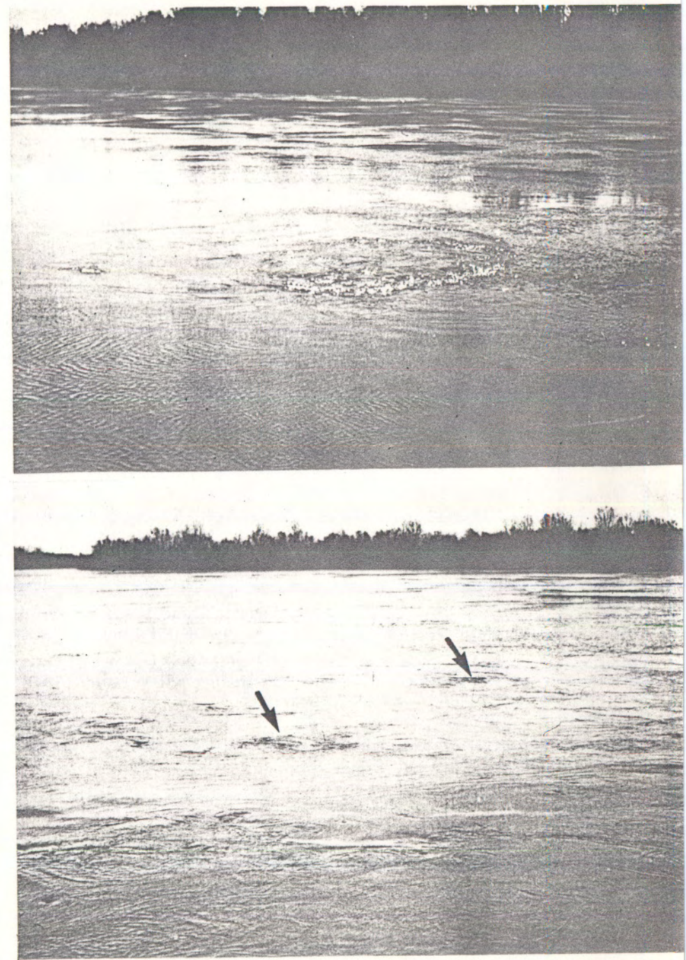
FIGURE 5. Boils in lower Wabash River. The growing boil in the centre of the upper photograph is about 1 m in diameter and outlined by white spots of reflected sunlight. The arrows in the lower photograph point to boils on the water surface which lie about 10 m downstream from the crest of a 1 m high transverse bar (water depth about 5 m). The two boils are about 1 m in diameter.
