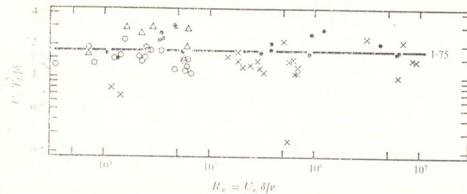
FIGURE 13. Sealing of Eulerian integral time scale with outer variables, emphasizing bed roughness. Symbols defined in table 2. The arithmetic mean of all data plotted is 1.75. The removal of three anomalously low values of T_E^* yields an arithmetic mean of 1.81, which corresponds to an apparent intermittency of 0.36. The data are the same as in figure 11, except for the removal of the Mississippi River measurements.
