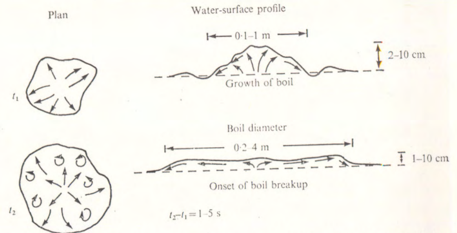
FIGURE 4. Development of typical boil in lower Wabash River. The view is that of an observer travelling with mean velocity of surface flow.
