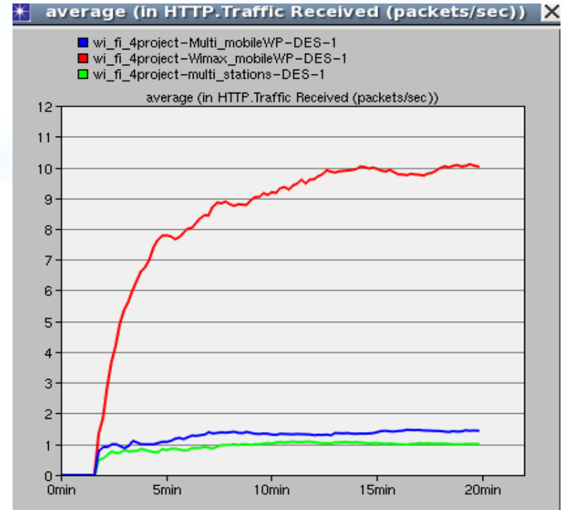
HTTP traffic received by the server
