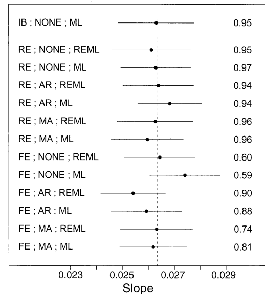
FIG. 4. Estimates of the regression coefficient (in \mu\text{m}/^\circ\text{C} ) for temperature vs. increment width from analyses of data sets simulated as described in Appendix B. Lines show 95% CI based on the empirical variance of 200 simulated slope estimates. The labels on the left give the analysis method (IB, individual based; RE, temperature as a random effect; FE, temperature as a fixed effect); the correlation structure assumed for the errors (none, first-order autoregressive, or moving average); and the estimation algorithm (maximum likelihood or restricted maximum likelihood). The numbers on the right give the proportions of 200 simulated confidence intervals that included the true mean slope.
