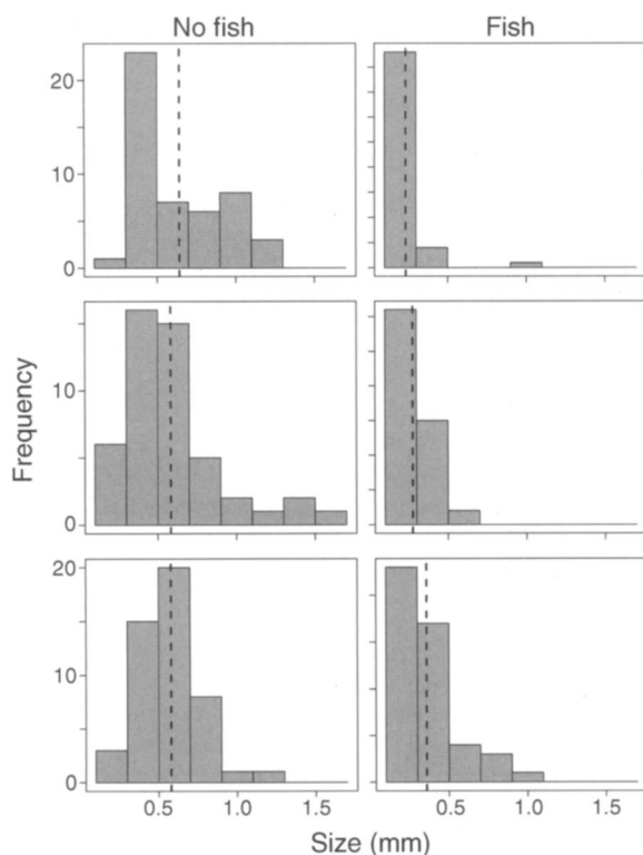
FIG. 1. Sizes of macrozooplankton in six experimental ponds at Cornell University, Ithaca, New York, USA (Murtaugh 1989): three ponds without fish (left column), three with fish (right), 48 zooplankton measurements per pond. The vertical dashed lines show the average sizes in each pond, used in the second analysis of the data.
