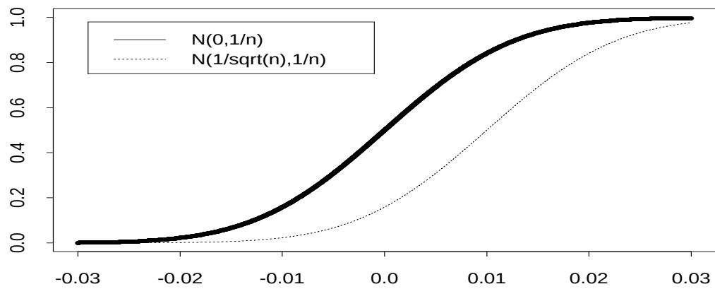
N(1/\sqrt{n}, 1/n) vs N(0, 1/n) ; n=10000
