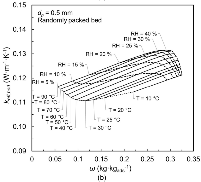
Figure 30. Effective thermal conductivity of open-system FAM-Z02 packed bed sorbers versus water uptake, including the isotherm and isobar lines for (a) SC arranged, and (b) randomly packed bed with 0.5 mm sorbent particles.
