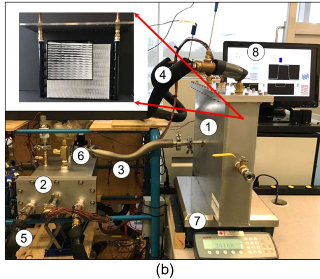
Figure 36. (a) schematic of the in-situ mass measurement testbed of an S-TES and (b) custom-built testbed, including: 1) sorber bed, 2) evaporator/condenser, 3) flexible hose, 4) HTF ports, 5) chilled/coolant water ports, 6) isolating control valve, 7) scale, and 8) LabVIEW program and data acquisition (DAQ) unit. Temperatures of the sorber bed and evaporator/condenser were maintained constant with three temperature control systems ( TCS_{hf} , TCS_{cf} and TCS_{ECU} ).
