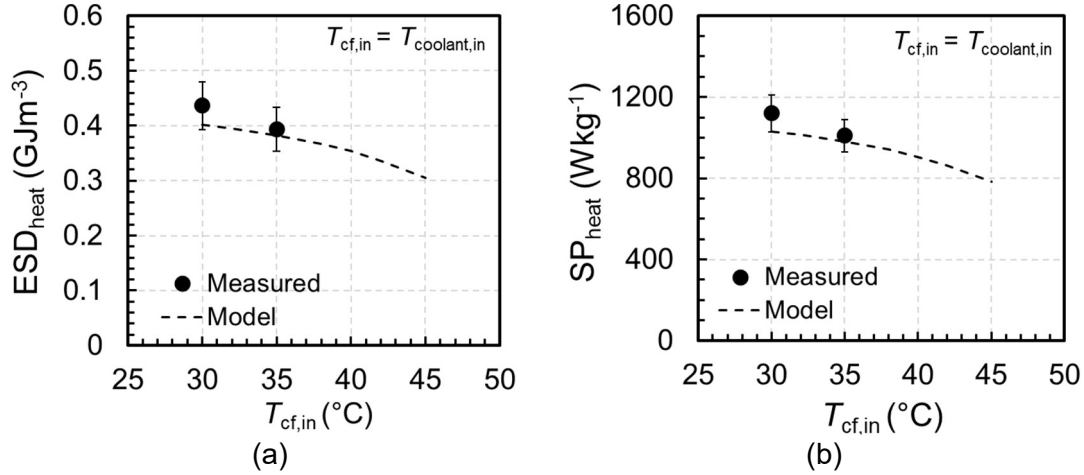
Figure 56. (a) ESD and (b) SP of heat storage 2 mm loose grain FAM-ZO2 sorber bed vs cooling fluid inlet temperature. T_{hf,in} = 90^{\circ}C , T_{chilled,in} = 15^{\circ}C , r_t = 1 , and t_{cycle} = t_{ch} + t_{dch} = 1200 s.
