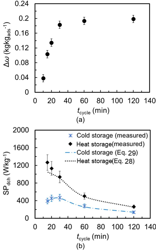
Figure 43. Effects of cycle time on the (a) net water uptake and (b) specific discharge power of a 0.3-mm coated FAM-ZO2 heat and cold sorption TES. T_{\text{des}} = 90\text{ }^{\circ}\text{C} , T_{\text{ads}} = 30\text{ }^{\circ}\text{C} and T_{\text{ECU}} = 20\text{ }^{\circ}\text{C} .
