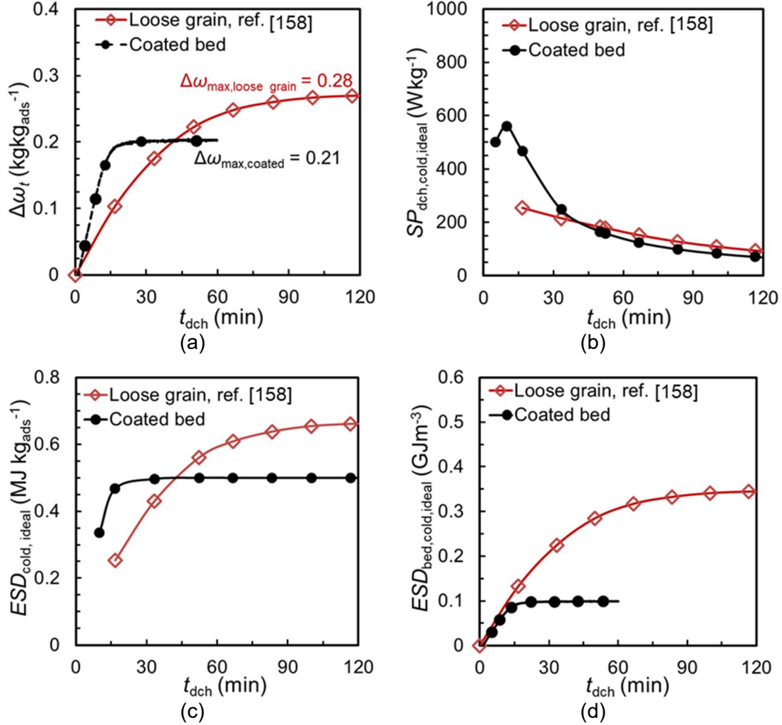
Figure 41. (a) Net water uptake, (b) specific discharge power (Eq. (18)), (c) material-based ESD (Eq. (19)), and (d) sorber bed-based ESD, obtained from ESD_{bed, cold, ideal} = (\Delta\omega h_{fg} m_s)/V_{bed\ HEX} , of 0.3-mm coated FAM-Z02 sorption TES compared to a 2-mm diameter FAM-Z02 loose grain (ref. [158]) for cold storage applications. The charging is done long enough to ensure that the S-TES is fully charged. Active volume of coated sorber bed is 3835 cm 3 ( A_{ht} = 2.8 cm 2 ) and loose grain sorber bed is 2876 cm 3 ( A_{ht} = 2.1 cm 2 ); T_{des} = 90 °C, T_{ads} = 30 °C, T_{ECU} = 20 °C, (\omega_{\infty})_{coated} = 0.20 \pm 0.01 kg kg ads -1 .
