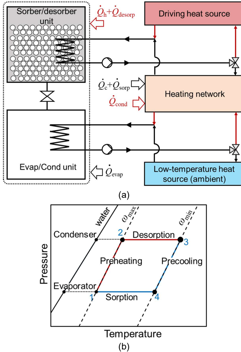
Figure 47. (a) A two-HEX S-TES concept [165], and (b) the ideal closed sorption thermodynamic cycle.
