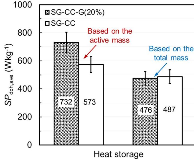
Figure 62. Effect of high-conductive additives on ESD and discharge power and (b) effects of storage duration and residual gas on ESD. Operating conditions are: T_{\text{des}}=90 \text{ }^{\circ}\text{C} , T_{\text{ads}}=T_{\text{cond}}=30 \text{ }^{\circ}\text{C} , T_{\text{evap}}=15 \text{ }^{\circ}\text{C} , and t_{\text{dch}}=35 \text{ min} .
