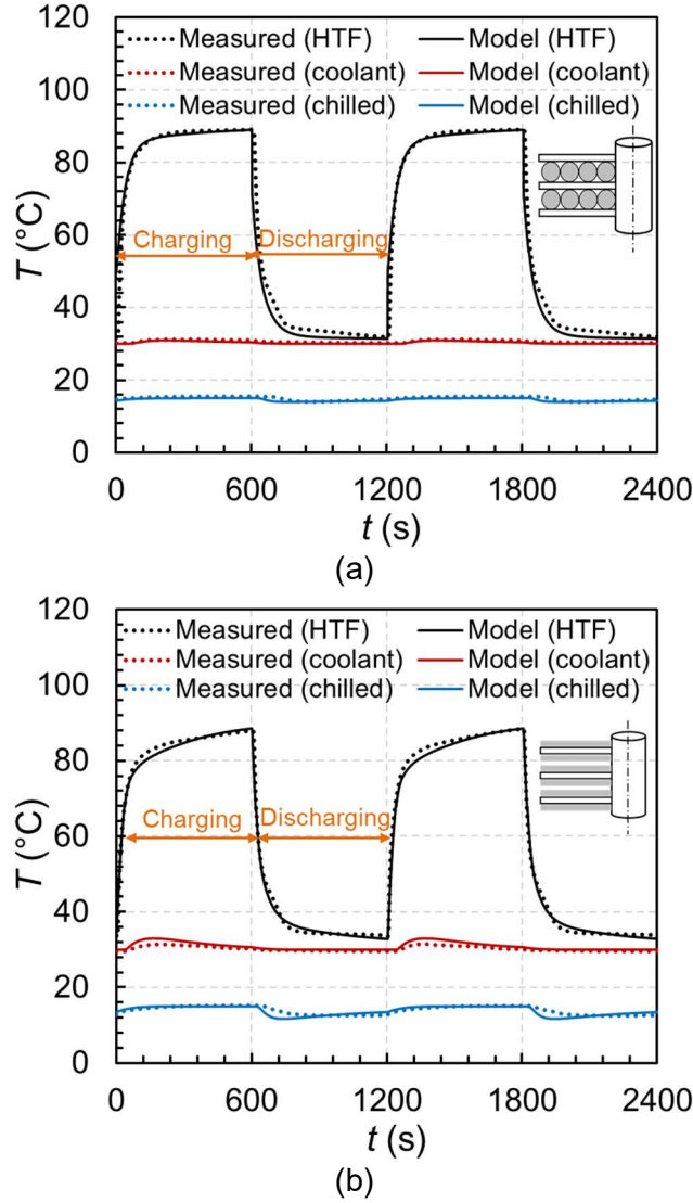
Figure 53. Temperature variation in the sorber bed, evaporator and condenser versus time, for (a) loose grain and (b) coated sorber bed — comparison between the theoretical model and experimental results. T_{hf,in} = 90\text{ }^{\circ}\text{C} , T_{cf,in} = T_{coola,in} = 30\text{ }^{\circ}\text{C} , T_{chilled,in} = 15\text{ }^{\circ}\text{C} , r_t = t_{dch}/t_{ch} = 1 , and t_{ch} + t_{dch} = 1200\text{ s} . The experimental data for loose grain and coated bed is presented in Appendix F.
