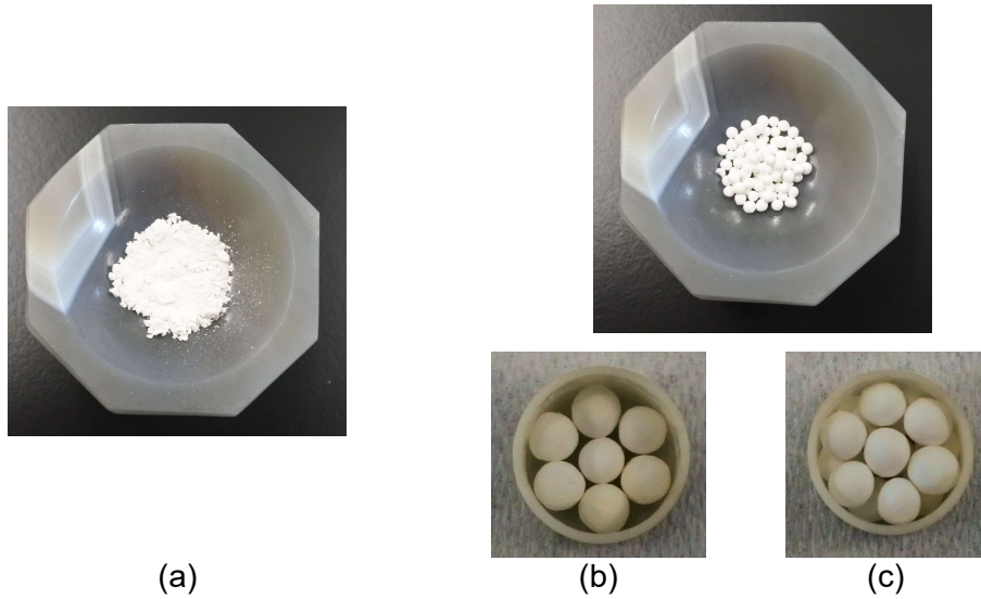
Figure 20. FAM-ZO2 samples with different configurations: (a) fine powder, (b) one layer of 2 mm particles, and (c) two layers of 2 mm particles.
