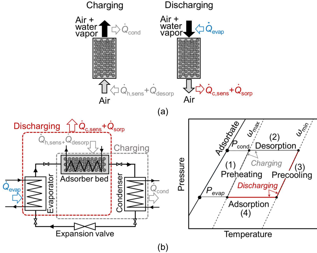
Figure 8. (a) Schematic of an open S-TES [35] and (b) schematic and the ideal thermodynamic cycle of a closed S-TES system.
