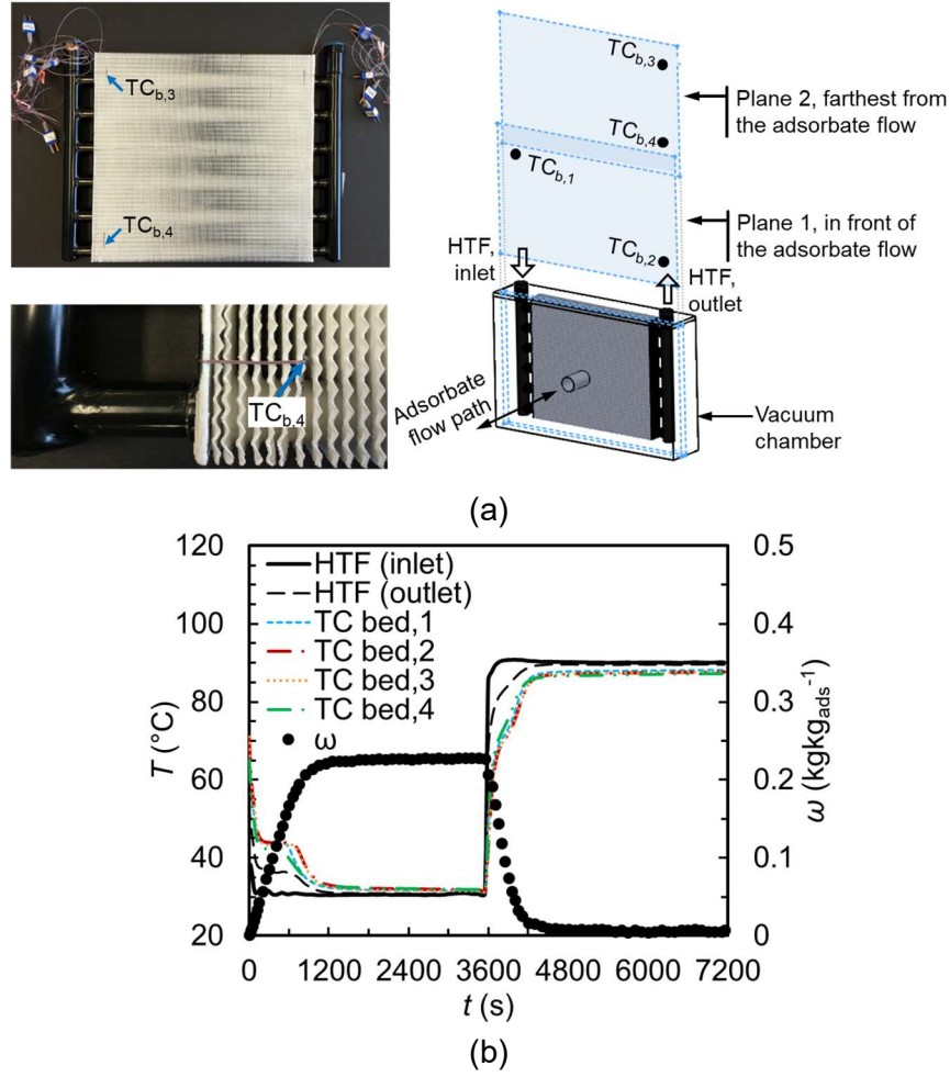
Figure 40. (a) Coated HEX with attached thermocouples on the surface of the coated sorbent, including: TC b,1 and TC b,2 in the front of the sorbate flow, and TC b,3 and TC b,4 at the plane farthest from the sorbate flow; (b) uptake and temperature variation inside the coated sorber bed vs time.
