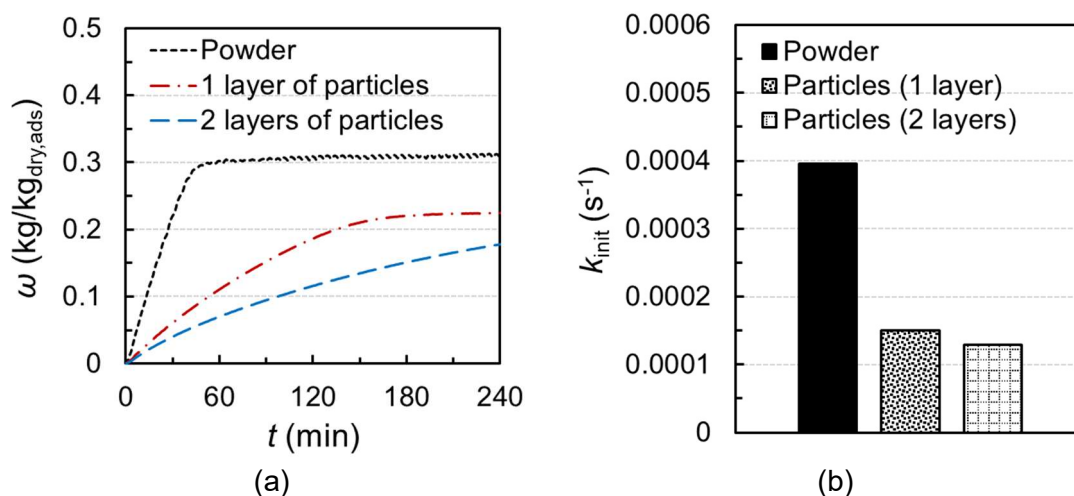
Figure 21. (a) water uptake versus time and (b) initial sorption rate of powder, 1 layer, and 2 layers of 2 mm diameter FAM-Z02 particles.
