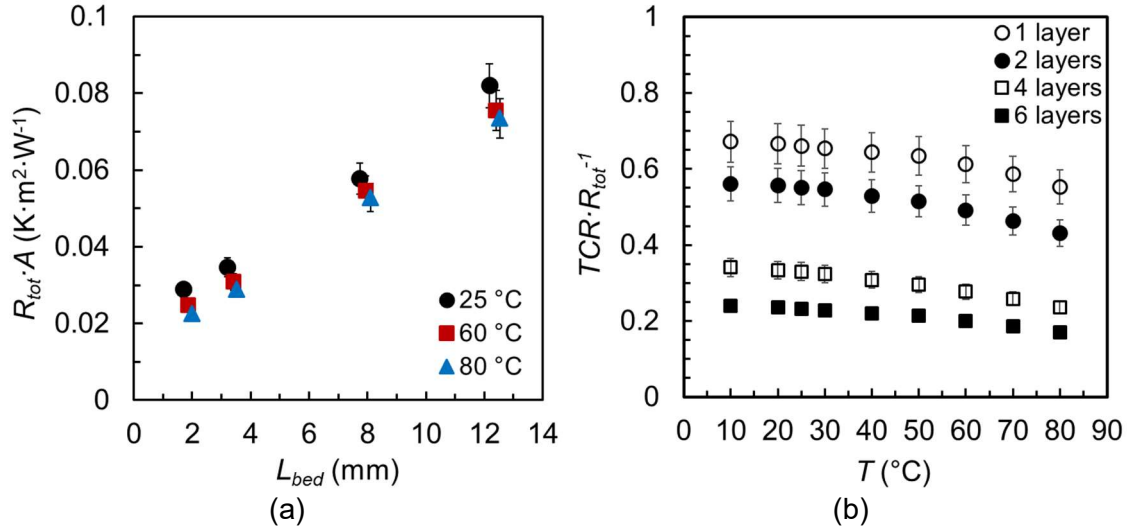
Figure 25. (a) R_{\text{tot}} A versus bed thickness of 2-mm FAM-Z02 packed beds for 1, 2, 4, and 6 layers, with water uptake of 0.30 \pm 0.02 \text{ kg kg}_{\text{ads}}^{-1} , at temperatures of 25, 60 and 80 °C under contact pressures of 0.7 kPa, and (b) measured values for relative importance of TCR to the total thermal resistance at temperatures of 10 to 80 °C.
