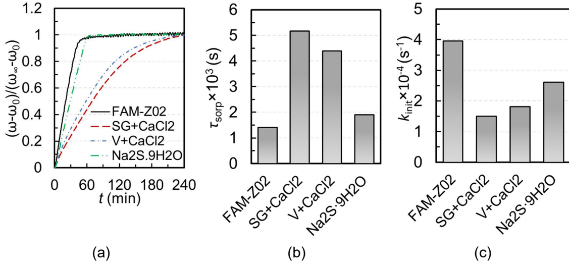
Figure 16. Sorption characteristics: (a) dimensionless water uptake (\omega/\omega_\infty) , (b) sorption characteristic time (\tau_{\text{sorp}}) , obtained from Eq. (7), (\omega - \omega_0)/(\omega_\infty - \omega_0) = 1 - \exp(-t/\tau_{\text{sorp}}) , and (c) initial sorption rate (k_{\text{init}}) for the first 15 min of sorption, obtained from equation k_{\text{init}} = d((\omega - \omega_0)/(\omega_\infty - \omega_0))/dt , for the sorbent candidates of FAM-Z02, silica gel+CaCl 2 (SG+CaCl 2 ), vermiculite+CaCl 2 (V+CaCl 2 ), and Na 2 S-H 2 O.
