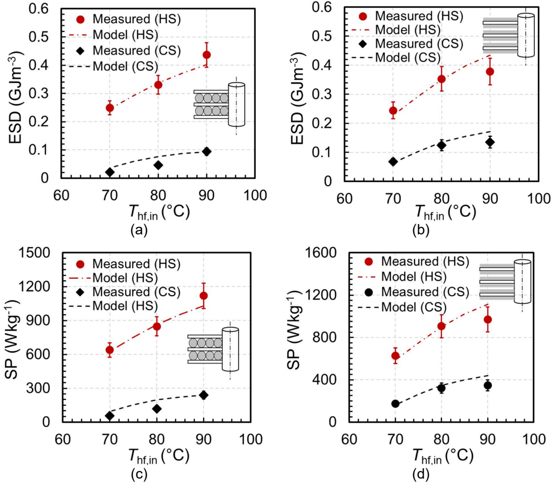
Figure 55. Material-based ESD of cold and heat storage versus heating fluid temperature for (a) 2 mm loose grain packed bed and (b) 0.2 mm coated FAM-ZO2 sorber bed and average SP for (c) 2 mm loose grain packed bed and (d) 0.2 mm coated FAM-ZO2 sorber bed. T_{cf,in} = T_{coolant,in} = 30 °C, T_{chilled,in} = 15 °C, r_t = 1 , and t_{cycle} = t_{ch} + t_{dch} = 1200 s.
