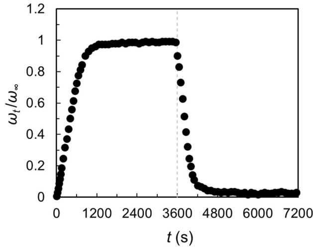
Figure 38. Dimensionless water uptake of a 0.3 mm FAM-Z02 coated sorber bed. T_{\text{des}} = 90 °C , T_{\text{ads}} = 30 °C , T_{\text{ECU}} = 20 °C, and \omega_\infty = 0.20 \pm 0.01 kgkg _{\text{ads}}^{-1} .
